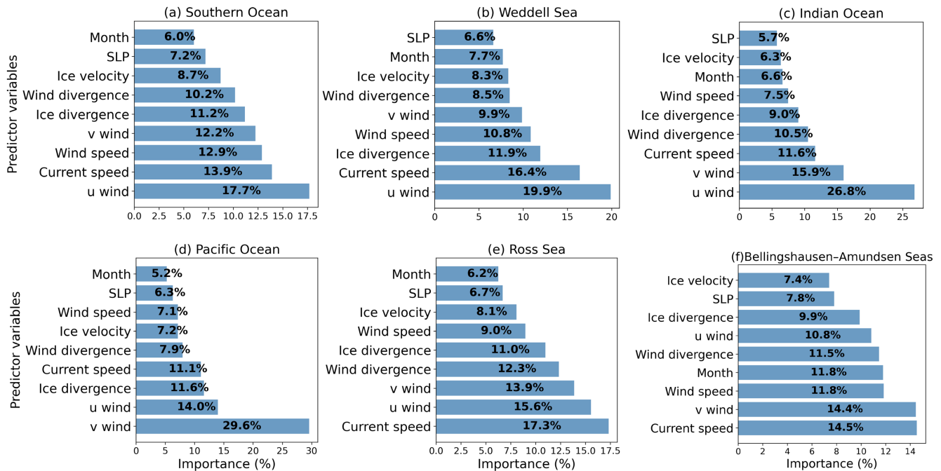
Figure 5. Relative importance of predictor variables for lead frequency based on the test subset across (a) the Southern Ocean and its regions: (b) Weddell Sea, (c) Indian Ocean, (d) Pacific Ocean, (e) Ross Sea, and (f) Bellingshausen–Amundsen Seas during April–September, 2003–2023. Values represent the percentage contribution to the model performance.
