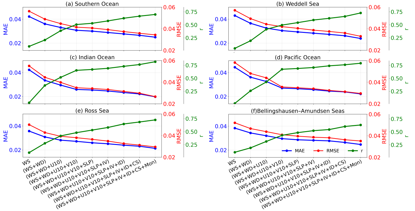
Figure 4. Incremental predictor contribution analysis showing the progressive improvement in model performance as predictor variables are sequentially added for (a) the Southern Ocean and its regions: (b) Weddell Sea, (c) Indian Ocean, (d) Pacific Ocean, (e) Ross Sea, and (f) Bellingshausen–Amundsen Seas during April–September, 2003–2023. Lines represent the MAE (blue), RMSE (red), and r (green). Predictors are added in the following sequence: wind speed (WS)→wind divergence (WD)→zonal u wind (U10)→meridional v wind (V10)→sea-level pressure (SLP)→ice velocity (IV)→ice divergence (ID)→ocean current speed (CS)→month (Mon).
