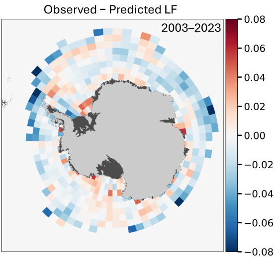
Figure A2. Spatial difference between observed and predicted mean LF (Observed - Predicted LF) for the Southern Ocean from April to September, 2003–2023, based on the test subset. Data are aggregated to 2° latitude × 5° longitude grid resolution, consistent with Fig. 1.
