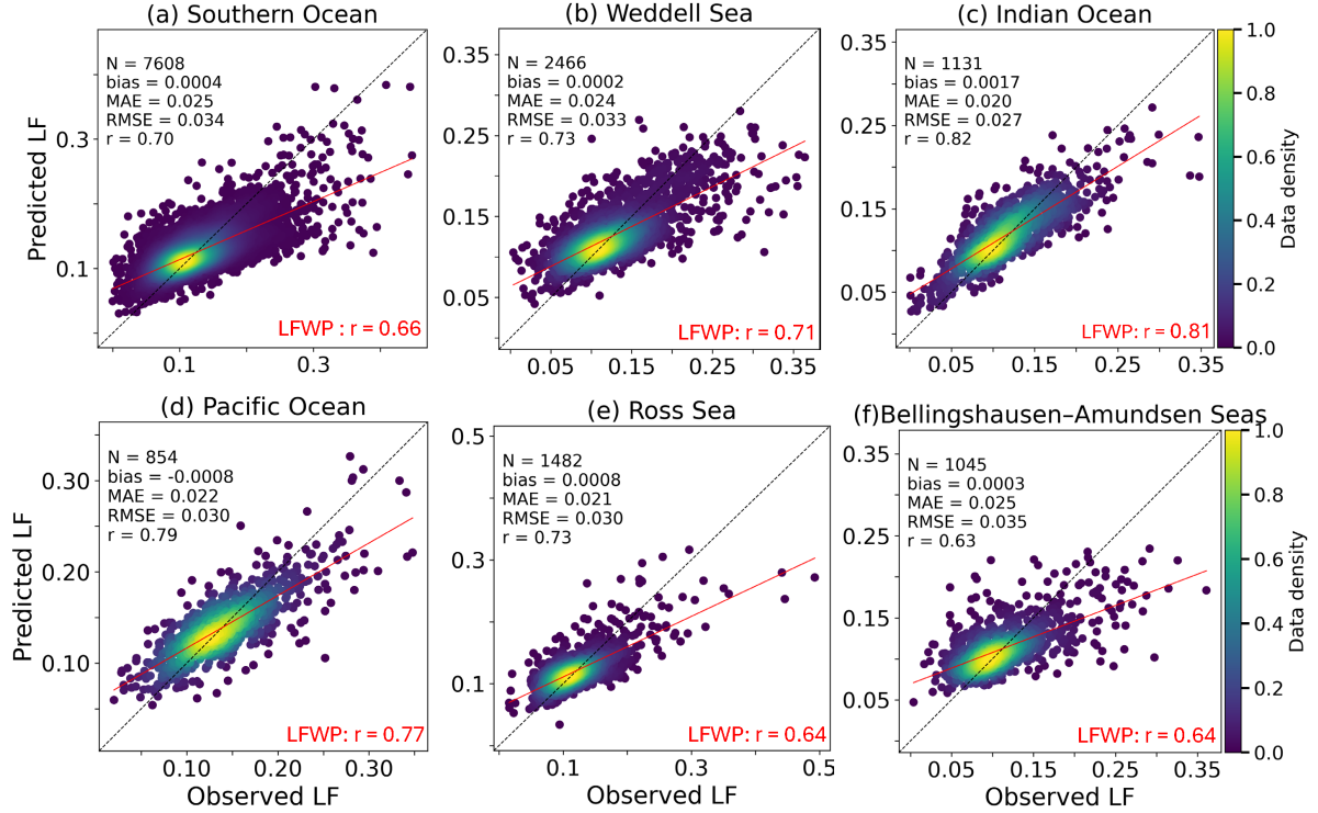
Figure 2. Model performance evaluation comparing observed versus predicted lead frequency based on the test subset for (a) the Southern Ocean and regional sectors: (b) Weddell Sea, (c) Indian Ocean, (d) Pacific Ocean, (e) Ross Sea, and (f) Bellingshausen–Amundsen Seas during April–September, 2003–2023. The black dashed line represents the 1:1 reference line, and the red line shows the linear regression fit. Color gradients indicate data point density. Performance metrics include sample size (N), bias (mean error), mean absolute error (MAE), root mean square error (RMSE), and Pearson correlation coefficient (r), all based on the model with the coastal polynyas from Lin et al. (2024) included. The red text in each panel shows the corresponding r of the model for LF without polynyas (LFWP: r), provided for comparison.
