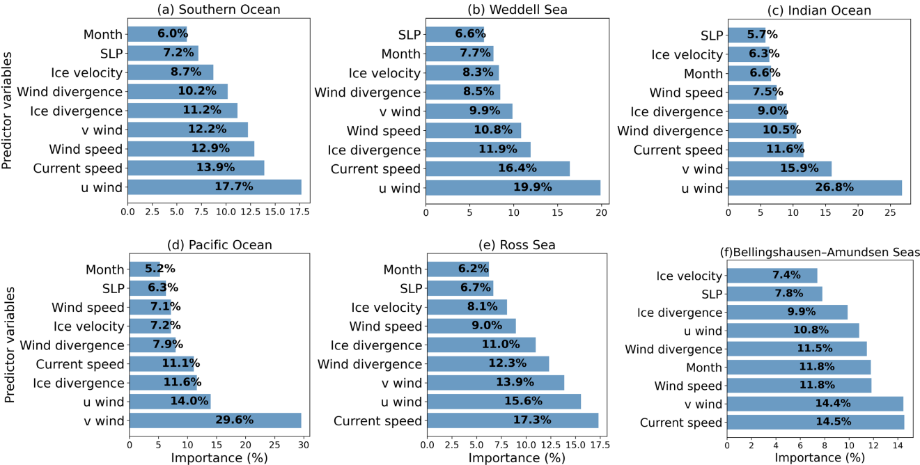
Relative importance of predictor variables for lead frequency based on the test subset for June (2003–2023) across (a) the Southern Ocean and its regions: (b) Weddell Sea, (c) Indian Ocean, (d) Pacific Ocean, (e) Ross Sea, and (f) Bellingshausen-Amundsen Seas:
