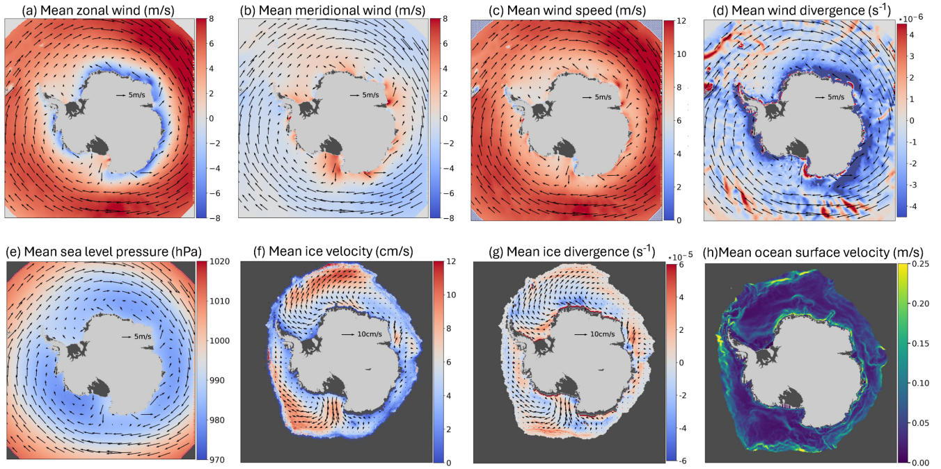
Figure A2. Mean winter (April–September, 2003–2023, excluding 2012) fields of predictor variables used for LF analysis: (a) 10 m zonal u wind, (b) 10 m meridional v wind, (c) 10 m wind speed, (d) wind divergence, (e) sea level pressure, (f) ice velocity, (g) ice divergence, and (h) ocean surface current speed. Mean wind vectors ( 5 \text{ m s}^{-1} ) and mean ice motion vectors ( 10 \text{ cm s}^{-1} ) are shown as black arrows in the respective panels. All atmospheric fields are from ERA5, ice motion from the Polar Pathfinder product, and ocean currents from ORAS5.
