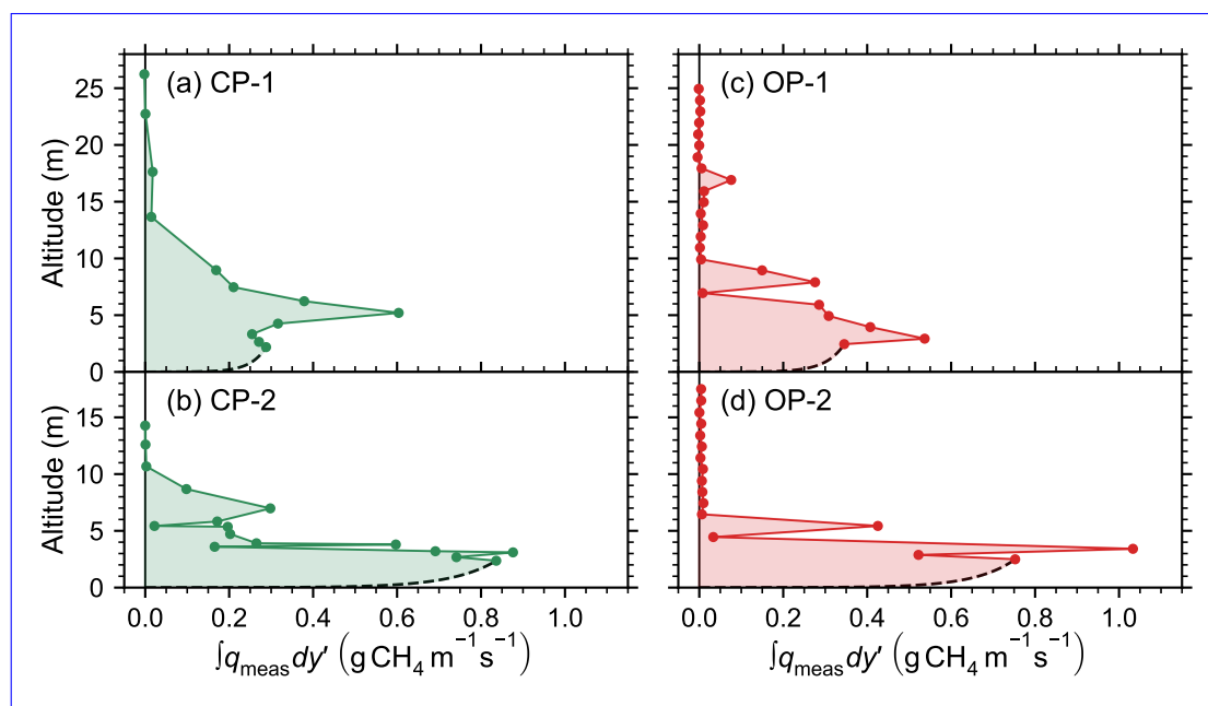
Figure 6. Calculated transect-integrated flux densities ( \int q_{\text{meas}} dy' ) for each transect used in the DMB approach. The dashed lines indicate the logarithmic fitting that was employed to extrapolate the profile from the ground to the height of the first measurement transect.
