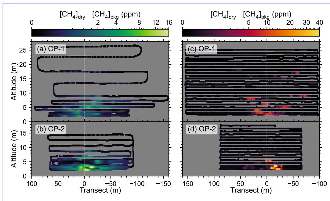
Figure 4. Measured dry methane concentrations after removing the background for the four curtain flights. (a, b) Curtains for the closed-path sensor at downwind distances of 163 m and 87 m, respectively. (c, d) Curtains for the open-path sensor at 149 m and 77 m downwind.
