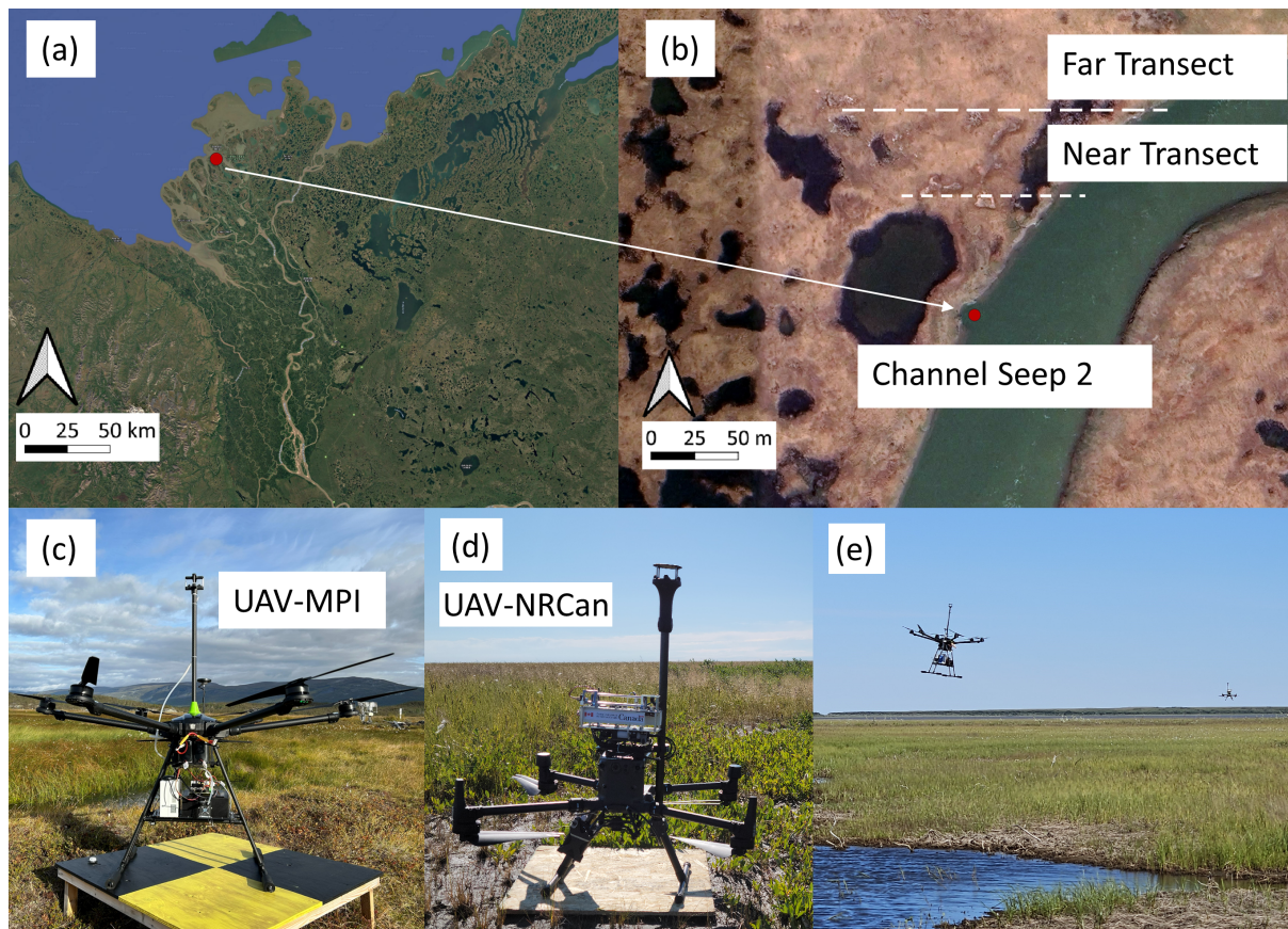
Figure 1. Study area in the outer Mackenzie River Delta, NT, Canada (a); Aerial image of the location of Channel Seep 2 ( 69.319583^{\circ} N, 135.477520^{\circ} W) indicated by red dot and approximate transects flown indicated by dashed lines (b) ((a) and (b) overlaid on satellite images from ©Google Maps); Images showing the two UAV platforms, UAV-MPI (c) and UAV-NRCan (d). Image (e) shows the two UAVs sampling downwind of \text{CH}_4 seep in the near (UAV-MPI) and far (UAV-NRCan) distances.
