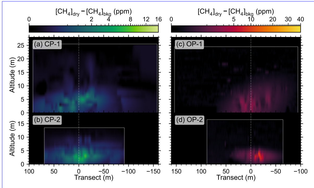
Figure 7. Kriged \text{CH}_4 enhancement fields from UAV-MPI for flights (a) CP-1 and (b) CP-2 and from UAV-NRCan for flights (c) OP-1 and (d) OP-2. The measured curtain extents are illustrated with boxes indicated by white lines, and the center of the curtain is indicated with a white vertical dashed line.
