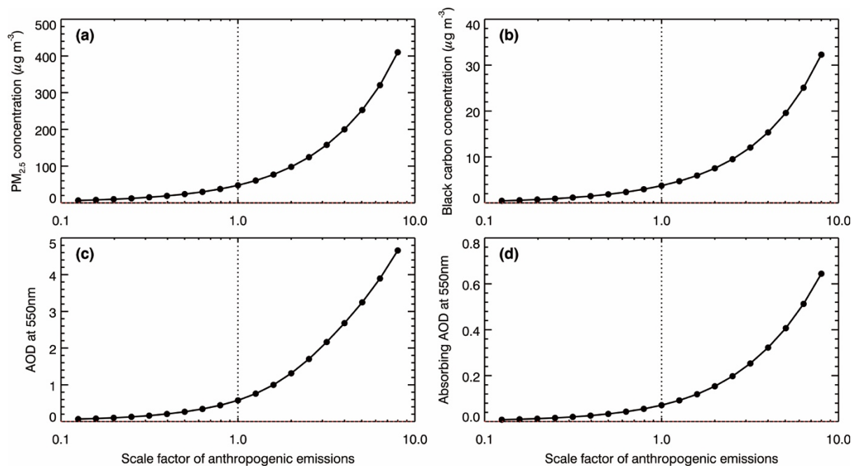
725 Figure 6: Average (a) near-surface PM 2.5 (b) black carbon mass concentration, (c) AOD at 550nm, and (d) absorbing AOD at 550 nm in GZB+GZBs from 26 to 28 January 2022, as a function of the scale factor of anthropogenic emissions.
