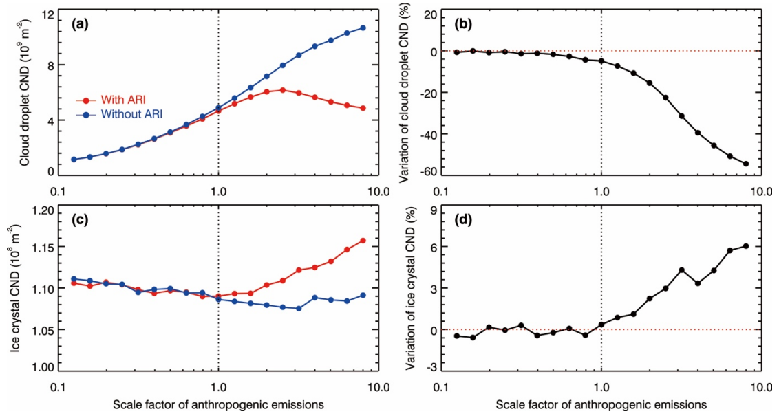
735 Figure 8: Average (a) cloud droplet CND, (b) variation of cloud droplet CND due to ARIs, (c) ice crystal CND, and (d) variation of ice crystal CND due to ARIs over GZB+GZBs from 26 to 28 January 2022, as a function of the scale factor of anthropogenic emissions.
