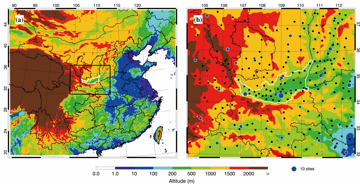
690 Figure 1: (a) WRF-Chem simulation domain with topography and (b) Guanzhong basin (GZB) and its surrounding areas (GZBs). In (b), the black dots denote the meteorological sites with rain gauge and the blue dots denote centers of cities with air pollutants observations and the size of blue circles denotes the number of ambient monitoring sites of cities. The white contour outlines the GZB and the area outside of GZB in (b) is referred to as GZBs.
