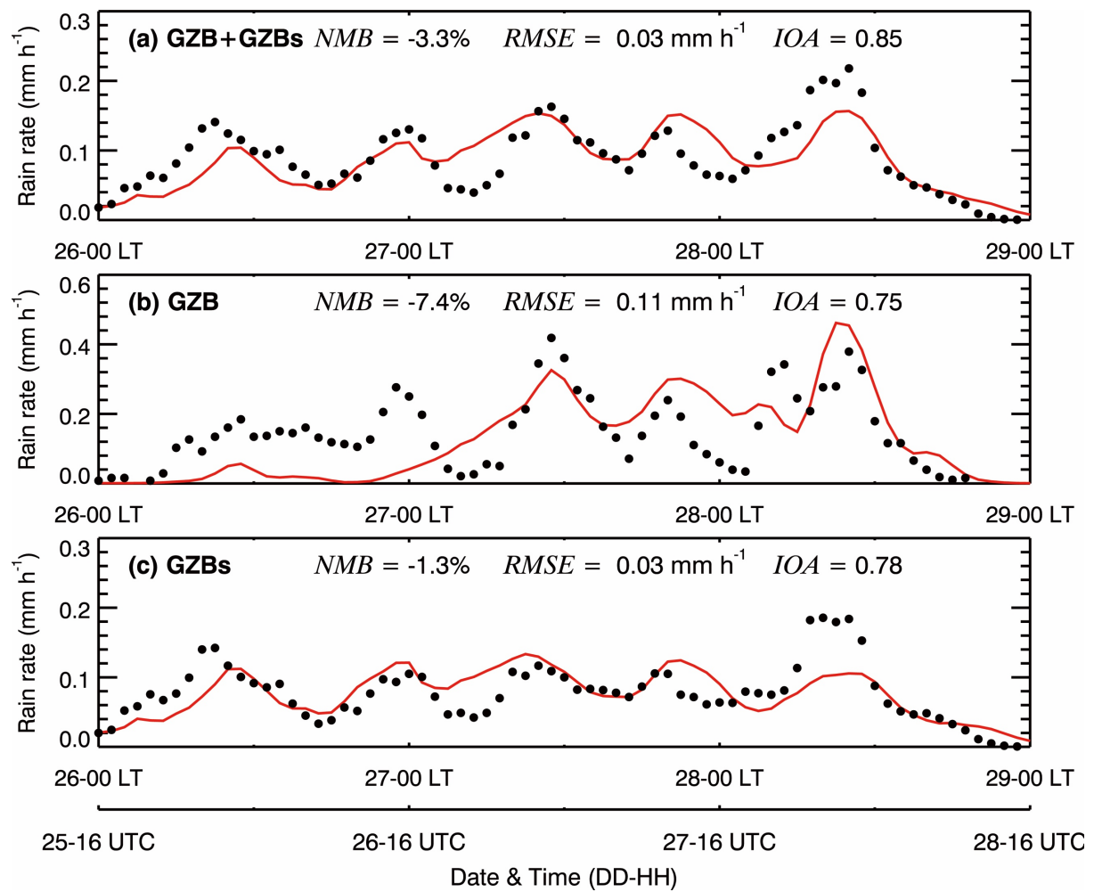
710 Figure 4: Comparison of observed (black dots) and simulated (solid red lines) diurnal profile of hourly rain rate averaged at monitoring sites in (a) GZB+GZBs, (b) GZB, and (c) GZBs from 26 to 28 January 2022.
