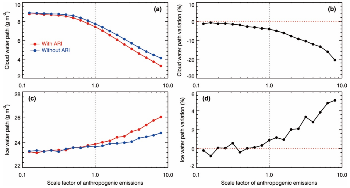
745 Figure 9: Average (a) CWP, (b) variation of CWP due to ARIs, (c) IWP, and (d) variation of IWP due to ARIs over GZB+GZBs from 26 to 28 January 2022, as a function of the scale factor of anthropogenic emissions.
