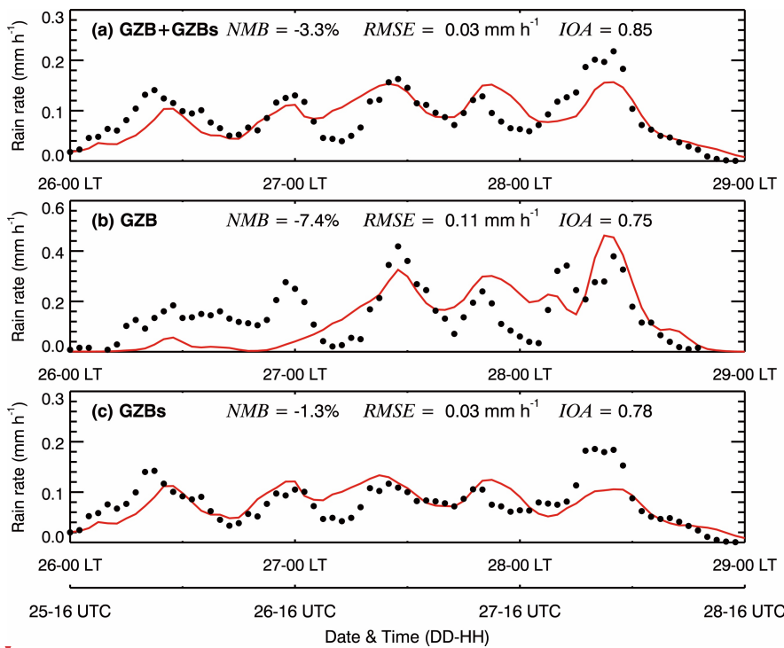
Figure 4: Comparison of observed (black dots) and simulated (solid red lines) diurnal profile of hourly rain rate averaged at monitoring sites in (a) GZB+GZBs, (b) GZB, and (c) GZBs, from 26 to 28 January 2022.
