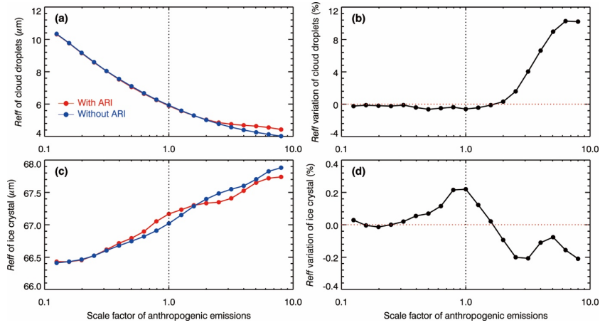
Figure 10: (a) p -mean of R_{eff,c} , (b) variation of p -mean of R_{eff,c} due to ARIs, (c) p -mean of R_{eff,i} , and (d) variation of p -mean of R_{eff,i} due to ARIs over GZB+GZBs from 26 to 28 January 2022, as a function of the scale factor of anthropogenic emissions.
