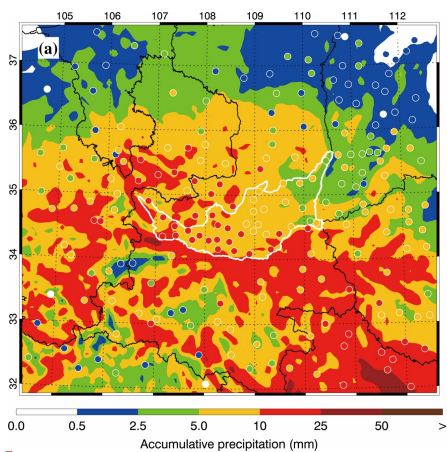
Figure 5: (a) Pattern comparisons of simulated (color counters) vs. observed (colored dots) accumulative precipitation, and (b) scatter plot of simulated and observed accumulative precipitation in GZB, GZBs, and GZB+GZBs from 26 to 28 January 2022. The white contour outlines the GZB, and the area outside of GZB in (a) is referred to as GZBs.
