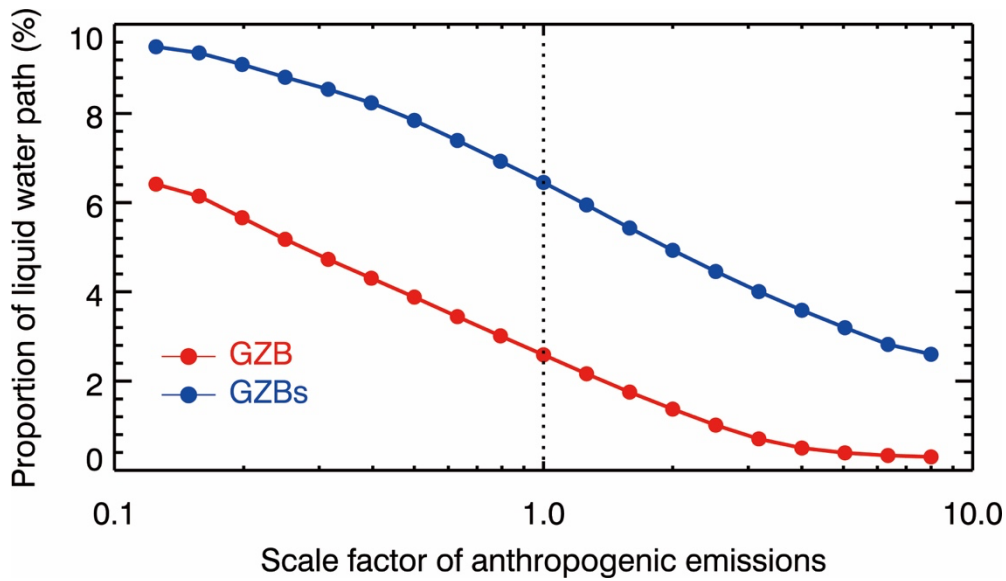
Figure S9: The proportion of liquid water paths over GZB and GZBs from 26 to 28 January 2022 in the F_BASE, as a function of the scale factor of anthropogenic emissions.
