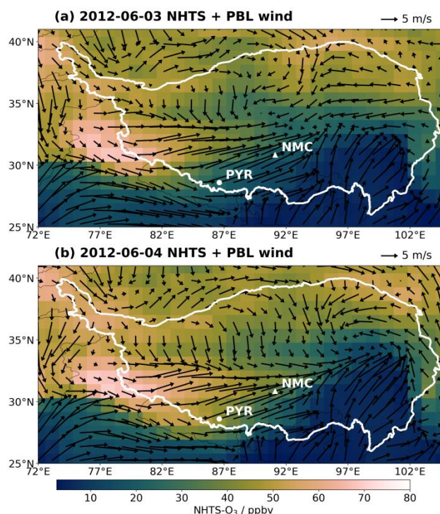
Figure 9. EMAC simulated changes in the regional distribution of surface NHTS-O 3 (color shading, units: ppbv) and the boundary layer average wind field (arrows, units: m/s) during a typical NHTS-O 3 transport event over the Tibetan Plateau: (a) corresponds to 3 June 2012, and (b) corresponds to 4 June 2012. White lines highlight the Tibetan Plateau area, and white dots mark the locations of the PYR (circle) and NMC (triangle) stations.
