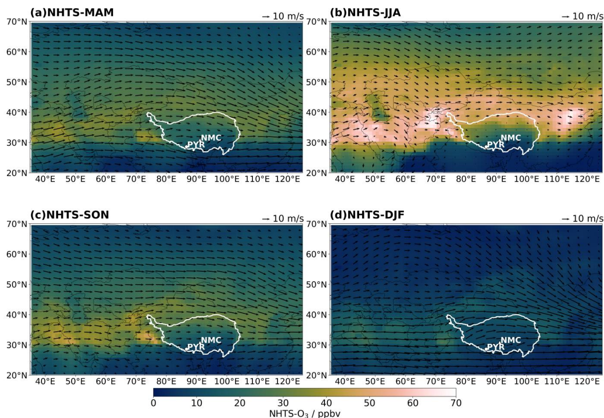
Figure 6. EMAC simulated regional distributions of surface NHTS-O 3 and 500 hPa wind field over parts of Eurasia (35°E-125°E, 20°N-70°N) in different seasons averaged over the period 2010-2012: (a) Spring, (b) Summer, (c) Autumn, (d) Winter. Color shading denotes NHTS-O 3 volume mixing ratio (units: ppbv), and black arrows represent the wind field (units: m/s). White lines highlight the Tibetan Plateau area, and white dots mark the locations of the PYR (circle) and NMC (triangle) stations.
