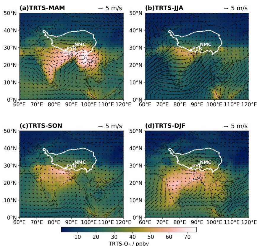
Figure 7. EMAC simulated regional distributions of surface TRTS-O 3 and boundary layer average wind field over a larger area covering the Tibetan Plateau, South Asia, and Southeast Asia in different seasons averaged over the period 2010–2012: (a) Spring, (b) Summer, (c) Autumn, (d) Winter. Color shading denotes TRTS-O 3 volume mixing ratio (units: ppbv), and black arrows represent the wind field (units: m/s). White lines highlight the Tibetan Plateau area, and white dots mark the
