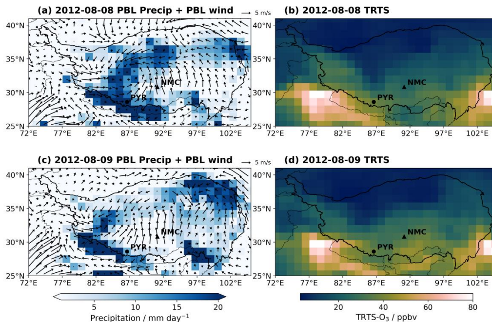
Figure 10. EMAC simulated changes in the regional distribution of surface TRTS-O 3 for a typical TRTS-O 3 transport event during the 2012 Asian summer monsoon: Row 1 (a, b) corresponds to 8 August 2012, and Row 2 (c, d) corresponds to 9 August 2012. Column 1 (a, c) shows the regional distributions of daily accumulated precipitation (color shading, units: mm day -1 ) overlaid with the boundary layer average wind field (arrows, units: m/s). Column 2 (b, d) presents the regional
