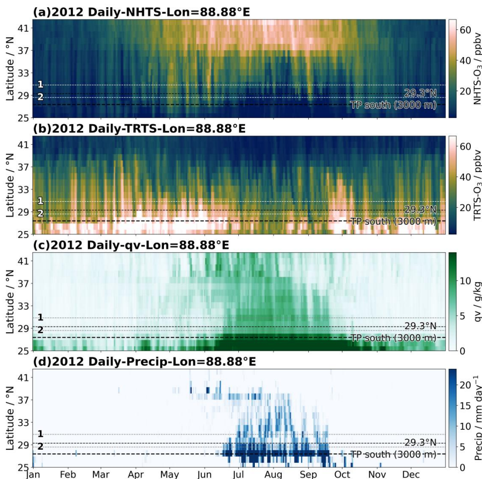
Figure 8. Time series of daily average surface (a) NHTS-O 3 mixing ratio (units: ppbv), (b) TRTS-O 3 mixing ratio (units: ppbv), (c) specific humidity (qv, units: g kg -1 ), and (d) precipitation (units: mm day -1 ) over the Tibetan Plateau at 88.88°E longitude (the midpoint of the longitudes of the two stations, NMC and PYR) in 2012, simulated by the EMAC model. The latitude 29.3°N (the boundary between the NHTS and TRTS source regions) is marked by a black dashed line, and dashed gray lines with numbered labels indicate the latitudes of the two stations (with “1” for NMC and “2” for PYR). The thick black dashed line indicates the southern boundary of the Tibetan Plateau at this longitude.
