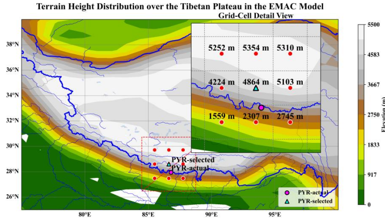
Figure B1 Spatial distribution of model terrain height over the southern Tibetan Plateau and the locations of the PYR station and candidate EMAC grid cells. The actual location of PYR is denoted by the pink dots. The selected grid cell is denoted by blue triangle.
