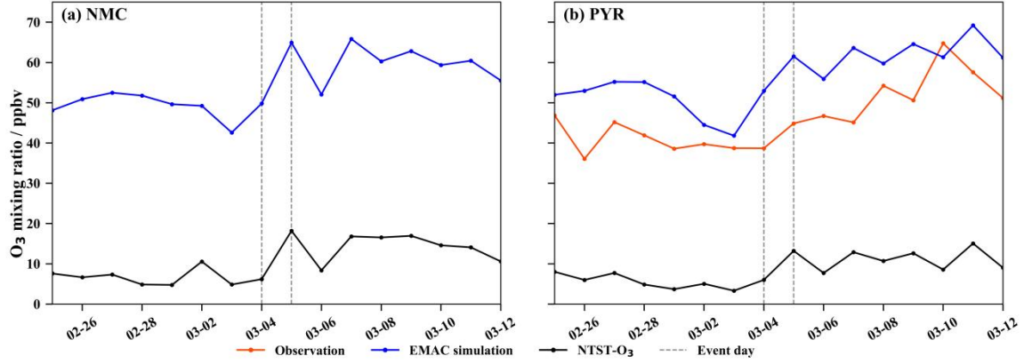
Figure A9 Time series of observed surface O_3 , modeled total surface O_3 , and surface NTST- O_3 at NMC and PYR stations during the stratospheric intrusion event of 4-5 March 2010.
