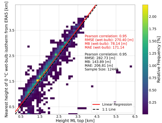
Figure B1. Scatter-density plots of the 0^\circ\text{C} wet-bulb temperature height level from ERA5 versus detected ML top heights. In addition, the Pearson correlation coefficient, RMSE, MB and MAE are given for the comparison of the ML top heights with both, the heights of the 0^\circ\text{C} wet-bulb temperature isotherm (red) and the 0^\circ\text{C} environmental temperature isotherm (black).
