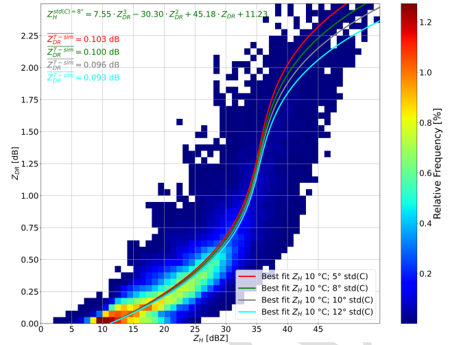
Figure 5. As in Fig. 2 but the best-fit lines of simulated Z_{DR} = f(Z_H) at a constant temperature of 10 °C with various \text{std}(\text{C}) and the mean values of Z_{DR} between 0 and 20 dBZ ( Z_{DR}^{\text{T-sim}} ) for different \text{std}(\text{C}) values.
