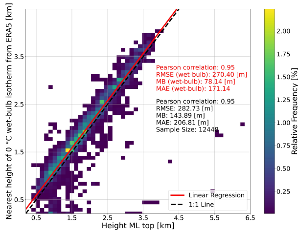
Figure B1. Scatter-density plots of the 0 °C wet-bulb temperature height level from ERA5 versus detected ML top heights. In addition, the Pearson correlation coefficient, RMSE, MB and MAE are given for the comparison of the ML top heights with both, the heights of the 0 °C wet-bulb temperature isotherm (red) and the 0 °C environmental temperature isotherm (black).
