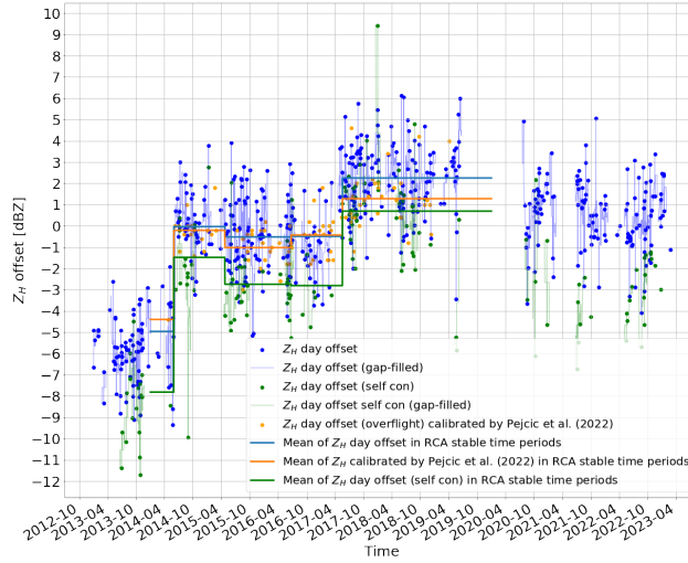
Figure 10. Daily Z_H offsets obtained from the reverse Z_H-Z_{DR} method (blue dots), the GPM overflights (orange dots; Pejic et al., 2022) and the self-consistency relations ( \Delta_{self}[Z_H] ) in the period between January 2013 to March 2023, respectively. Mean values of Z_H offsets in RCA stable time periods from Pejic et al. (2022) are given as blue, orange and green horizontal lines, respectively.
