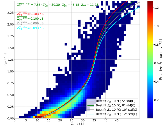
Figure 5. As in Fig. 2 but the best-fit lines of simulated Z_{DR} = f(Z_H) at a constant temperature of 10 °C with various std(C) and the mean values of Z_{DR} between 0 and 20 dBZ ( \overline{Z_{DR}^{T-sim}} ) for different std(C) values.
