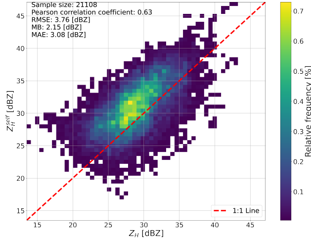
Figure 9. 2D histogram of Z_H^{self} (see Eq. 5) versus measured and offset corrected Z_H using the reverse Z_H - Z_{DR} method in the time period from 2013 to 2023. In addition to the sample size, Pearson correlation coefficient, RMSE, MB and MAE are also given.
