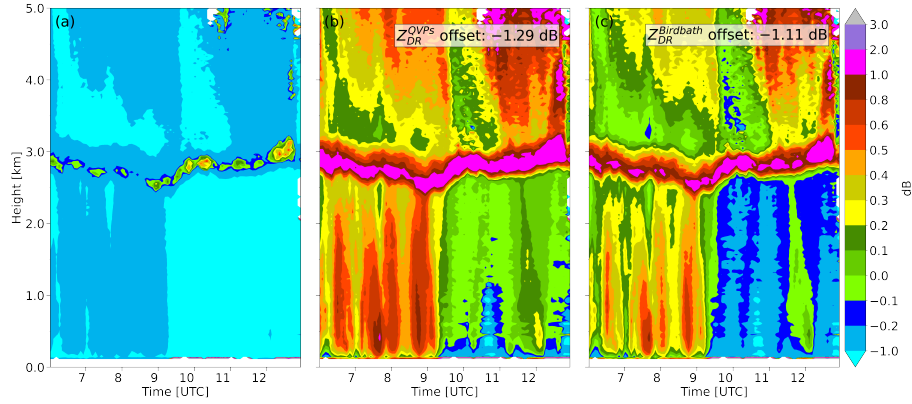
Figure 3. QVPs of Z_{DR} not offset corrected (a), offset corrected using QVP method (b) and birdbath scan method (c) for the 3 July 2013, from 06:00 UTC to 13:00 UTC.
