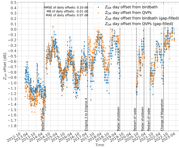
Figure 4. Daily Z_{DR} offsets calculated using for the period between January 2013 to March 2023 the QVP (orange) and birdbath scan (blue) method, respectively. The times of important changes in BoXPoI are given as vertical dashed lines with the respective caption. RMSE, MB and MAE calculated for the time period between 24 April 2014 and 3 April 2017 are shown as well.
