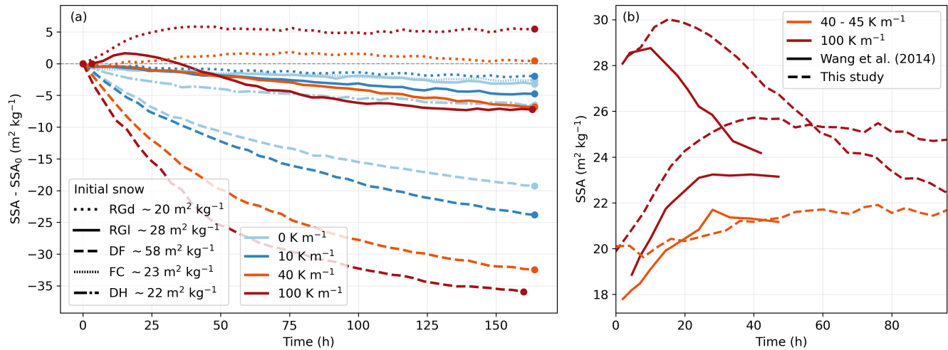
Figure 10. (a) Comparison of SSA evolution for all experiments performed at -3^{\circ}\text{C} , expressed as SSA normalized by the initial value ( \text{SSA}_0 ). The initial snow type is indicated by the line style, and its mean initial SSA is given in the legend. (b) Comparison of the SSA evolution during TGM between selected experiments from Wang and Baker (2014) and the present study using the RGI and RGd samples.
