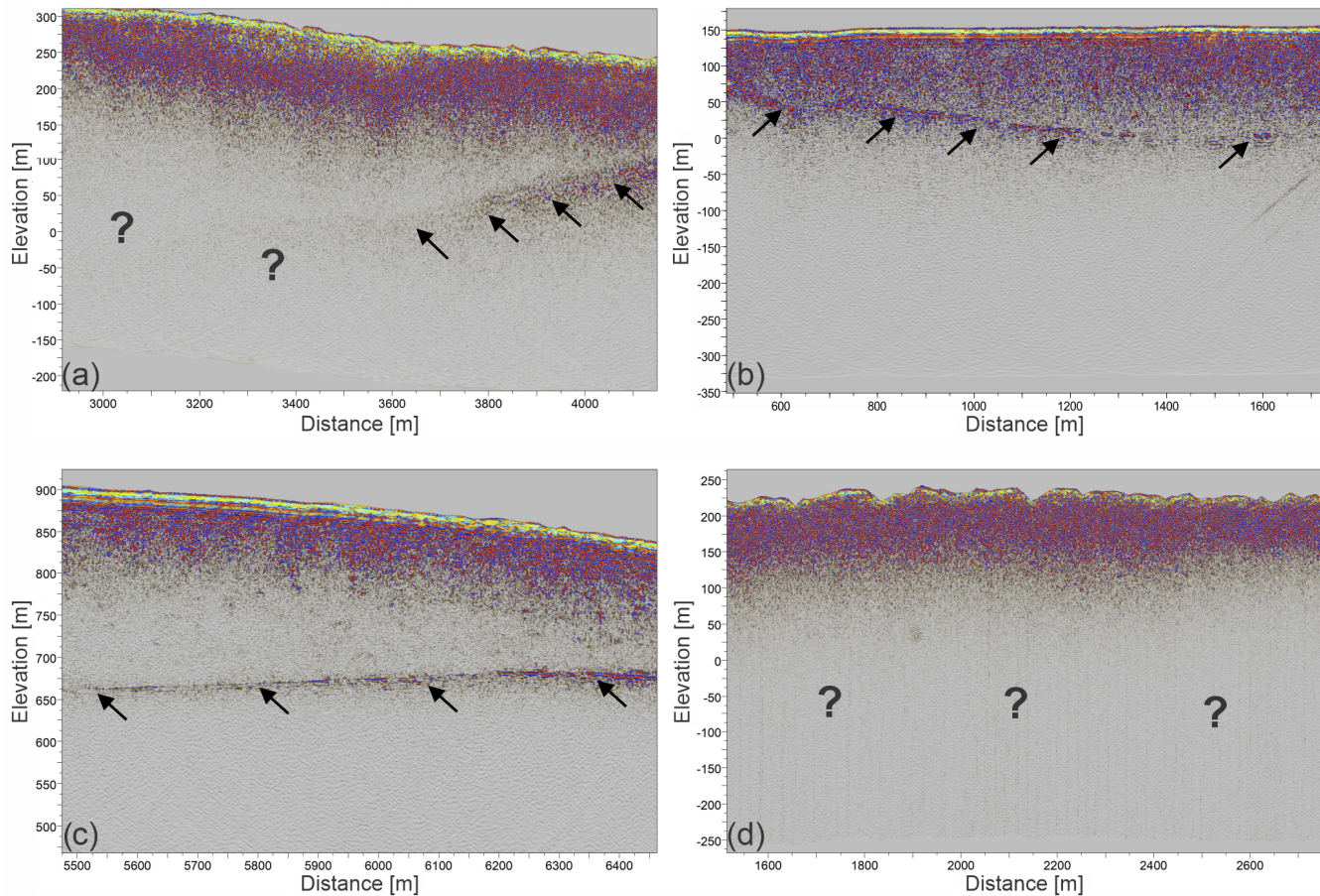
Figure 2. (a–d) Examples of 25 MHz radar sections. Black arrows mark the interpreted bed, while question marks highlight sectors with no reliable basal return. For profiles location, see Figure 1a.
