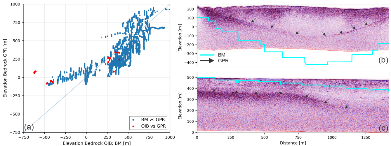
Figure 3. (a) Scatterplot of AIRETH-derived bedrock elevations compared to BM (blue) and OIB (red). The pale diagonal represents the 1:1 line. (b, c) Representative GPR profiles showing the mismatch between the bed identified in AIRETH profiles (black arrows) and BM (light blue line). For profile location, see Figure 3a.
