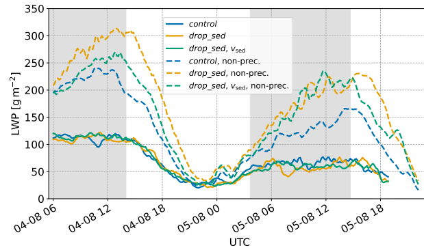
Figure A4. Leg 16A liquid water path (LWP) for the control (blue), drop_sed (orange) and halved sedimentation speed (green) experiments, including the precipitating (solid) and non-precipitating (dashed) simulations. A 1 h rolling mean was applied to all lines. Shading as in Fig. 3.
