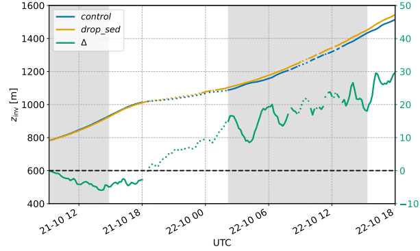
Figure A2. Leg 04A inversion height z_{\text{inv}} of the long spinup experiment, where droplet sedimentation is activated only after 15 h. Colours and shading as in Fig. 3. The dotted periods correspond to the stages where the mean cloud fraction is below 40 %.
