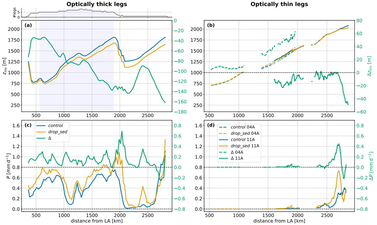
Figure 3. Binned distance plots of the inversion height z_{inv} (top panels) and the surface precipitation rate P (bottom panels), separated by category. Panels (a) and (c) represent the thick legs, whereas panels (b) and (d) represent the thin legs. The former are combined into one curve with the leg contribution depicted above the panels in grey, whereas the latter are depicted individually using dashed (solid) lines for Leg 04A (Leg 11A). The left y-axis corresponds to the absolute magnitude of both control (blue) and drop_sed (orange), while the right y-axis corresponds to the difference \Delta (green). The light blue shading indicates the core region, where at least five legs are contributing. In all panels save for (b), a rolling mean of roughly 75 km was applied.
