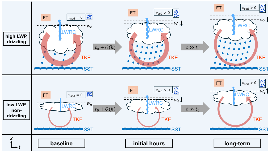
Figure 11. Schematic to illustrate the impact of droplet sedimentation on the two different idealised cloud categories ( top : optically thick and precipitating, bottom : optically thin and non-precipitating). Both show a similar initial effect regarding entrainment, but evolve structurally different afterwards. The first stage is the baseline state at time t_0 before sedimentation is activated (indicated by v_{sed} ). The middle stage is the state in the initial hours and the last stage is the state after a longer period of time. The cloud thickness is a rough measure of the liquid water path (LWP), the light blue arrows indicate longwave radiative cooling (LWRC), while the red arrows indicate turbulent circulations (turbulent kinetic energy, TKE). The ocean surface is illustrated by blue waves (sea surface temperature, SST). Dashed lines represent the inversion height z_{inv} under the dry free troposphere (FT), where entrainment occurs (marked by w_e ), with the control inversion in grey for comparison, while the arrow thickness represents the strength of the respective quantity. Note that the light blue arrows are intentionally placed in the middle (bottom) of the cloud, if radiative cooling is saturated (unsaturated).
