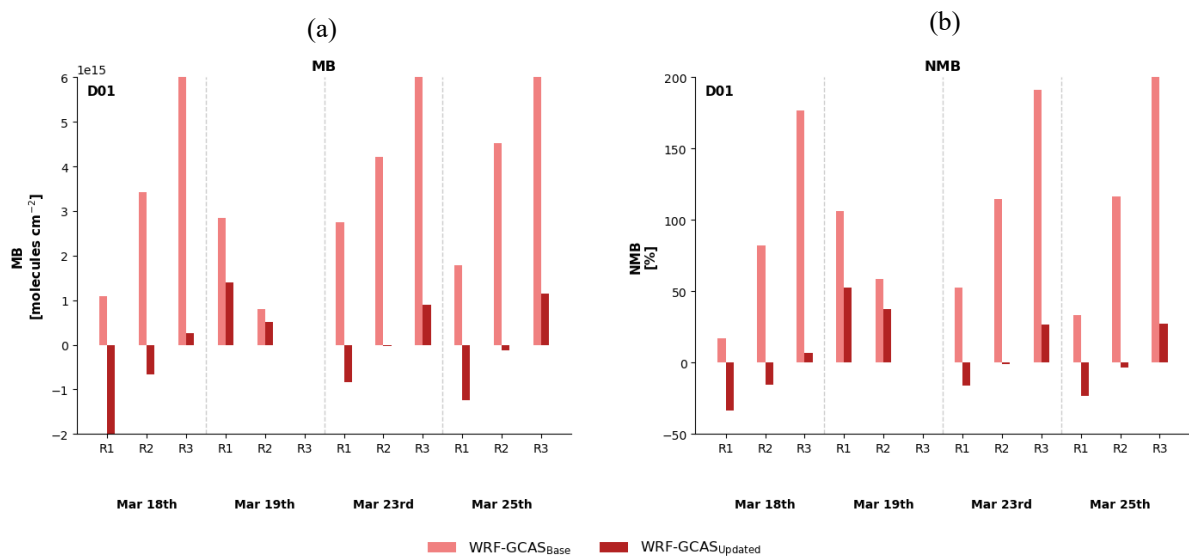
336 Figure S1819. (a) Mean bias (MB) and (b) normalized mean bias (NMB) comparing WRF-GCAS Base D01 (light red) and 337 WRF-GCAS Updated D01 (red) against GCAS observations for each raster period and ASIA-AQ flight day. Bias reductions in 338 WRF-GCAS Updated D01 increase throughout the day, indicating improved representation of the daytime NO 2 evolution relative 339 to the base simulation.
