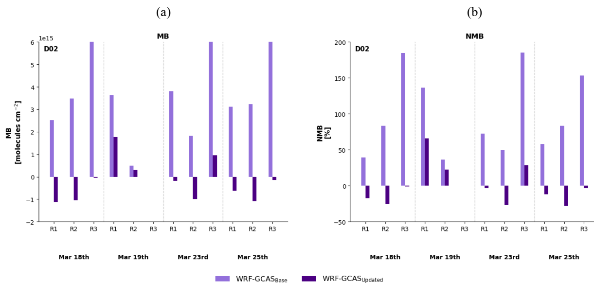
319 Figure S1748. (a) Mean bias (MB) and (b) normalized mean bias (NMB) comparing WRF-GCAS Base D02 (light purple) and 320 WRF-GCAS Updated D02 (dark purple) against GCAS observations for each raster period and ASIA-AQ flight day. Bias 321 reductions in WRF-GCAS Updated D02 increase throughout the day, indicating improved representation of the daytime NO 2 322 evolution relative to the base simulation.
