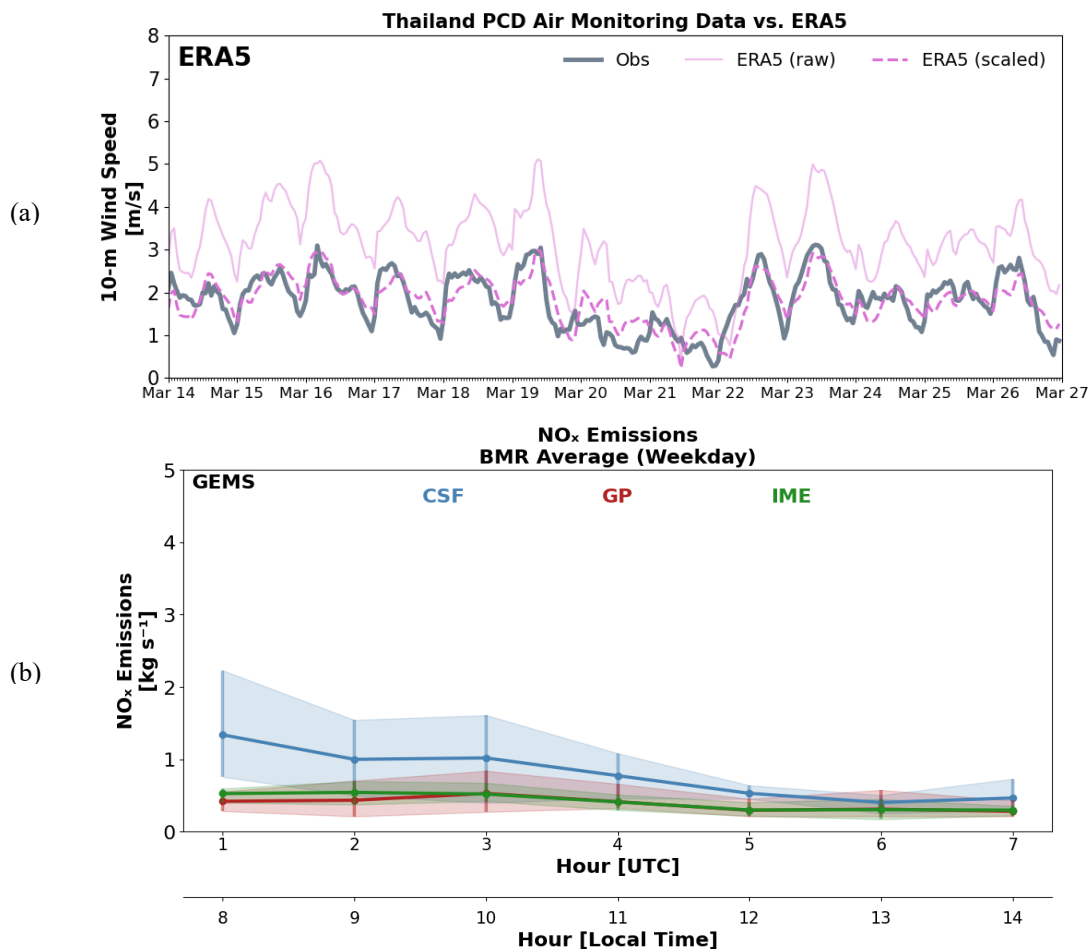
139 Figure S54. (a) ERA5 (solid pink) and Thailand Pollution Control Department (PCD) ground-monitor network (grey) wind 140 speed ( \text{m s}^{-1} ) during the ASIA-AQ deployment period (14–27 March 2024). ERA5 wind speeds scaled by a factor of 0.6 are 141 shown as dashed pink lines. (b) GEMS-derived daytime NO x emissions ( \text{kg s}^{-1} ) estimated using the cross-sectional flux (blue), 142 Gaussian plume inversion (red), and integrated mass enhancement (green) methods. Emissions represent averages across 143 daytime hours and weekdays during the ASIA-AQ deployment. As a sensitivity test, ERA5 wind speeds were scaled by a 144 factor of 0.6 prior to inversion to assess wind speed uncertainty. Reduced wind speeds lead to lower inferred emissions ( \approx 40\% ), 145 consistent with enhanced NO 2 accumulation under weaker transport and a reduced emission flux required to reproduce the 146 observed columns. These adjusted emissions fall below those inferred from other observational constraints, suggesting that 147 further wind speed reductions may not be appropriate for representing PBL-averaged transport in the BMR.
