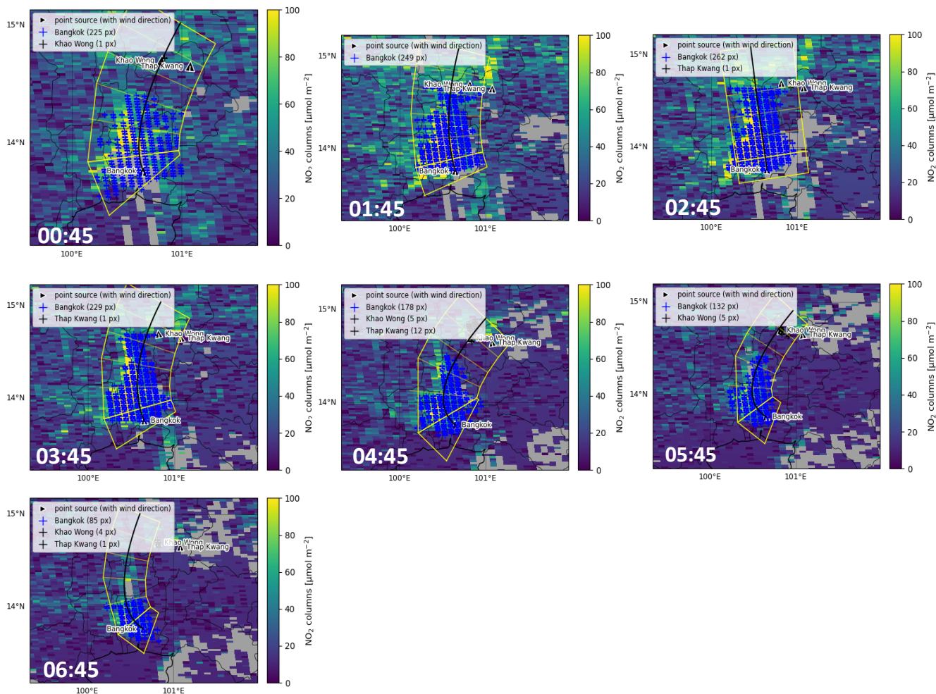
107 108 Figure S32. Example of the cross-sectional flux approach applied on 15 March 2024 using GEMS daytime measurements 109 (00:45:00–06:45:00 UTC; 07:45:00–13:45:00 LT), generated with the ddeq Python package (Kuhlmann et al., 2024). Detected 110 satellite pixels associated with the Bangkok urban plume are marked with blue ticks. A vector originating from Bangkok 111 indicates the plume direction based on ERA5 wind fields at the source location. Khao Wong and Thap Kwang districts in 112 Saraburi Province represent point sources distinct from the Bangkok urban plume, influenced by limestone quarry operations 113 and heavy-truck transport (Makkhao and Prueksasit, 2023).
