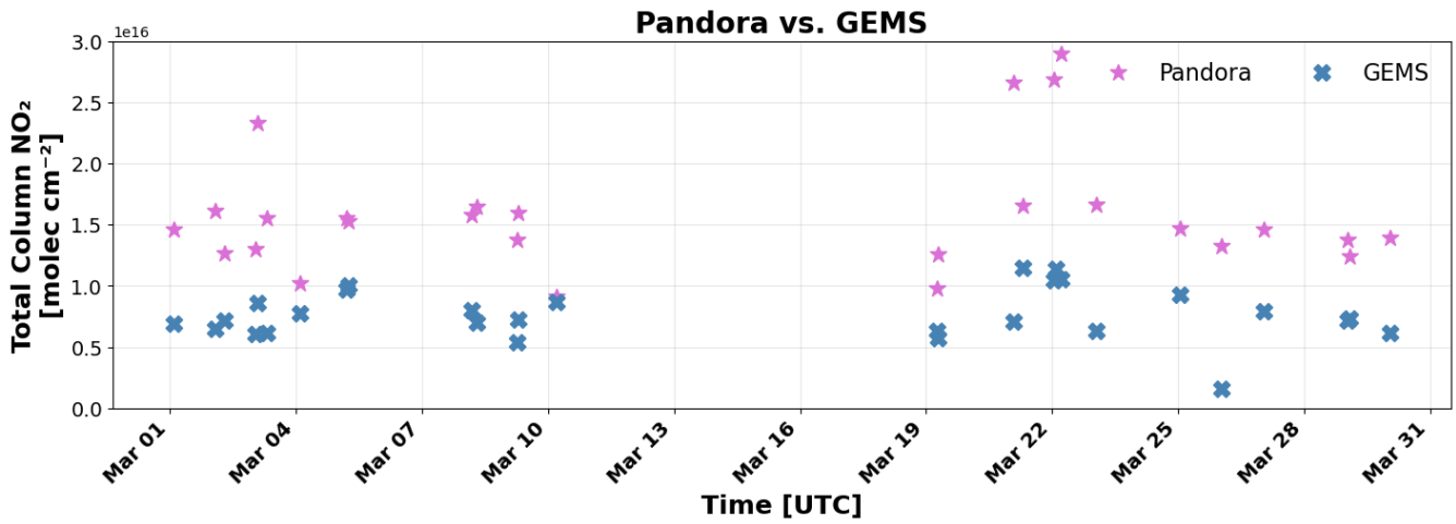
Figure S15. (a) Comparison of Pandora (pink) and GEMS (blue) total column NO 2 for high-quality observations during the March 2024. The ASIA-AQ deployment and model simulation period is representative of 14 – 27 March 2024 ASIA-AQ deployment period. GEMS reproduces the temporal variability observed by Pandora (CORR = 0.7) but systematically underestimates column magnitudes (mean bias \approx -9.2 \times 10^{15} molecules cm -2 ; mean ratio \approx 0.6 ), with the largest discrepancies occurring during the stagnation event on 21 March 2024. GEMS is generally a factor of two lower than Pandora during this period. (b) Sensitivity of CSF-derived NO x emissions to GEMS NO 2 bias correction over the BMR. The solid line shows the nominal inversion, while the solid line represents emissions derived after scaling GEMS NO 2 columns by a factor of 1.67.
