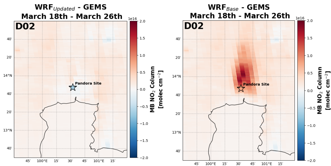
Figure S1314. Spatial distribution of mean NO 2 column bias over the BMR averaged over 18–26 March 2024. Background shading represents WRF–GEMS bias, with the Pandora site location and corresponding model bias indicated. Results are shown for (a) WRF Updated and (b) WRF Base simulations.
