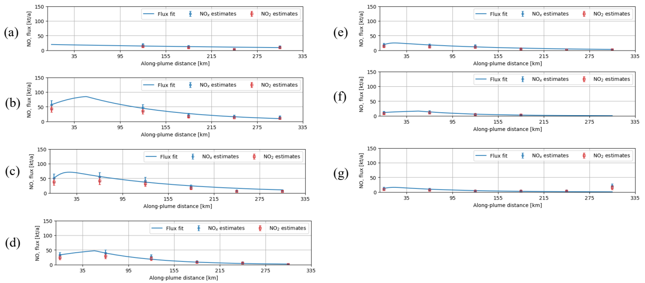
120 Figure S43. Examples of cross-sectional flux fits on 17 March 2024 for (a) 00:45:00 UTC (07:45:00 LT), (b) 01:45:00 UTC 121 (08:45:00 LT), (c) 02:45:00 UTC (09:45:00 LT), (d) 03:45:00 UTC (10:45:00 LT), (e) 04:45:00 UTC (11:45:00 LT), (f) 122 05:45:00 UTC (12:45:00 LT), and (g) 06:45:00 UTC (13:45:00 LT), generated with the ddeg Python package (Kuhlmann et 123 al., 2024). Derived NO x fluxes vary throughout the daytime, with peak values in the morning hours and decreasing toward the 124 afternoon, consistent with the daytime pattern of vehicular traffic emissions in the Bangkok Metropolitan Region (BMR).
