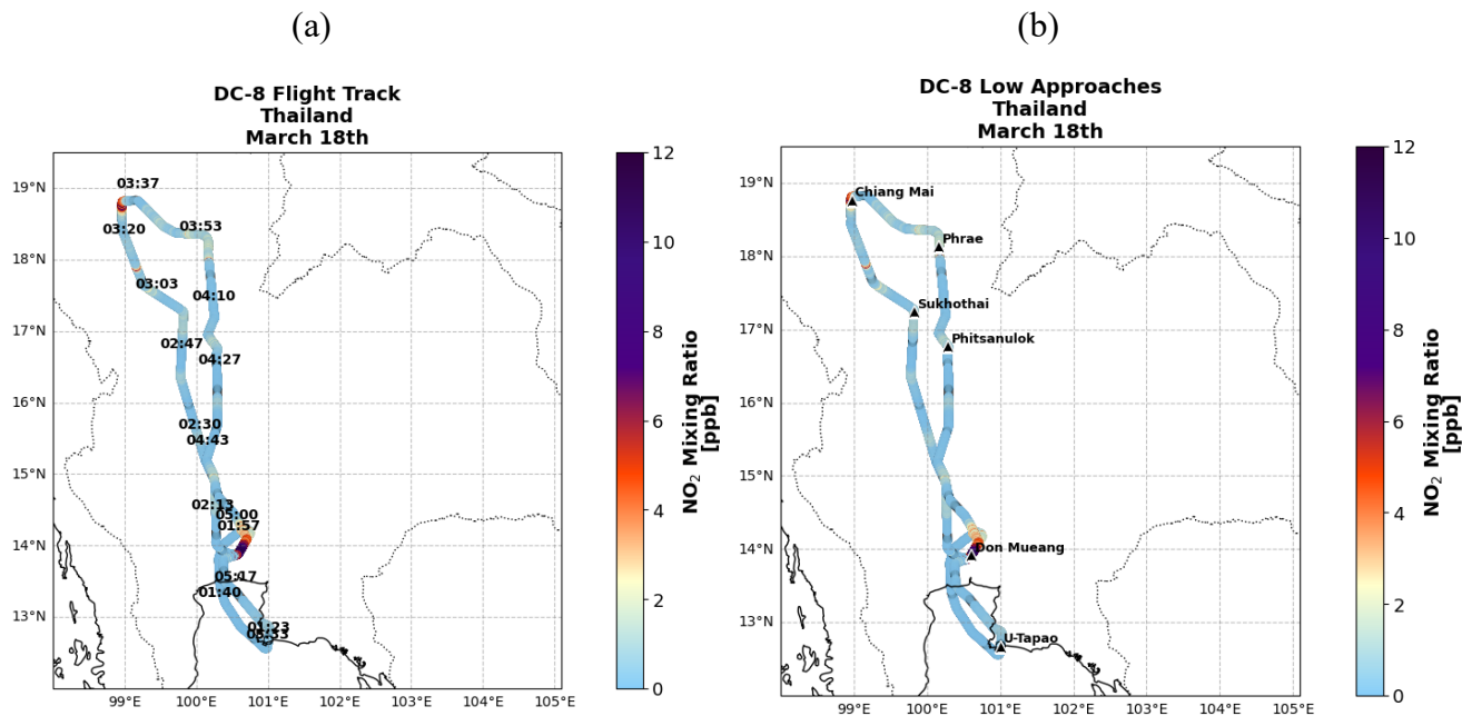
350 Figure S1920. (a) Typical DC-8 flight track during the Thailand-led ASIA-AQ field campaign. The aircraft departed from U- 351 Tapao Rayong Pattaya International Airport and flew northward across Bangkok and central Thailand toward Chiang Mai. 352 (b) Locations of airports where the DC-8 conducted low approaches for profiling and sampling surface air quality (U-Tapao, 353 Don Mueang, Phitsanulok, Sukhothai, Phrae, and Chiang Mai). NO 2 mixing ratios (ppbv) measured by NCAR's NO x O 3 354 instrument are shown along the flight track, with time annotations indicated.
