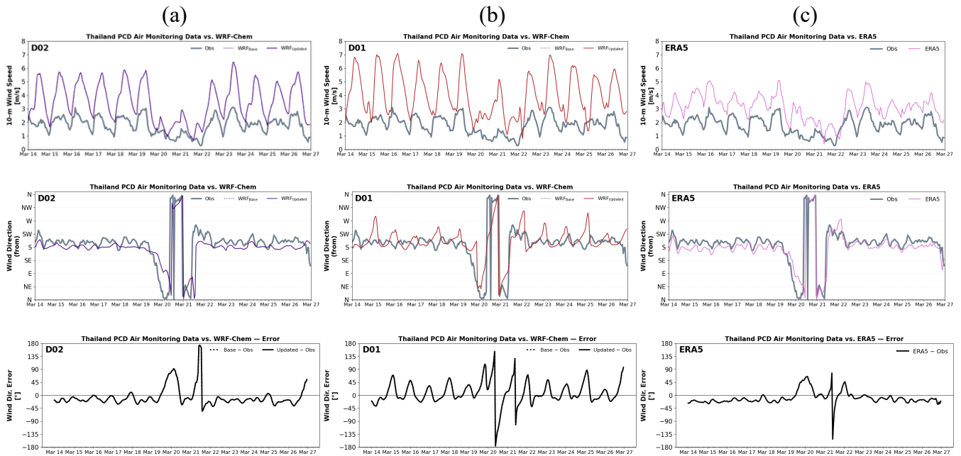
91 Figure S21. Comparison of (a) WRF Base D02 (purple), (b) WRF Base D01 (red), (c) ERA5 (pink) to Thailand Pollution Control 92 Department (PCD) ground-monitor network (grey) wind speed ( \text{m s}^{-1} ), wind direction (from), and wind direction error during 93 the ASIA-AQ deployment period (14–27 March 2024). Lines represent averages across stations within the BMR and 94 surrounding regions. Both model domains and ERA5 overestimate wind speeds relative to surface observations, potentially 95 due to unresolved urban canopy effects. These results suggest that improved urban parameterizations (e.g., a multi-layer urban 96 canopy model) could enhance model performance. Error diagnostics also highlight misrepresentation of a short-lived 97 northeasterly wind event on 20–21 March, leading to temporary errors in simulated transport direction.
