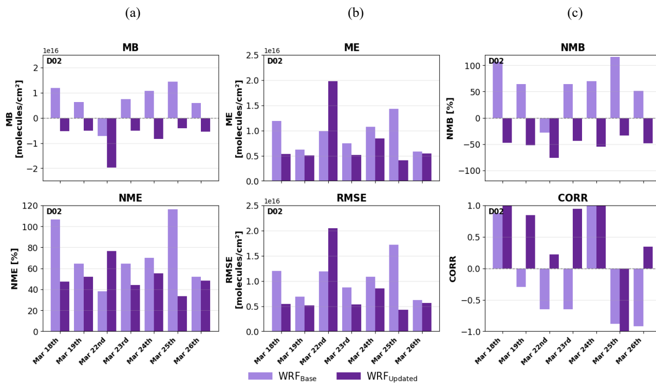
Figure S1516. Same as Figure S14, but for WRF Base D02 (light purple) and WRF Updated D02 (dark purple) evaluated against Pandora observations during the ASIA-AQ deployment period (14–27 March 2024).
