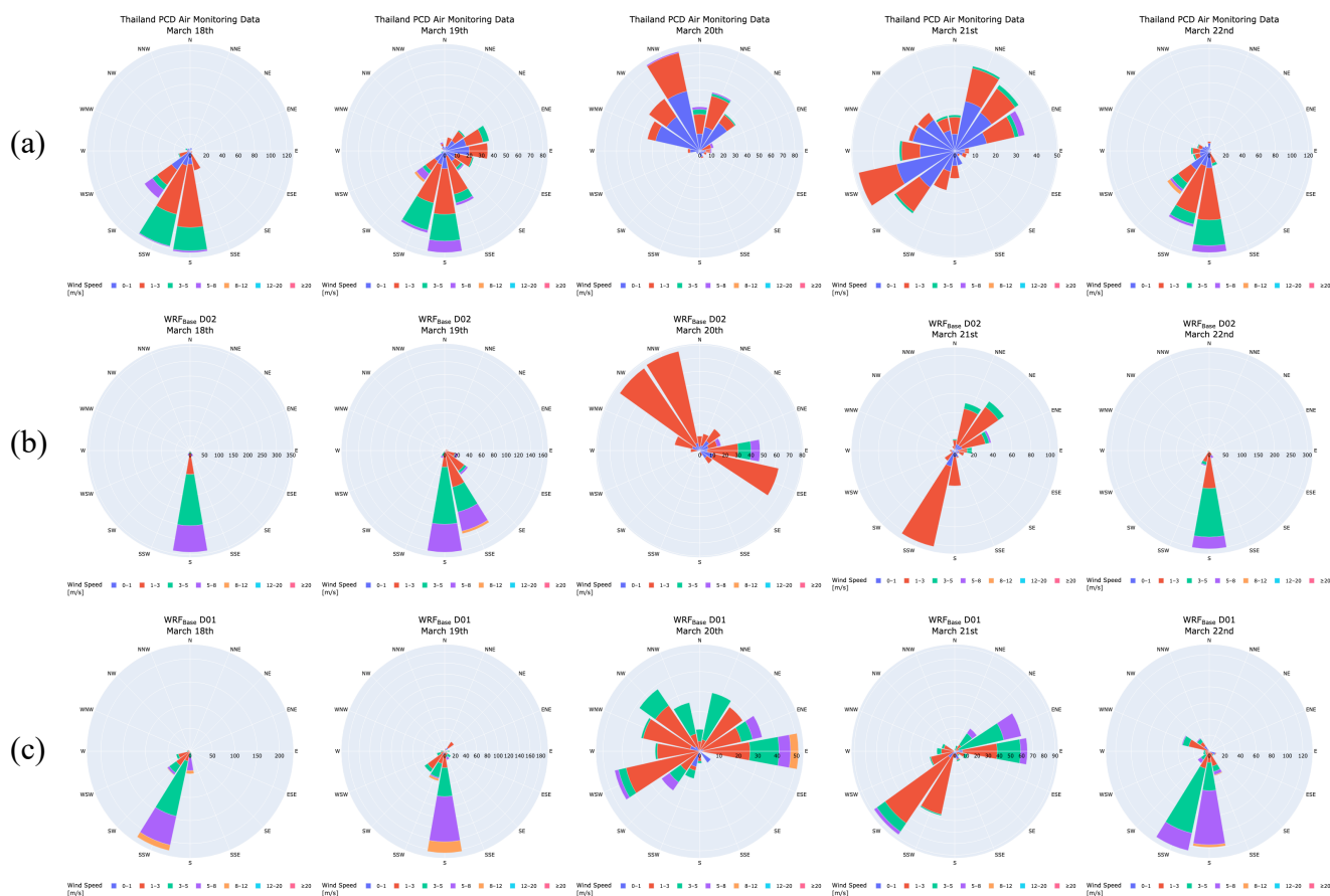
208 Figure S940. Comparison of observed wind roses (a) with modelled wind roses from (b) WRF Base D02 and (c) WRF Base D01 209 over the BMR for 18–22 March 2024. Panels show the frequency distribution of wind speed and direction. While the model 210 captures the dominant southerly flow, wind speeds are consistently overpredicted in both domains. The largest discrepancies 211 occur on 20–21 March, when the model fails to capture the observed shift toward northeasterly winds, likely contributing to 212 transport and concentration errors during this period.
