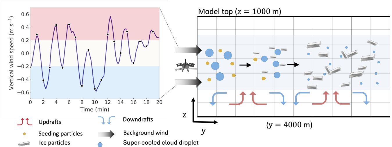
Figure 2. One-minute running average of the vertical wind speed in the grid cells where ice-nucleating particles (INPs) are released—and. The dots indicate the specific vertical wind speeds at the 20 distinct initiation times for the ensemble members. (b) schematic illustration of the computational domain after the spin-up period. Cloud seeding is performed between the coordinates (950, 10, 310) and (1050, 10, 310) m.
