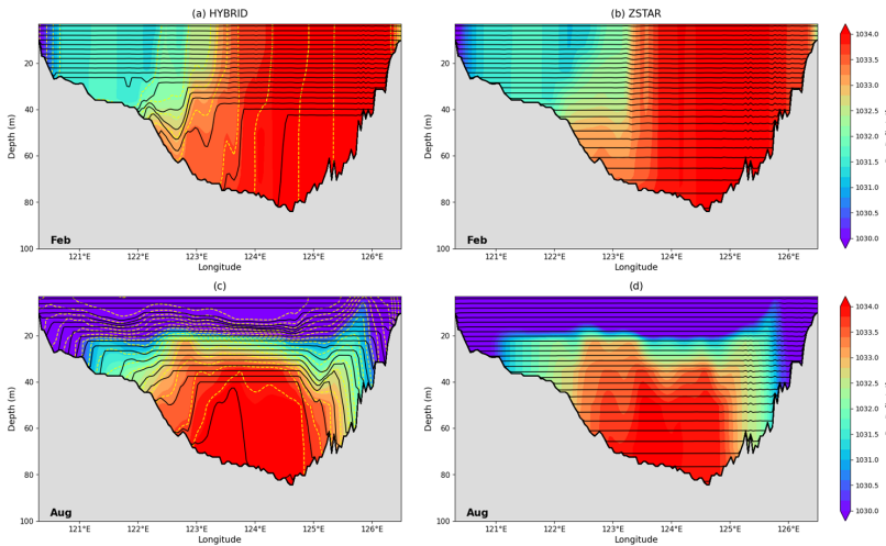
675 Figure 15: Zonal sections of the model interfaces and density along 36°N in the Yellow Sea for HYBRID and ZSTAR on (a–b) February 8 and (c–d) August 8. The background color contours represent potential density referenced to 2000 dbar. Black lines denote model layer interfaces and yellow dashed lines indicate target density surfaces used in the HYBRID configuration.
