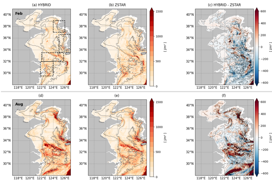
460 Figure 9: Depth-integrated baroclinic kinetic energy ( \text{J m}^{-2} ) for M_2 simulated by HYBRID and ZSTAR in the Yellow Sea, calculated from the first 15 d of each month’s simulation. Panels (a–b) and (d–e) show the February and August distributions for each configuration, respectively. Panels (c, f) present the differences between HYBRID and ZSTAR. The gray contours represent the 20, 50, and 80 m isobaths. The black boxes in panel (a) denote four energetic tidal regions used for quantitative evaluation through spatial averaging.
