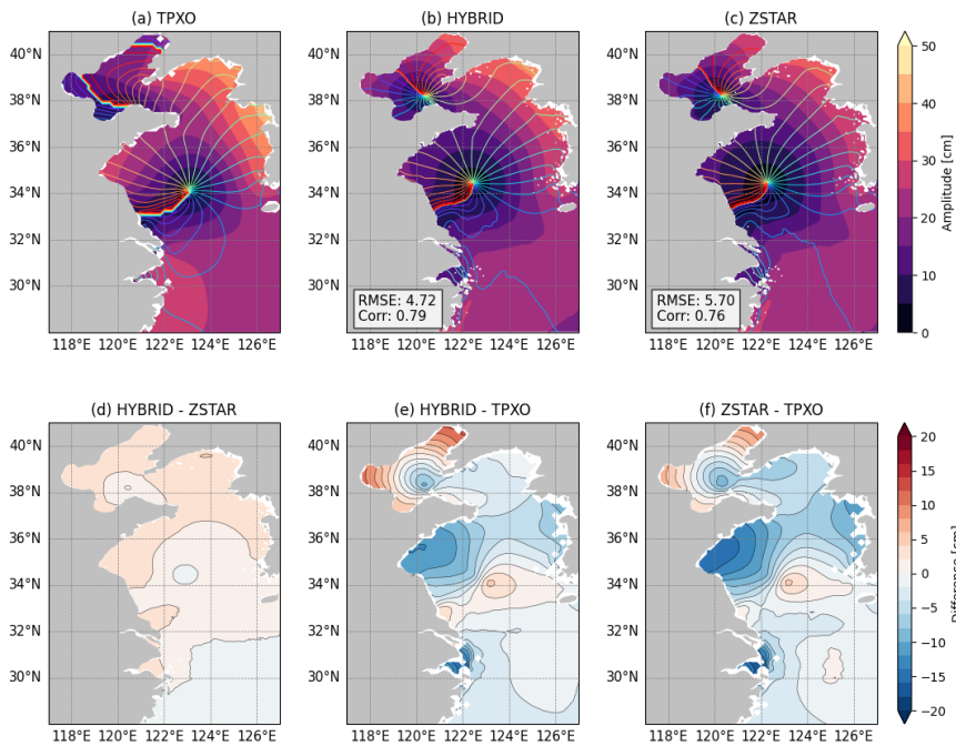
Figure 7: Spatial distribution of the diurnal K_1 tidal amplitude and phase from (a) TPXO, (b) HYBRID, and (c) ZSTAR in the Yellow Sea. Shaded contours indicate amplitude (cm) and colored lines denote phase. Panels (d-f) show amplitude differences: (d) HYBRID - ZSTAR, (e) HYBRID - TPXO, and (f) ZSTAR - TPXO. The spatial RMSE and Corr between each model and TPXO are also provided to quantify model performance.
