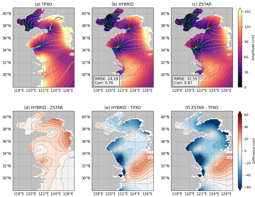
365 Figure 6: Spatial distribution of the semidiurnal M_2 tidal amplitude and phase from (a) TPXO, (b) HYBRID, and (c) ZSTAR in the Yellow Sea. Shaded contours indicate amplitude (cm) and colored lines denote phase. Panels (d–f) show amplitude differences: (d) HYBRID – ZSTAR, (e) HYBRID – TPXO, and (f) ZSTAR – TPXO. The spatial RMSE and Corr between each model and TPXO are also provided to quantify model performance.
