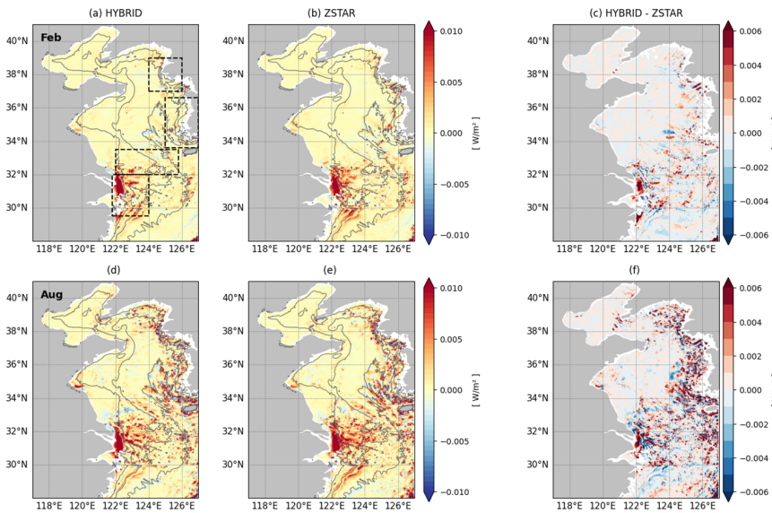
535 Figure 12: Depth-integrated barotropic to baroclinic energy conversion ( W m^{-2} ) for M_2 simulated by HYBRID and ZSTAR in the Yellow Sea, calculated from the first 15 d of each month's simulation. Panels (a–b) and (d–e) show the February and August distributions for each configuration, respectively. Panels (c, f) present the differences between HYBRID and ZSTAR. The gray contours represent the 20, 50, and 80 m isobaths. The black boxes in panel (a) denote four energetic tidal regions used for quantitative evaluation through spatial averaging.
