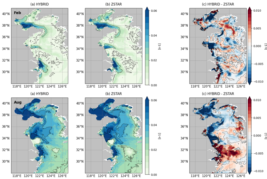
330 Figure 5: Spatial distribution of the depth-averaged buoyancy frequency in the Yellow Sea during February (top row) and August (bottom row). Panels (a, d) and (b, e) show the buoyancy frequencies from the HYBRID and ZSTAR configurations, respectively. Panels (c, f) present the difference between the two configurations (HYBRID – ZSTAR).
