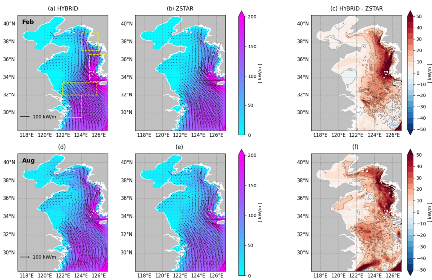
410 Figure 8: Barotropic tidal energy flux vectors its magnitudes for the M_2 constituent in the Yellow Sea, calculated from the first 15 d of each month's simulation. Panels (a–b) show fluxes and magnitudes for February and panels (d–e) for August, as simulated by HYBRID (left) and ZSTAR (right). Panels (c, f) present the differences in barotropic tidal energy magnitudes between HYBRID and ZSTAR. Arrows indicate the direction and magnitude of energy flux (units in \text{kW m}^{-1} ). The yellow boxes in panel (a) denote four energetic tidal regions used for quantitative evaluation through spatial averaging. 415
