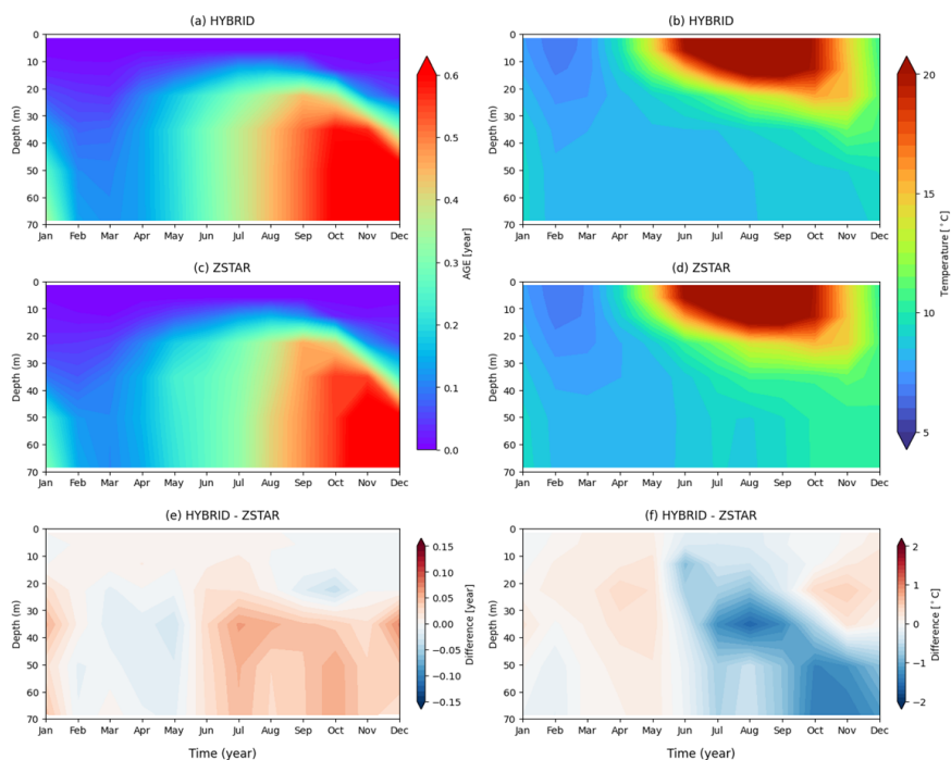
Figure 13: Seasonal evolution of age tracer (left) and temperature (right) at a fixed location in the central Yellow Sea ( 124^{\circ} E, 36^{\circ} N) based on monthly climatology over a 10-y period (2003–2012). Panels (a)–(b) show results from HYBRID and panels (c)–(d) show the corresponding fields from ZSTAR. Panels (e)–(f) present the differences between HYBRID and ZSTAR (HYBRID – ZSTAR) for the age tracer and temperature, respectively.
