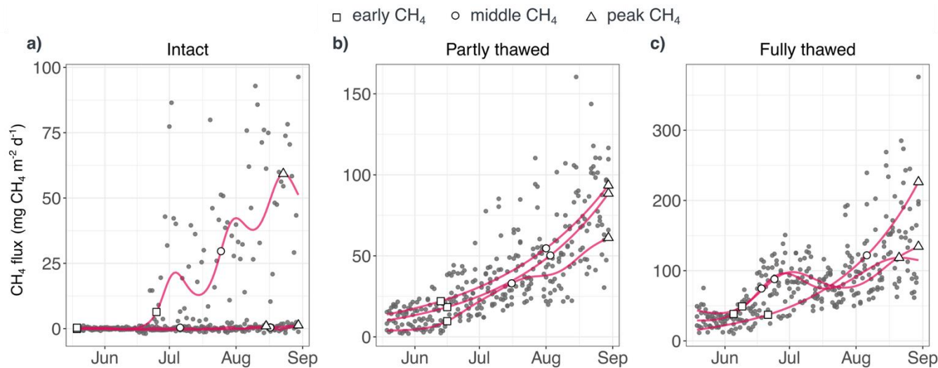
700 Figure B10: Daily median CH 4 flux with CH 4 flux period values over the productive season at intact (a), partly thawed (b) and fully thawed (c) stages. a-c) Red lines represent chamber-specific GAM fit ( R^2 \geq 0.3 ), except for one chamber in a) where GAM R^2 < 0.1 , and the line represents the moving 7-day median CH 4 flux. Squares represent early, circles middle and triangles peak CH 4 flux season. See chamber GAM R^2 in Table C5.
