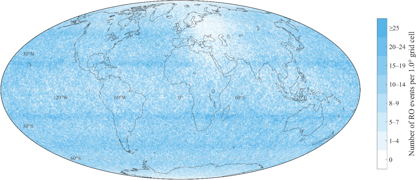
Global Multi-Mission RO Event Counts (1.0° Grid)
