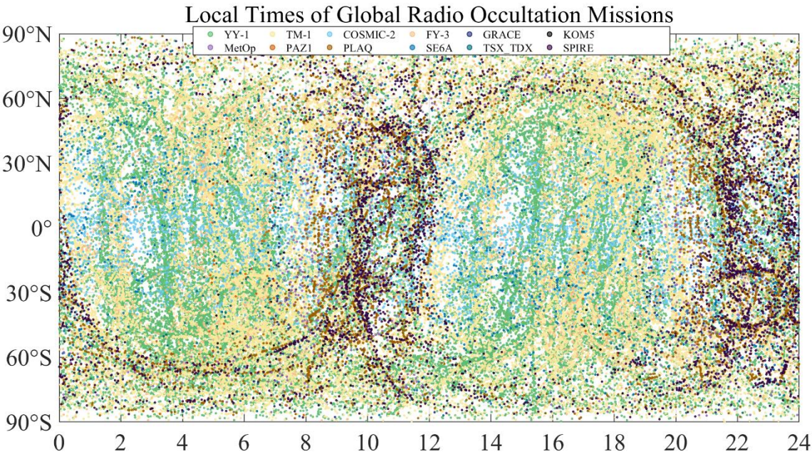
361 362 Figure 8. Local-time distribution of the combined radio occultation dataset on 1 January 2026.
