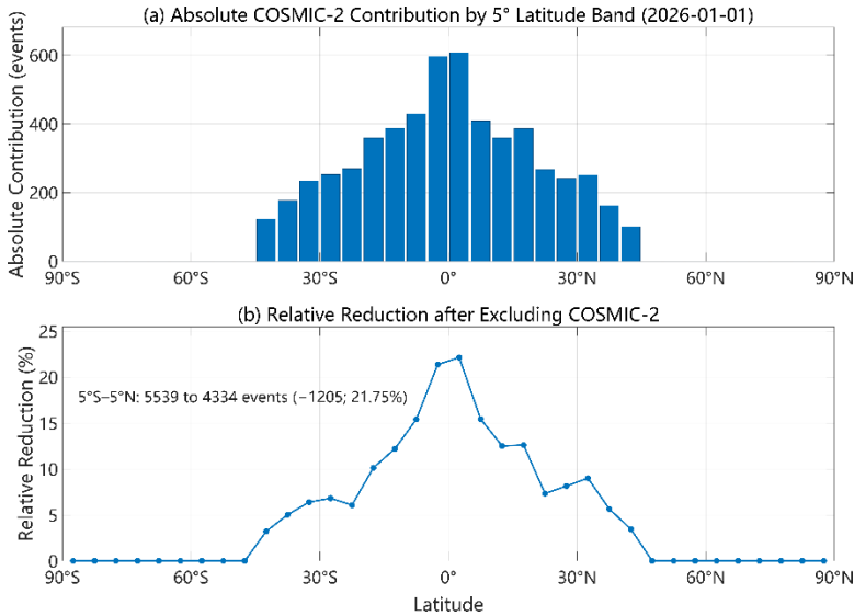
396 397 Figure 10. Sampling contribution of COSMIC-2 by 5° latitude band on 1 January 2026: (a) the absolute number of events removed 398 when COSMIC-2 is excluded, \Delta N = N_{12} - N_{11} ; and (b) the corresponding percentage reduction, 100\Delta N / N_{12} .
