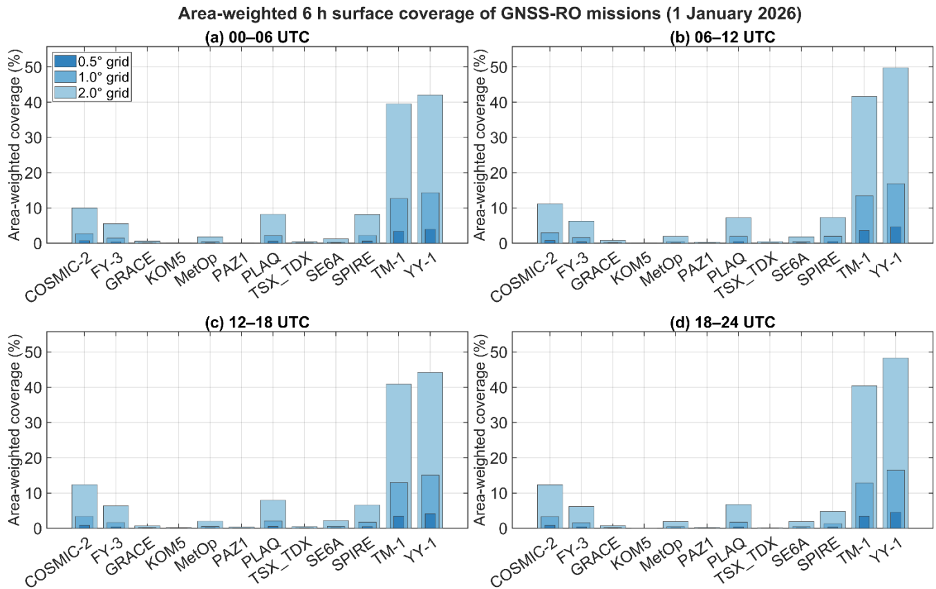
291 Figure 5. Area-weighted surface coverage of individual GNSS-RO missions within 6 h time windows on 1 January 2026.
