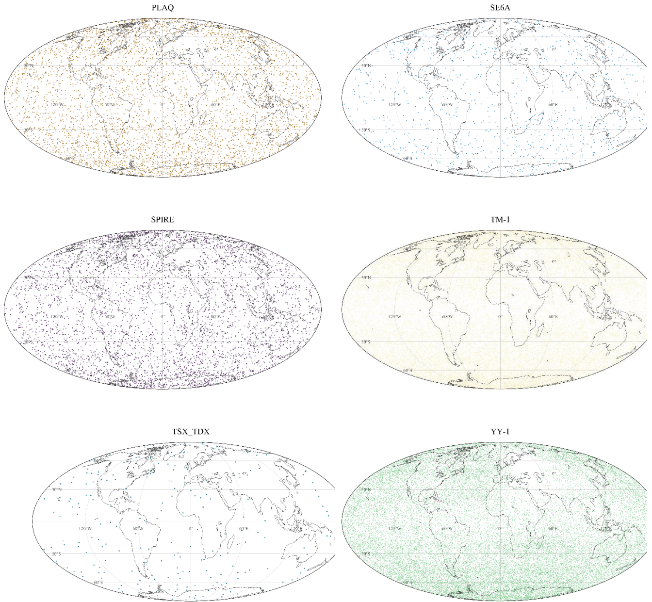
Figure 2. Global distribution of radio occultation events from individual missions on 1 January 2026. The distributions are shown using a Mollweide equal-area projection.
