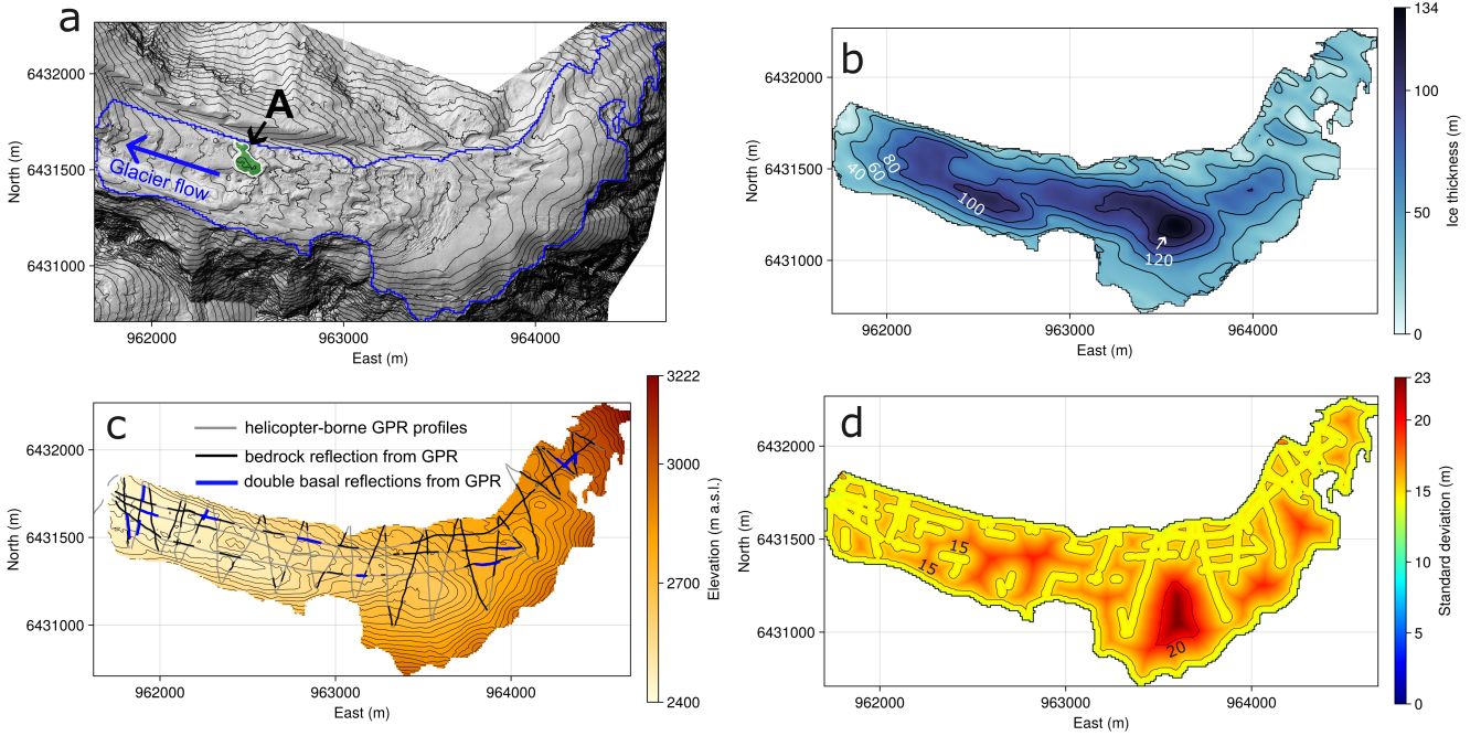
Figure 2. Surface elevation hillshade (a), ice thickness (b), bedrock elevation (c), and bedrock elevation uncertainties ( \pm standard deviation)(d) for Glacier de Bonne Pierre in October 2024. Black and blue lines in panel (c) indicate where bedrock elevation was obtained by GPR measurements; blue lines indicate where double basal reflections from GPR suggest the presence of subglacial channels. The letter A in panel (a) marks the location of the supraglacial lake that drained during the flood event in June 2024 (lake area in green). Contour intervals are 20 m for panels (a), (b) and (c), and 10 m for panel (d). The glacier outline refers to the year 2022.
