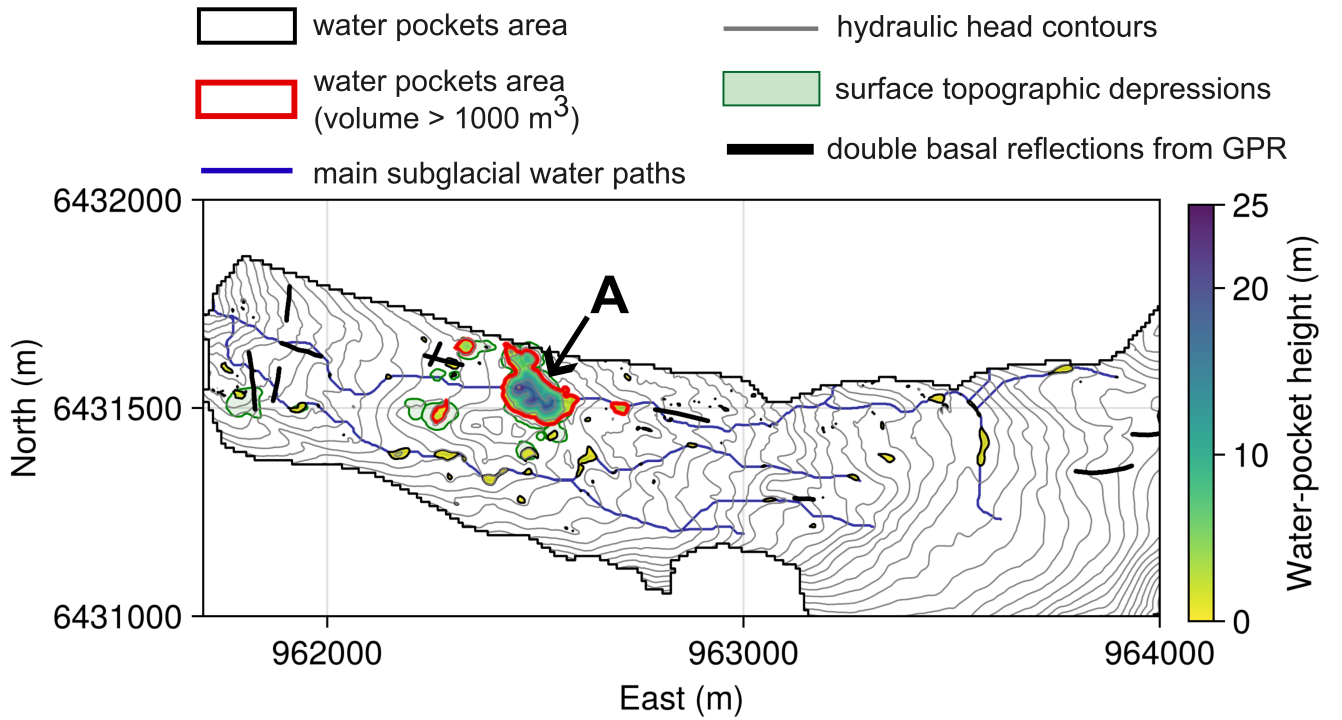
Figure 3. Distributed water-pocket water-pocket height and main subglacial water paths governed by hydraulic head modelled at Glacier de Bonne Pierre for June 2024 (only the tongue is shown here). The hydraulic head field is shown with thin grey contours at 10 m intervals. Potential water pockets larger than 10^3 \text{ m}^3 are outlined in red (in purple black if smaller). The main surface depressions in the DEM of August 2024 are shown by green shading. The letter A marks both the location of the largest water pocket ( 148 148 \cdot 10^3 \text{ m}^3 ) and the location of the supraglacial lake observed in June 2024. Only the subglacial flow paths (blue lines) with an upslope catchment area larger than 10^5 \text{ m}^2 are displayed for visualization (using f = 1 in Eq. (2)). Thick black lines show double basal reflections from GPR reflection that suggested suggest the presence of subglacial water channels . Glacier outline corresponds to the year 2022.
