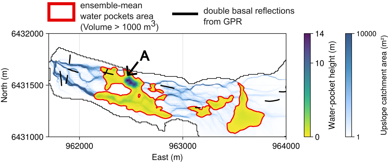
Figure 4. Ensemble-mean water-pocket water-pocket height and upslope catchment areas from 1000 stochastic realizations of the hydraulic head field at Glacier de Bonne Pierre for June 2024. Only merged outlines of ensemble-mean subglacial water pockets larger than 10^3 \text{ m}^3 are shown (in red). The letter A marks the location of the supraglacial lake observed in June 2024. Black lines indicate GPR-double basal from GPR reflections from GPR interpreted as subglacial water water channels.
