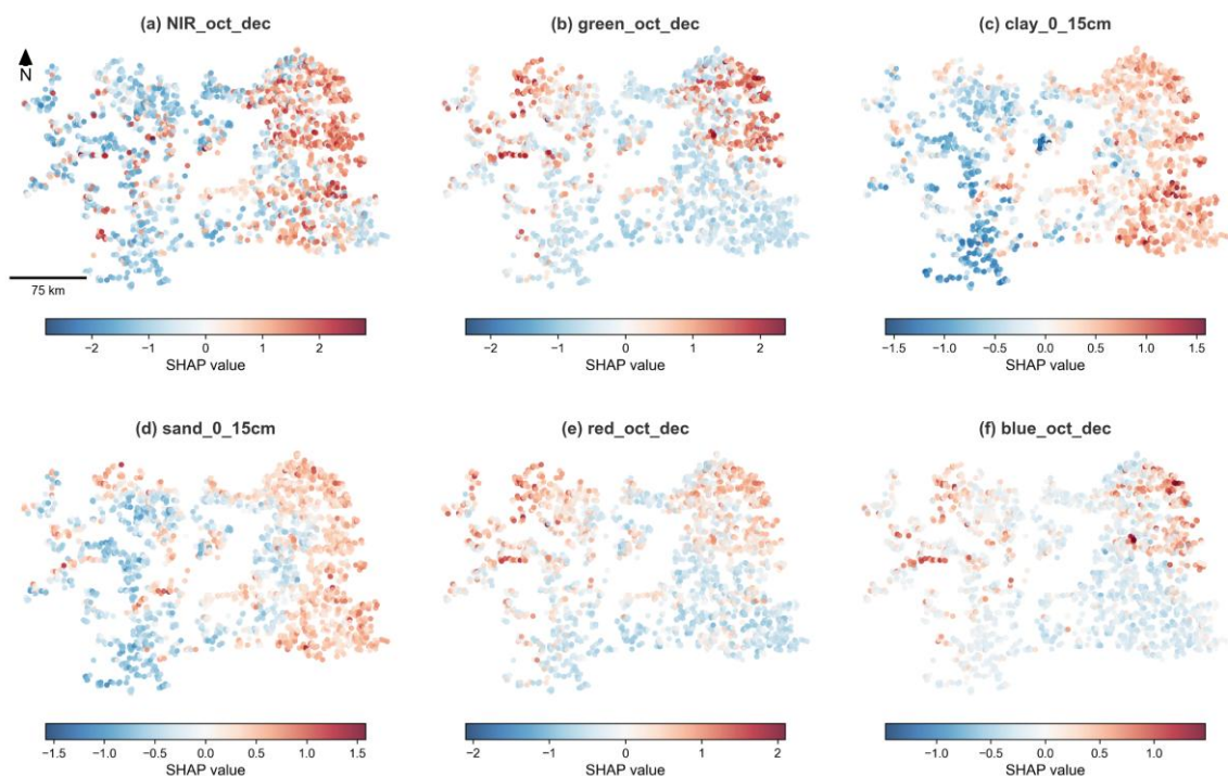
Figure 9 Spatial distribution of SHAP values for the optimal Oct–Dec model. The diverging maps illustrate the directional impact of the top six covariates: (a) NIR band, (b) green band, (c) clay [0–15cm], (d) sand [0–15cm], (e) red, and (f) blue band on predicted SOC. The colour gradient indicates the strength and direction of a feature's effect on the model output: red dots represent positive SHAP values (the variable drives SOC prediction higher at this location), while blue dots denote negative SHAP values (the variable drives SOC prediction lower at this location).
