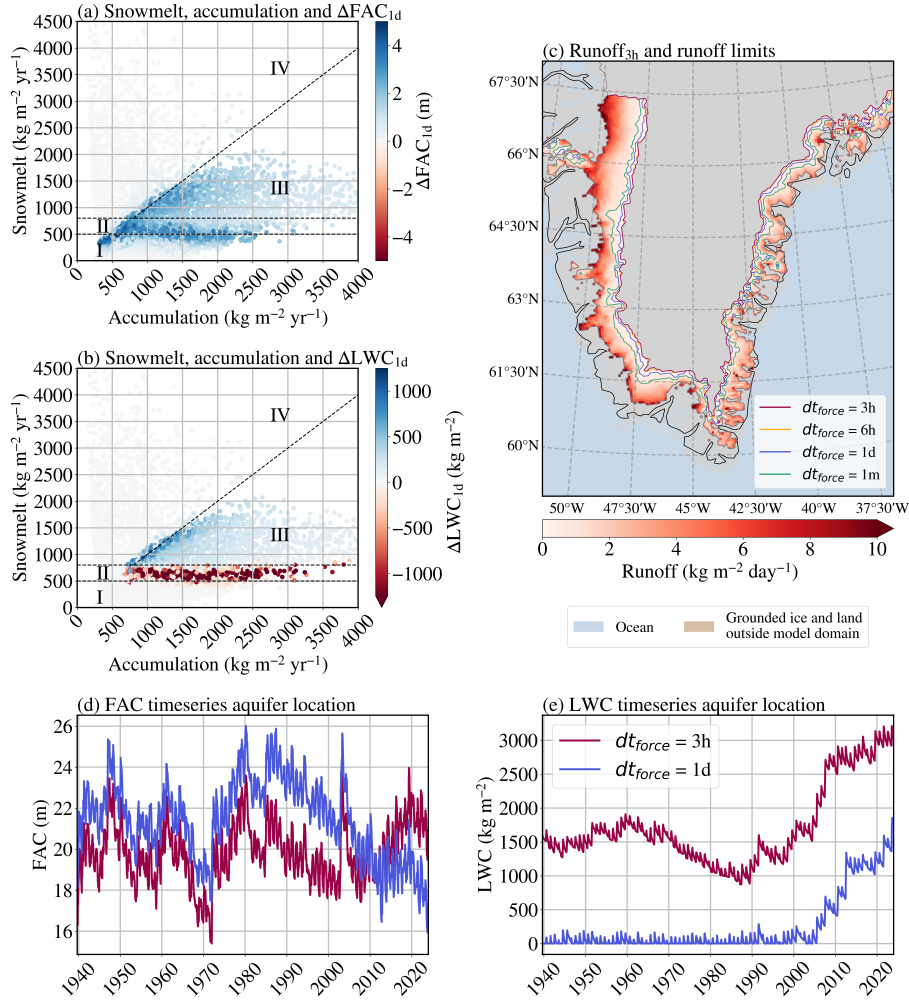
Figure 10. Average snowmelt against accumulation over 1939-1970 colour coded with average \Delta\text{FAC}_{1d} (a) and \Delta\text{LWC}_{1d} (b) over the simulation period. The black dashed lines represent snowmelt of 500 \text{ kg m}^{-2} \text{yr}^{-1} (climate zone I), 500\text{-}800 \text{ kg m}^{-2} \text{yr}^{-1} (climate zone II) and a MOA of 1 (separating climate zones III and IV). Panel (c) shows the average runoff 3h over the simulation period and the different runoff limits for the four dt_{force} . Panel (d) and (e) show timeseries of respectively \text{FAC}_{3h} and \text{FAC}_{1d} , and \text{LWC}_{3h} and \text{LWC}_{1d} . See Fig. 3e for a map with the grid cell location.
