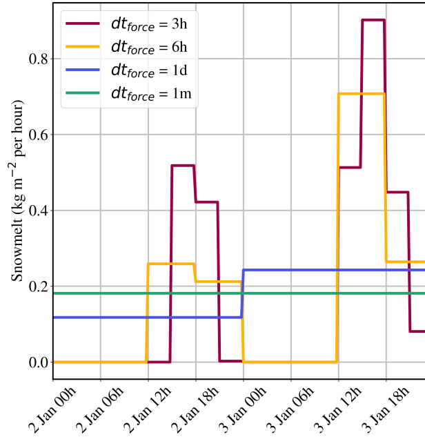
Figure 1. Example of 48 hours of snowmelt forcing at dt_{force} = 3h , 6h , 1d , and 1m . The graph also visualizes the model's interpolation of the forcing onto a 15-minute timestep. Note the presence of a diurnal cycle in the snowmelt input for dt_{force} = 3h and 6h and its absence for dt_{force} = 1d and 1m .
