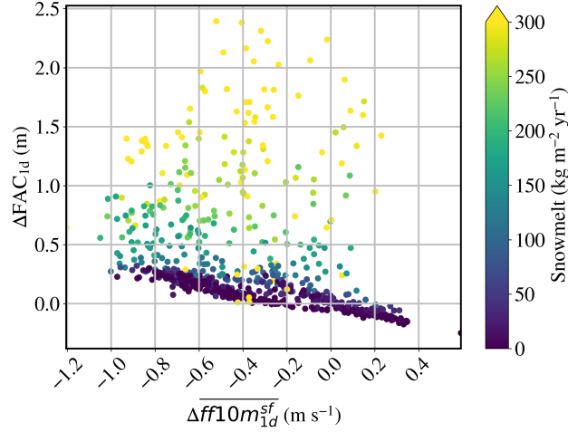
Figure 8. The \Delta \text{FAC}_{1d} against \Delta \overline{ff10m}_{1d}^{sf} in the APIS. \Delta \overline{ff10m}_{1d}^{sf} = \overline{ff10m}_{1d}^{sf} - \overline{ff10m}_{3h}^{sf} . In absence of melt, there is a clear relation between \Delta \overline{ff10m}_{1d}^{sf} and \Delta \text{FAC}_{1d} .
