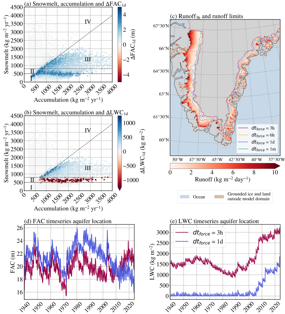
Figure 10. Average snowmelt against accumulation over 1939-1970 colour coded with average \Delta \text{FAC}_{1d} (a) and \Delta \text{LWC}_{1d} (b) over the simulation period. The black dashed lines represent snowmelt of 500 \text{ kg m}^{-2} \text{yr}^{-1} (climate zone I), 500\text{-}800 \text{ kg m}^{-2} \text{yr}^{-1} (climate zone II) and a MOA of 1 (separating climate zones III and IV). Panel (c) shows the average runoff 3h over the simulation period and the different runoff limits for the four dt_{force} . Panel (d) and (e) show timeseries of respectively \text{FAC}_{3h} and \text{FAC}_{1d} , and \text{LWC}_{3h} and \text{LWC}_{1d} . See Fig. 3e for a map with the grid cell location.
