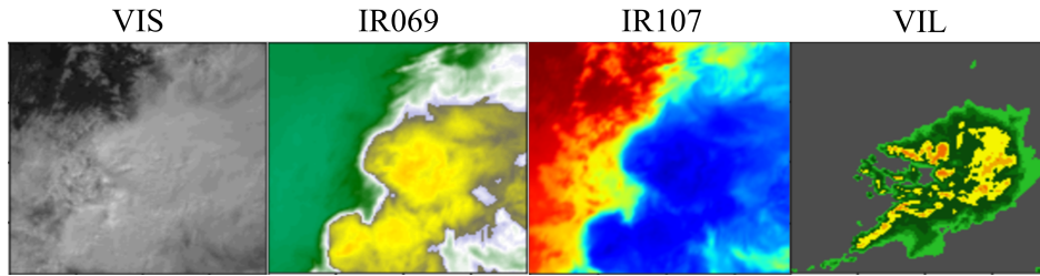
Figure 1. VIL, IR107, VIS, and IR069 represent the radar vertical liquid water content, the satellite infrared longwave window, the visible satellite imagery, and the satellite mid-level water vapor, respectively. Among them, VIL represents precipitation data, while VIS, IR107 and IR069 serve as additional meteorological information.
