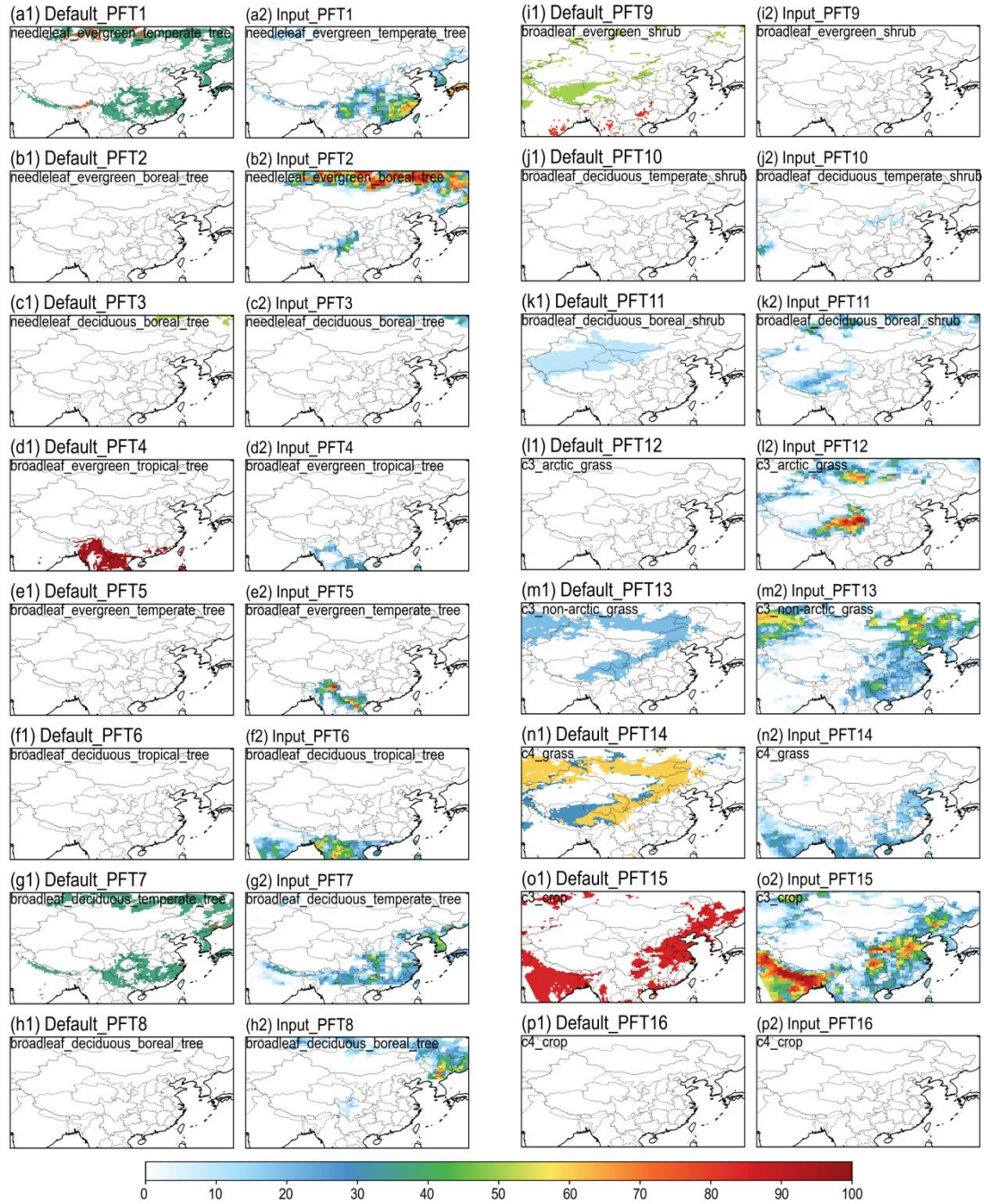
Figure S1: Comparison of default PFTs and their percentages in WRF-CLM4 with those inputted into WR-CLM5.
