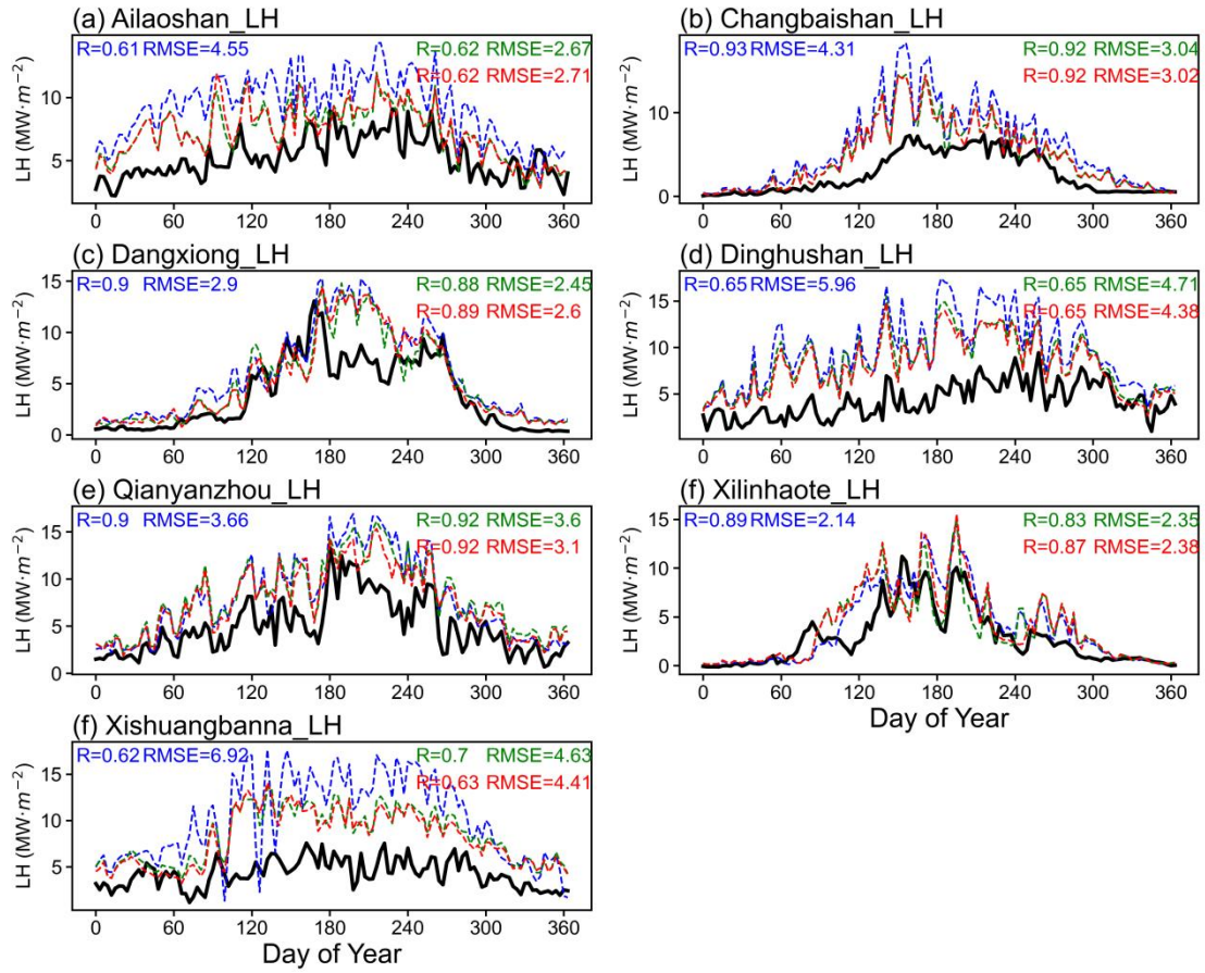
Figure S4: Same as Figure S4, but for LH.
