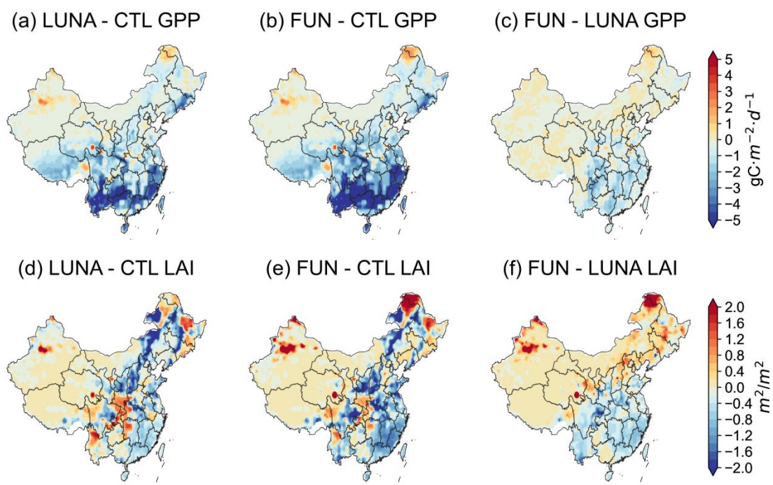
Figure S2: (a-c) The differences of GPP among three simulation experiments, and (d-f) the differences of LAI among three simulation experiments.
