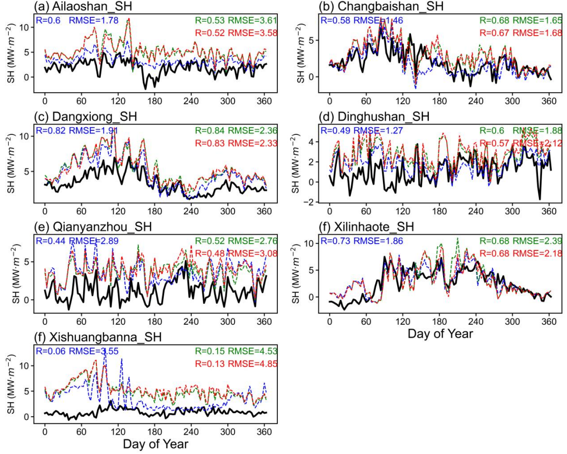
Figure S3: (a-c) The SH series at seven in-situ observation sites, with values derived from eddy-covariance observation (black solid line), Exp_CTL (blue dashed line), Exp_LUNA (green dashed line), and Exp_FUN (red dashed line).
