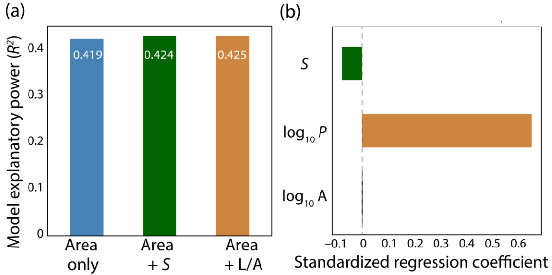
Fig. S6. Contribution of network-structure proxy to functional scaling. (a) Comparison of model explanatory power ( R^2 ) among models using drainage area alone and models additionally incorporating network-structure proxy ( S and L/A ). (b) Standardized regression coefficients of predictors in the extended model. The inclusion of network-structure proxy results in a small improvement in model performance. Standardized coefficients indicate that precipitation explains a larger proportion of variation than river-network structure, although the latter retains measurable effects.
