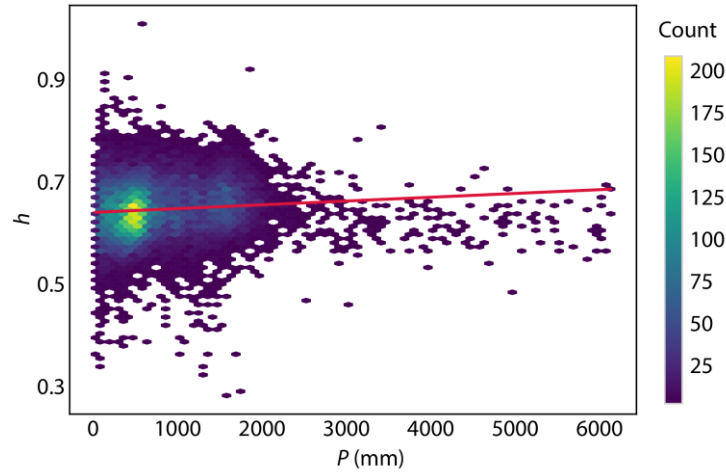
Fig. S1. Relationship between Hack's law exponent and precipitation. Hexagonal binning plot showing the distribution of Hack's law exponent ( h ) across the precipitation gradient ( P ). Colors indicate observation density, and the red line represents the fitted linear trend. The scaling exponent exhibits a weak positive association with precipitation, which suggests that climatic conditions may contribute to variations in river-network scaling structure.
