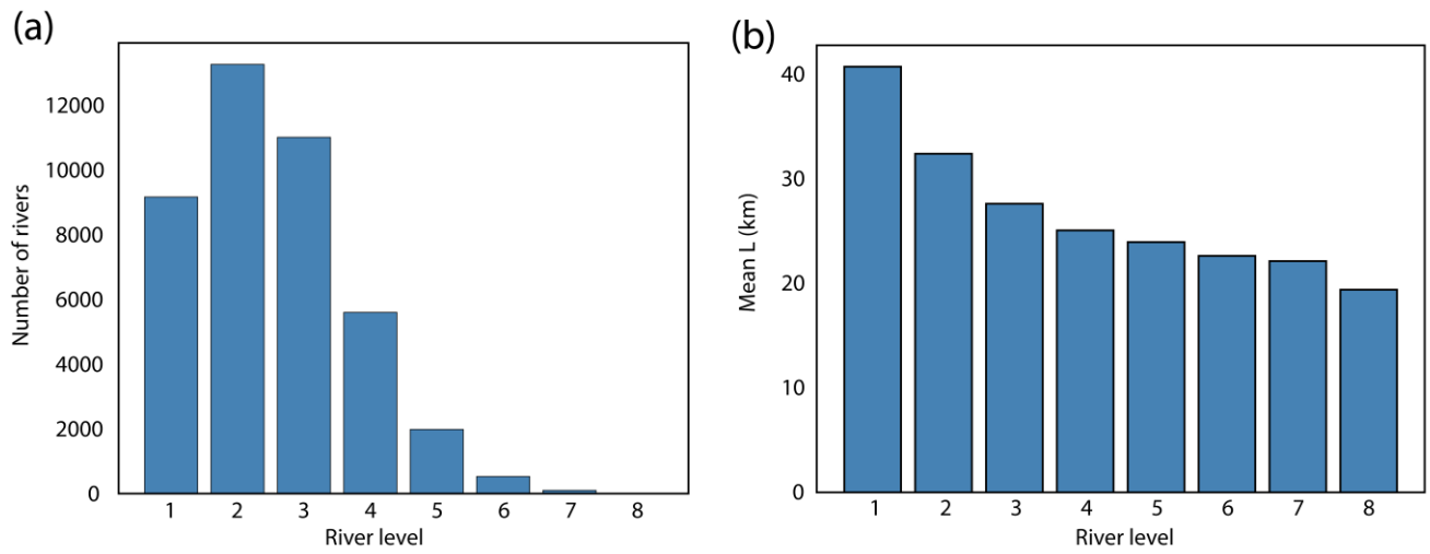
Fig. S3. Characteristics of river levels in the analyzed river network. (a) Distribution of river numbers among river levels. (b) Mean river length ( L ) associated with each river level.
