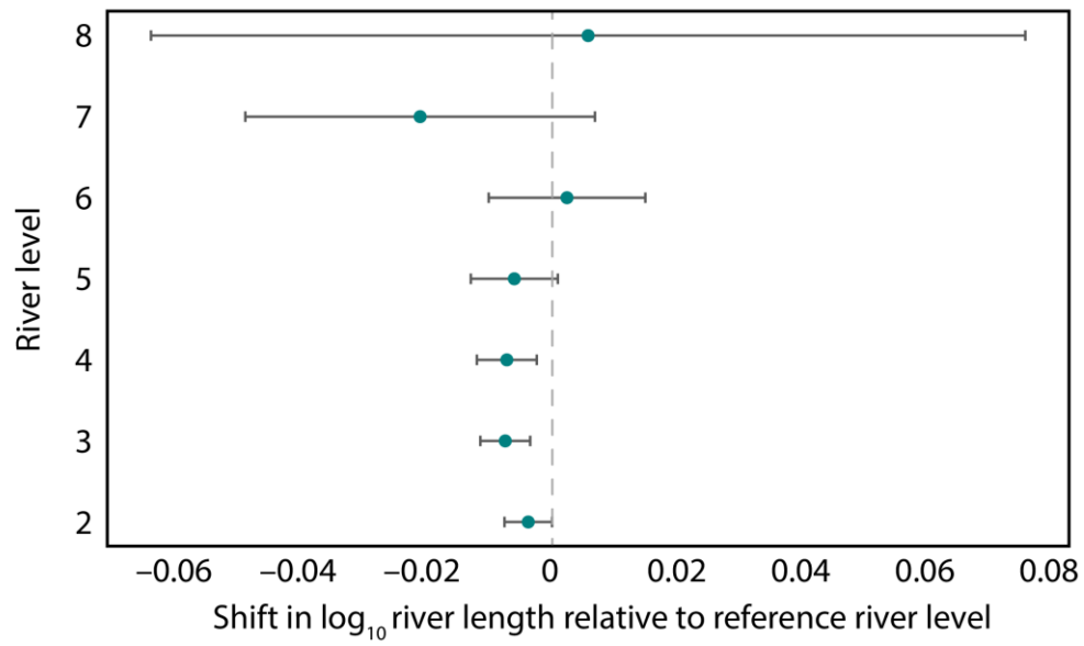
Fig. S4. Consistency of Hack's law across river levels. River-level dummy coefficients from a regression model of \log_{10} L against \log_{10} A . Coefficient estimates are expressed relative to the reference river level. The generally small effect sizes indicate that river-level differences contribute little to the observed geometric scaling relationship.
