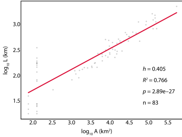
Fig. S2. Hack's law for representative main-stem rivers across China's major river basins. Relationship between river length ( L ) and drainage area ( A ) derived from one representative main-stem river selected from each basin ( n = 83 ). The fitted scaling exponent ( h = 0.405 ) is comparable to that obtained from the full river network dataset, which indicates that the observed geometric scaling relationship is robust to river selection.
