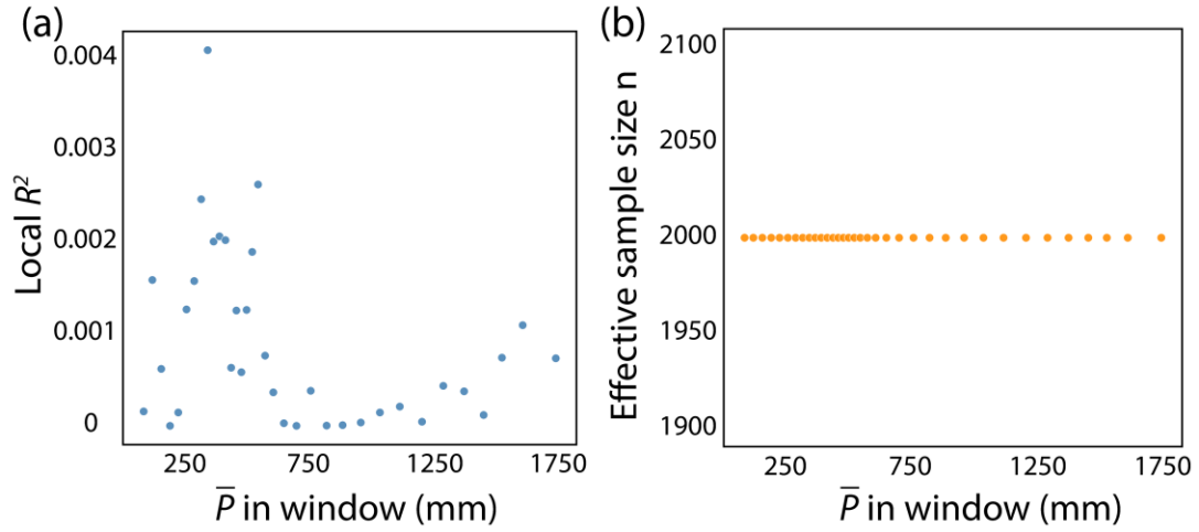
Fig. S5. Robustness of the moving-window analysis across the precipitation gradient. (a) Local goodness-of-fit ( R^2 ) of the moving-window regression along the precipitation gradient. (b) Effective sample size ( n ) within each moving window. The approximately constant sample size across windows indicates that variations in local model performance are not driven by differences in sample availability.
