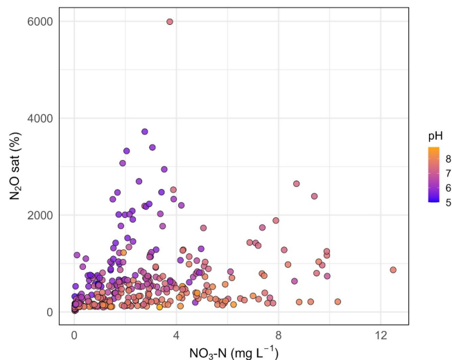
Figure 4. Nitrous oxide ( \text{N}_2\text{O} ) saturation versus nitrate ( \text{NO}_3^- -N) concentration. The color gradient indicates the pH in the stream water.
