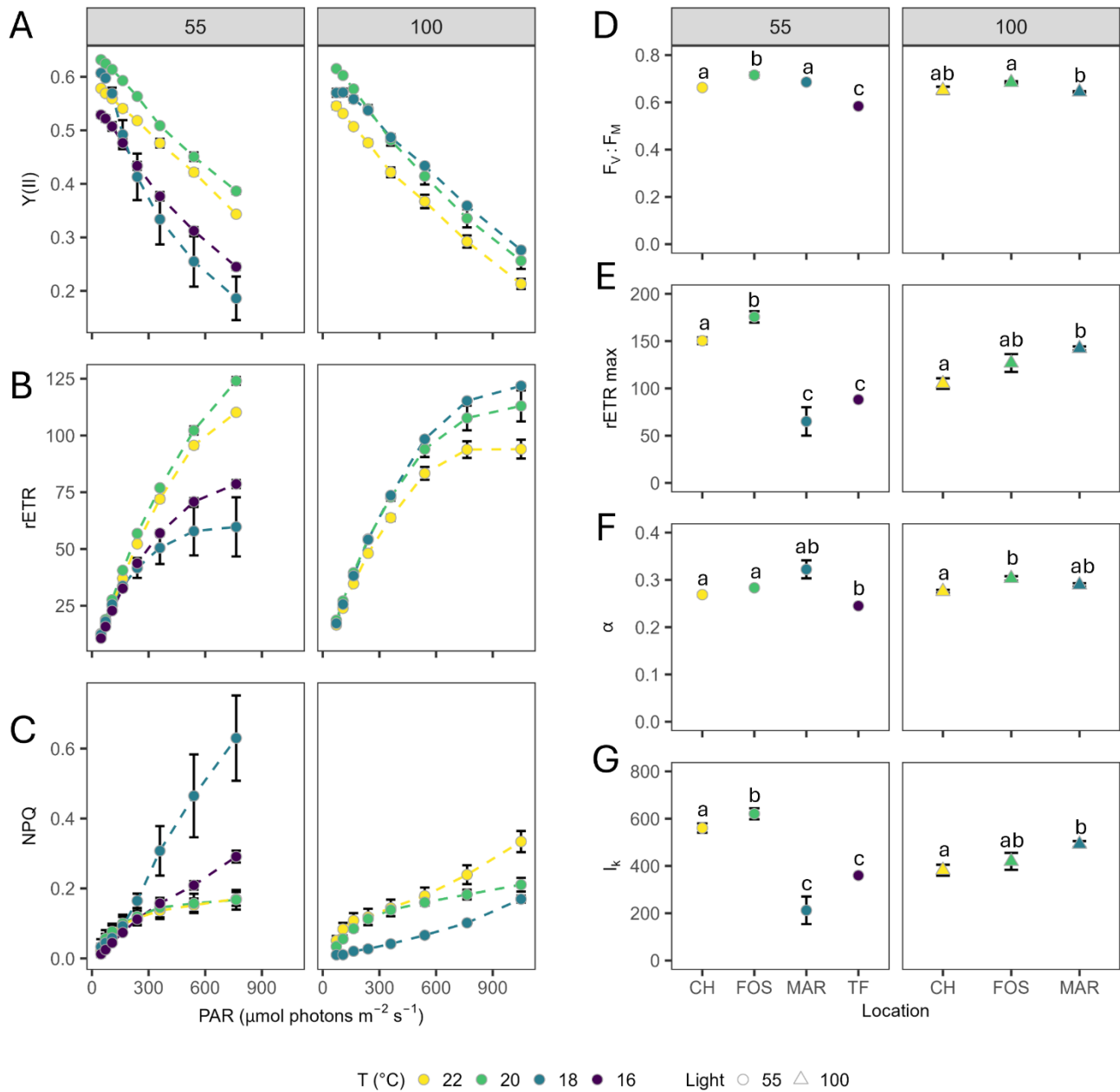
315 Figure 4: Chlorophyll fluorescence parameters. A Effective quantum yield of PSII [Y(II)], B relative electron transport rates (rETR), and C non-photochemical quenching (NPQ), as a function of irradiance (PAR), D maximum quantum yield of PSII ( F_V:F_M ), E maximum rETR max ( \mu\text{mol electrons m}^{-2} \text{s}^{-1} ), F light utilisation efficiency (alpha; \alpha ) and G minimum saturating irradiance ( I_k ( \mu\text{mol photons m}^{-2} \text{s}^{-1} )) determined for Leptocylindrus danicus strains acclimated to temperature conditions under
