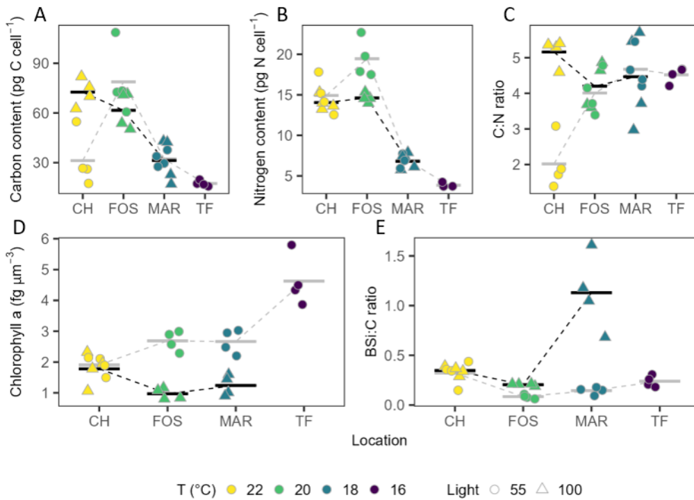
385 Figure 6: Elemental composition. A total carbon per cell (pg), B total nitrogen per cell (pg), C carbon to nitrogen ratio (C:N), D chlorophyll a per cell volume (fg μm -3 ), E biogenic silicate to carbon (bSi) ratio of Leptocylindrus danicus strains from low (circles) and high (triangles) light. Data are individual replicates ( n = 4 ) and horizontal bars represent their mean value. Stippled lines between means are provided as a visual guide.
