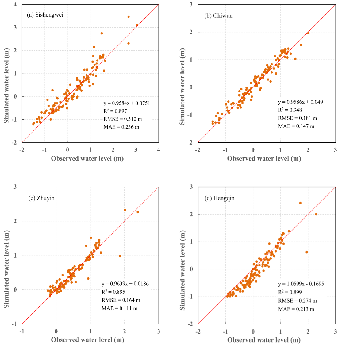
Figure 5. Comparison between the simulated and observed water levels during Typhoon Hato from 0:00 on August 20 to 0:00 on August 25.
