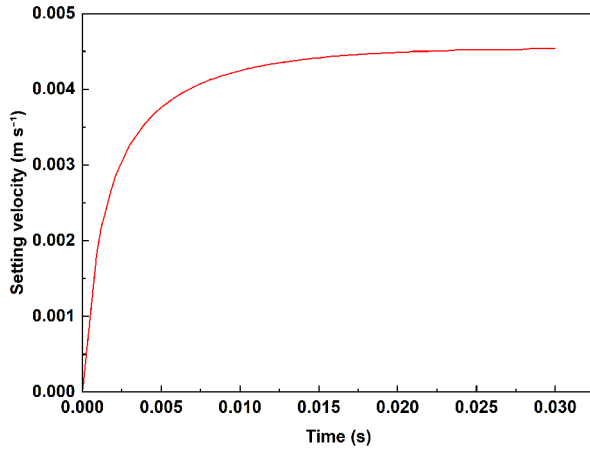
205 Figure 5. Temporal evolution of simulated settling velocity for 100-μm particles
