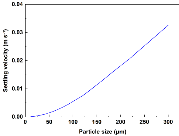
215 Figure 6. Effect of particle size on settling velocity
