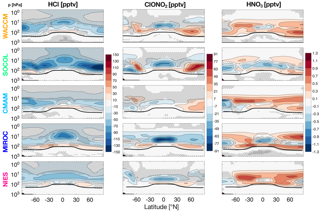
Figure 8. Zonal mean mixing ratio anomalies of hydrochloric acid, chlorine nitrate, and nitric acid mixing ratio [(\text{senD2-sai} - \text{senD2-fix}) / \text{senD2-fix}] caused by SAI for the period 2060-2079. Black lines: senD2-sai tropopause. Hatched areas: not significant at a 1 % level in a two-sample t-test.
