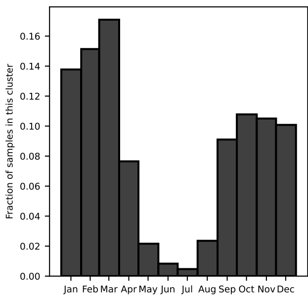
P(\mathcal{L} | N_d) Distribution (top 25% cluster matches)
