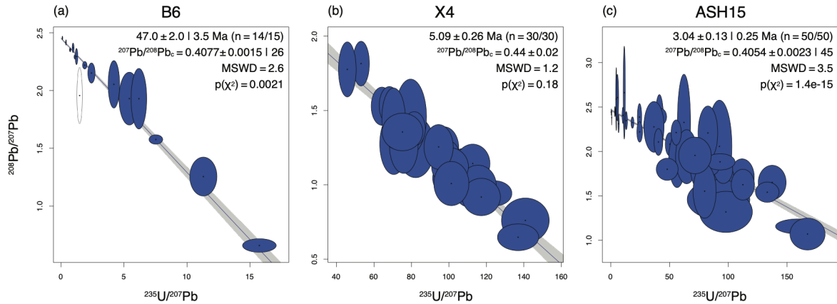
Figure 5: LA-ICPMS results for B6, X4, and ASH15 obtained with the ^{207}\text{Pb}/^{235}\text{U} method using a 380 \mu\text{m} diameter laser spot. All isochron dates are disequilibrium-corrected with initial [^{231}\text{Pa}/^{235}\text{U}] = 0 .
