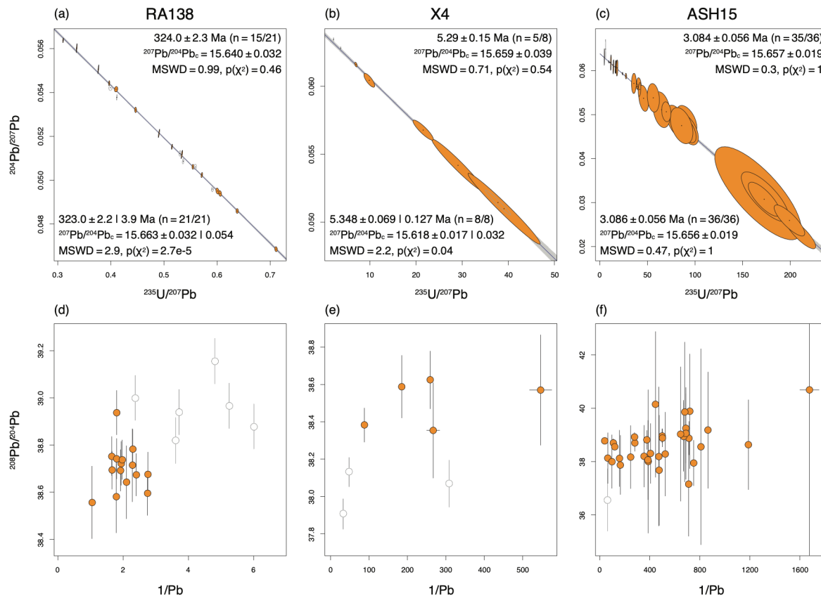
Figure 4: Utility of ^{208}\text{Pb}/^{204}\text{Pb} in carbonates as a tracer of contamination, and its effect on age interpretation. (a–c) ^{208}\text{Pb} -filtered (text near top and coloured ellipses) and unfiltered (bottom text, empty ellipses), ^{231}\text{Pa} -corrected ID-TIMS ^{207}\text{Pb}/^{235}\text{U} isochron dates for RA138, X4, and ASH15. (d–f) corresponding measured ^{208}\text{Pb}/^{204}\text{Pb} vs. 1/(\text{Pb ppm}) systematics and suggested exclusion of outliers (empty symbols).
