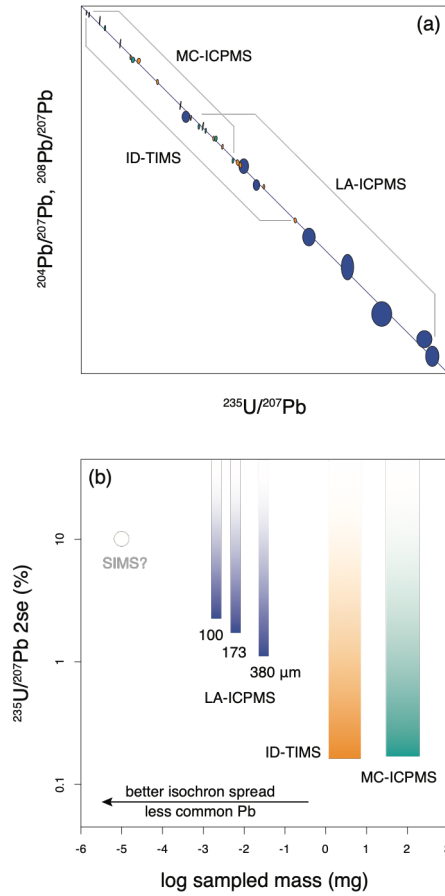
Figure 2: Schematic illustration of ^{207}\text{Pb}/^{235}\text{U} isochron data spread and precision expected from various analytical methods in a hypothetical radiogenic carbonate sample. (a) Inverse isochron view ( ^{204}\text{Pb} - or ^{208}\text{Pb} -based) showing how sampling characteristics affect the position of data along the isochron. In situ data have the greatest spread and reach the highest U/Pb; solution data have more initial Pb. Their spread should roughly follow the sample mass. (b) Relationship between the achievable data-point uncertainty for ^{235}\text{U}/^{207}\text{Pb} and sampled mass (based on new and literature data). LA-ICPMS fields are marked with laser beam diameters in \mu\text{m} . The precision of a theoretical SIMS analysis is a guess.
