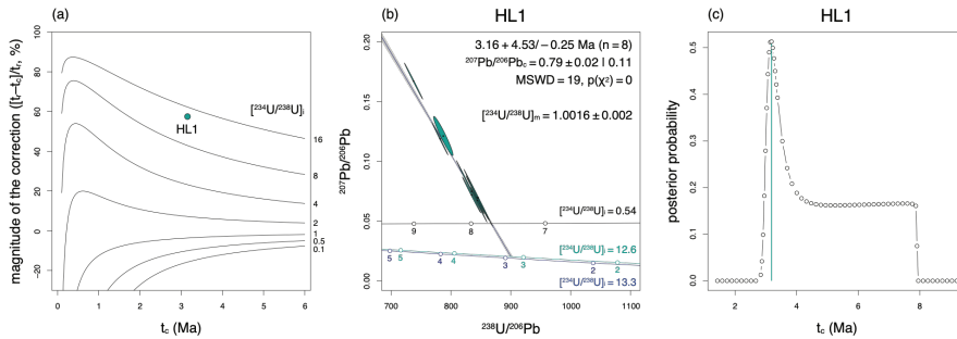
Figure 1: ^{234}\text{U} disequilibrium correction in young carbonates. (a) Nomogram of the relative magnitude of the correction vs. corrected date for different values of [^{234}\text{U}/^{238}\text{U}]_i ; t_c is the uncorrected date, assuming secular equilibrium, t_c is the corrected date. (b) Disequilibrium-corrected U-Pb data of Hoogland sample HL1 from Pickering et al. (2019), using a measured present-day ^{234}\text{U}/^{238}\text{U} activity ratio [^{234}\text{U}/^{238}\text{U}]_m = 1.0016 with nominal 1‰ uncertainty ( 1\sigma ); three concordia lines are shown, for the maximum likelihood solution ( t_c = 3.16 Ma, corresponding to an inferred initial activity ratio [^{234}\text{U}/^{238}\text{U}]_i = 12.6 ), the lower age limit ( t_l = 2.91 Ma with [^{234}\text{U}/^{238}\text{U}]_i = 13.3 ) and upper age limit ( t_u = 7.69 Ma with [^{234}\text{U}/^{238}\text{U}]_i = 0.54 ), respectively. (c) Posterior distribution of the corrected date, using a uniform prior for [^{234}\text{U}/^{238}\text{U}]_i from 0 to 20; t_l and t_u correspond to the 2.5 and 97.5 percentiles of this distribution respectively; t_c is marked by a vertical line.
