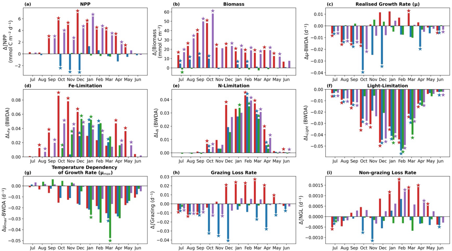
Figure 6. Simulated changes ( \Delta ) in phytoplankton class specific and total mean climatological terms determined from the mean climatological difference between high and low integrated total NPP seasons for: (a) depth integrated \Delta\text{NPP} , (b) depth integrated \Delta\text{Biomass} , (c) biomass-weighted depth-averaged growth rate \Delta\mu , (d) biomass-weighted depth-averaged iron limitation, \Delta L_{\text{Fe}} (positive \Delta L_{\text{Fe}} indicates reduced iron limitation), (e) biomass-weighted depth-averaged nitrogen limitation \Delta L_{\text{N}} (positive \Delta L_{\text{N}} indicates reduced nitrate limitation), (f) biomass-weighted depth-averaged light limitation \Delta L_{\text{Light}} (negative \Delta L_{\text{Light}} indicates increased light limitation), (g) biomass-weighted depth-averaged growth rate temperature dependency \mu_{\text{max}} , (h) phytoplankton biomass normalized specific grazing loss rate \Delta\text{Grazing} , and (i) phytoplankton biomass normalized specific non-grazing loss rate \Delta\text{NGL} . Stars denote that mean monthly climatological difference in the selected high and low NPP season groups is significantly exceeds the full time series climatological variability at the p < 0.05 level (10,000 iteration random year group bootstrapping analysis).
