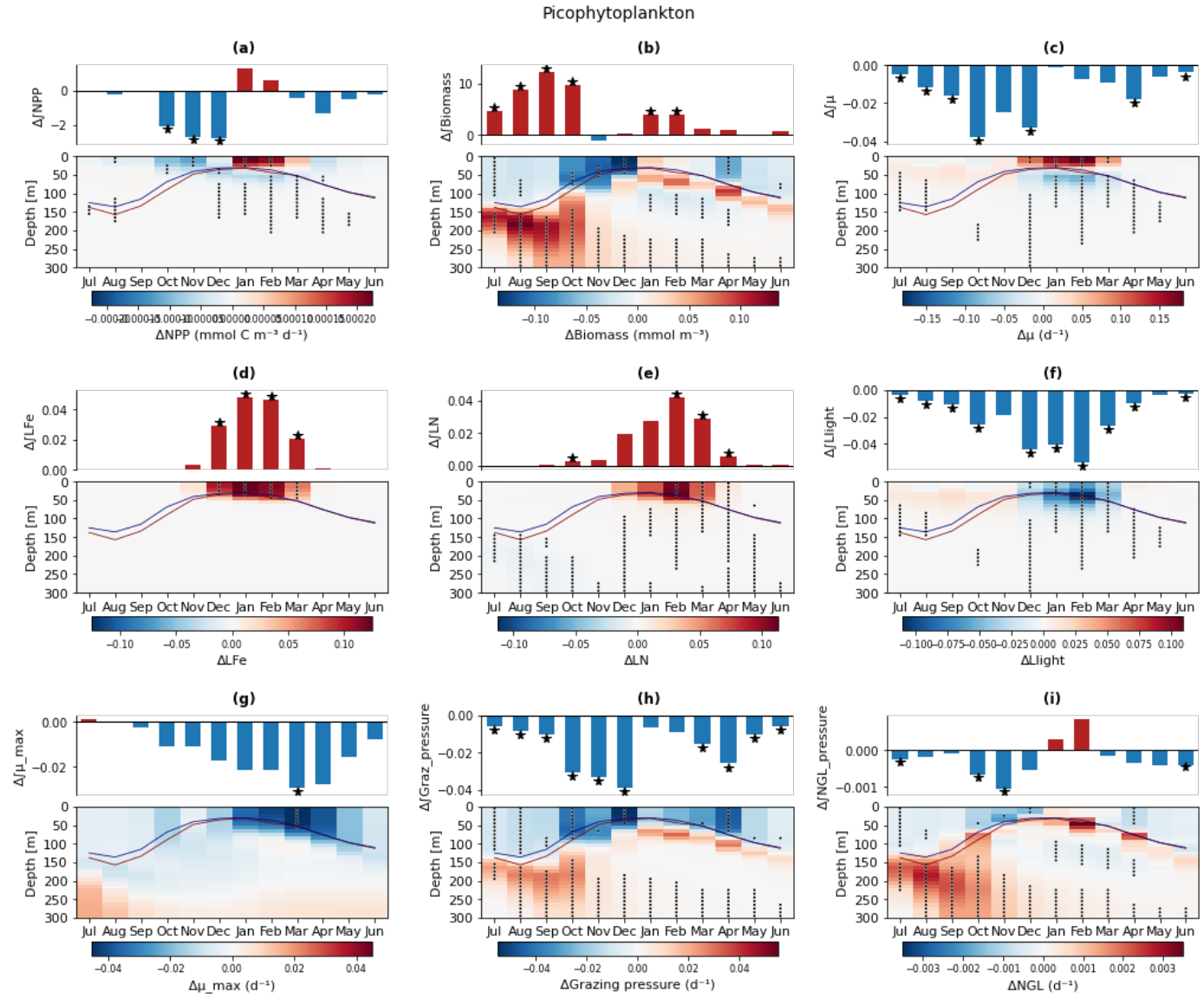
Figure A4. Simulated picophytoplankton class specific integrated (bar plots) and depth resolved (interpolated onto a 10 m regular grid) mean climatological a) \Delta\text{NPP} b) \Delta\text{Biomass} , c) biomass-weighted depth-averaged growth rate \Delta\mu , d) biomass-weighted depth-averaged iron limitation, \Delta L_{\text{Fe}} , e) biomass-weighted depth-averaged nitrogen limitation \Delta L_{\text{N}} , f) biomass-weighted depth-averaged light limitation \Delta L_{\text{light}} , g) Biomass-weighted depth-averaged growth rate temperature dependency \mu_{\text{max}} , h) phytoplankton biomass normalized specific grazing loss rate, \Delta\text{Grazing} , i) phytoplankton biomass normalized specific non-grazing loss rate, \Delta\text{NGL} . \Delta terms were determined from the mean climatological difference between high and low integrated total NPP seasons. Stars denote that mean monthly climatological difference in the selected high and low picophytoplankton NPP season groups significantly exceeds the full time series climatological variability at the p < 0.05 level (10,000 iteration random year bootstrapping analysis).
