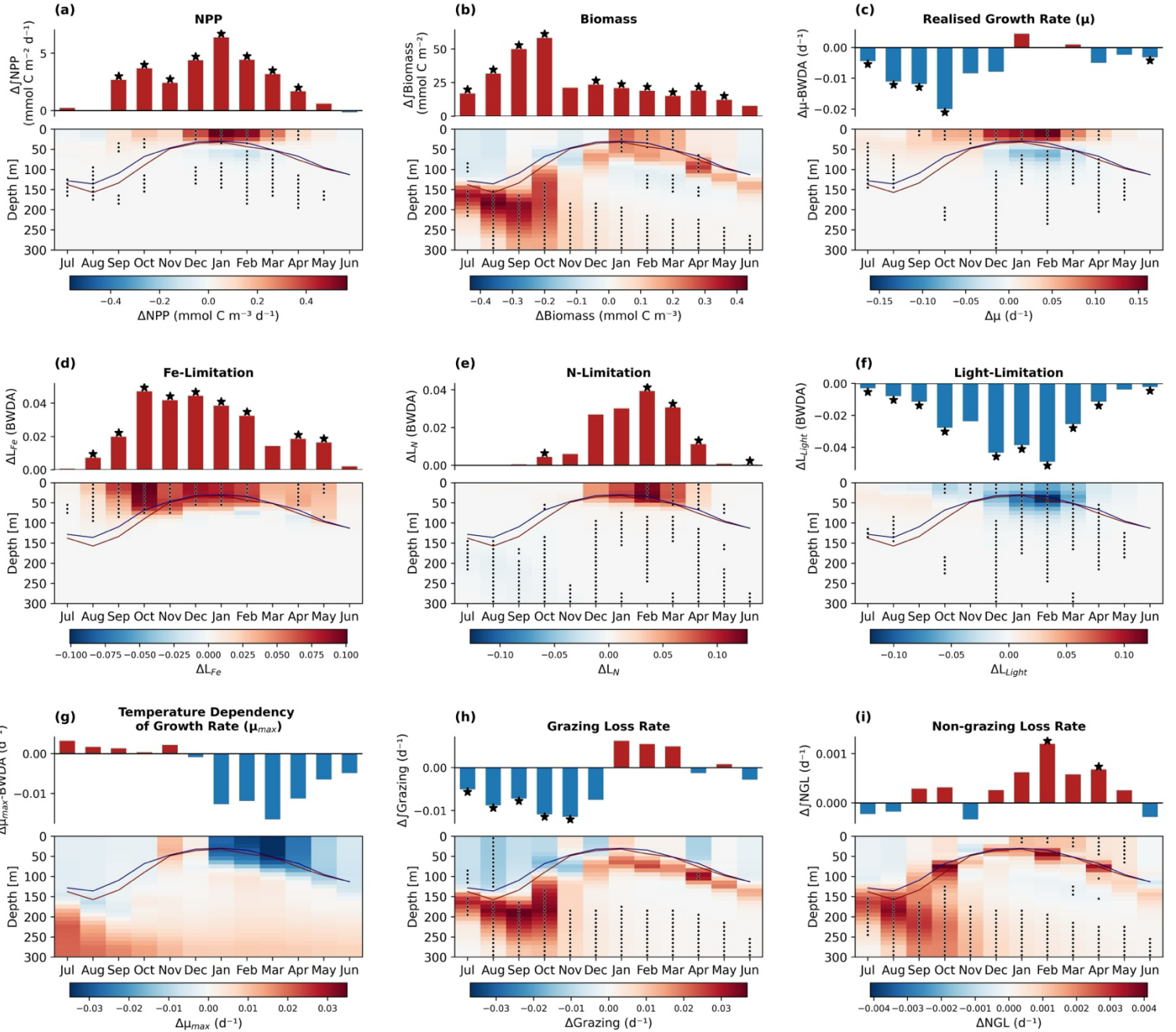
Figure 7. Simulated integrated (bar plots) and depth resolved (interpolated onto a 10 m regular grid) mean climatological (a) \Delta \text{NPP} , (b) \Delta \text{Biomass} , (c) biomass-weighted depth-averaged growth rate \Delta \mu , (d) biomass-weighted depth-averaged iron limitation, \Delta L_{\text{Fe}} , (e) biomass-weighted depth-averaged nitrogen limitation \Delta L_{\text{N}} , (f) biomass-weighted depth-averaged light limitation \Delta L_{\text{light}} , (g) Biomass-weighted depth-averaged growth rate temperature dependency \mu_{\text{max}} , (h) phytoplankton biomass normalized specific grazing loss rate \Delta \text{Grazing} , and (i) phytoplankton biomass normalized specific non-grazing loss rate \Delta \text{NGL} . \Delta terms were determined from the mean climatological difference between high and low integrated total NPP seasons. Stars and stippling denote that mean monthly climatological difference in the selected high and low NPP season groups significantly exceeds the full time series climatological variability at the p < 0.05 level (10,000 iteration random year bootstrapping analysis). Red and blue solid lines denote mean MLDs in respective high and low NPP year groups.
