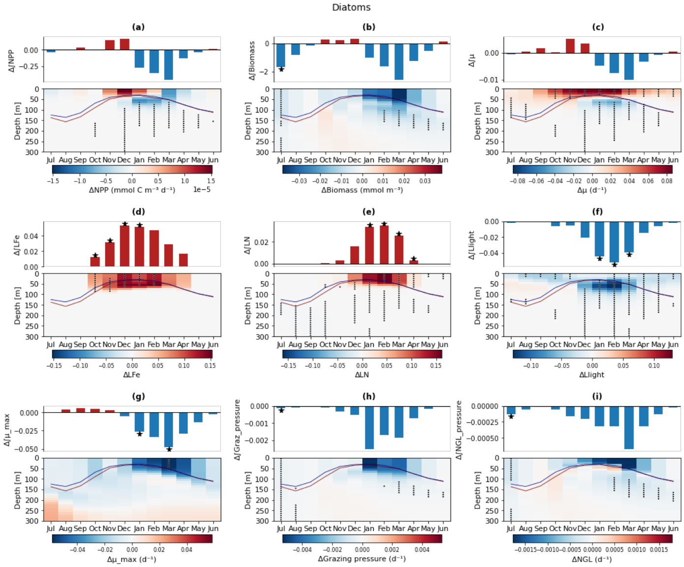
Figure A5. Simulated diatom class specific integrated (bar plots) and depth resolved (interpolated onto a 10 m regular grid) mean climatological a) \Delta NPP b) \Delta Biomass , c) biomass-weighted depth-averaged growth rate \Delta \mu , d) biomass-weighted depth-averaged iron limitation, \Delta L_{Fe} , e) biomass-weighted depth-averaged nitrogen limitation \Delta L_N , f) biomass-weighted depth-averaged light limitation \Delta L_{light} , g) Biomass-weighted depth-averaged growth rate temperature dependency \mu_{max} , h) phytoplankton biomass normalized specific grazing loss rate, \Delta Grazing , i) phytoplankton biomass normalized specific non-grazing loss rate, \Delta NGL . \Delta terms were determined from the mean climatological difference between high and low integrated total NPP seasons. Stars denote that mean monthly climatological difference in the selected high and low diatom NPP season groups significantly exceeds the full time series climatological variability at the p < 0.05 level (10,000 iteration random year bootstrapping analysis).
