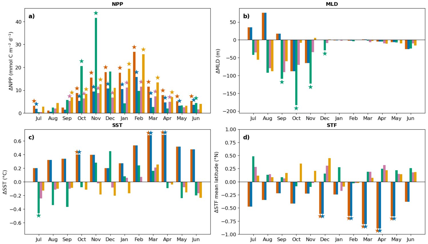
NPP (OC-CCI) Remote Sensing Algorithm
