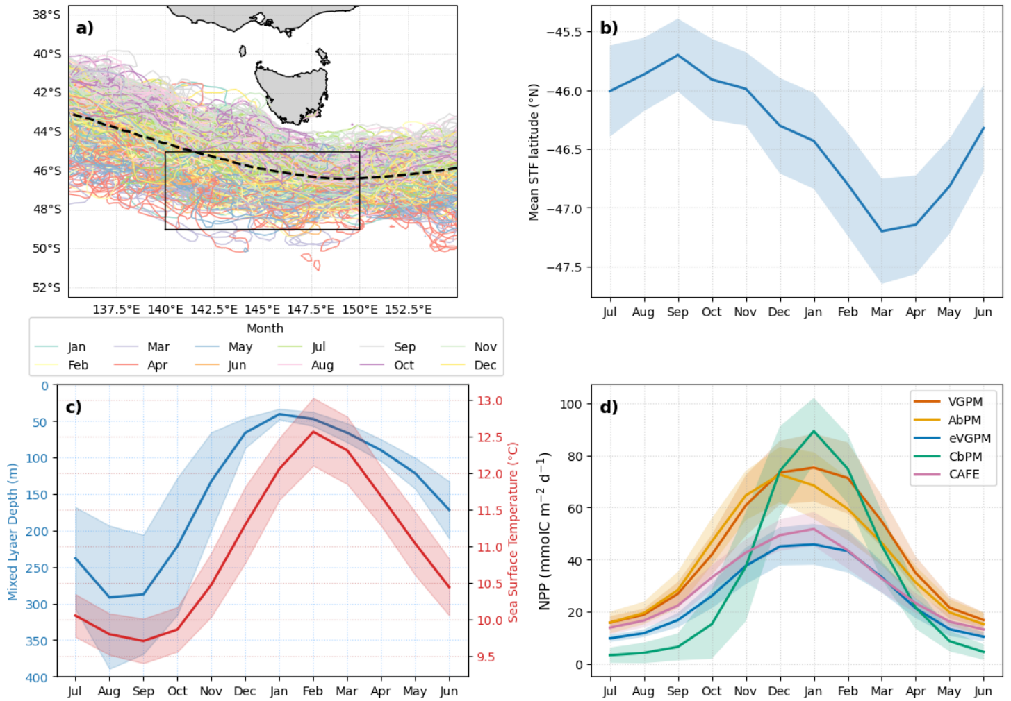
105 Figure 1. (a) Regional bounding box (solid black line) in which observational and modelled climatological averages were calculated. Mean monthly contours of the subtropical front (STF; 11-degree isotherm at 100 m depth, definition per Orsi et al. 1995) for the period 1998–2022 are given by coloured lines, with the mean given by the dashed black line. (b) climatological STF extent (1998–2022) as the mean latitude (°N) ( \pm 1\sigma from the mean) of the
