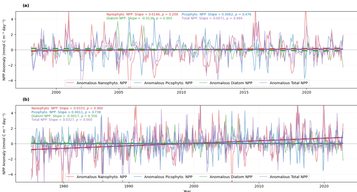
525 Figure 10. (a) PISCES-Quota-Fe simulated class specific NPP monthly anomalies (thin lines), fitted with ordinary least squares trend regressions for the period 1998-2022 corresponding to the remote sensing record. (b) Extended NPP trend analysis over the full study simulation time series 1975-2022.
