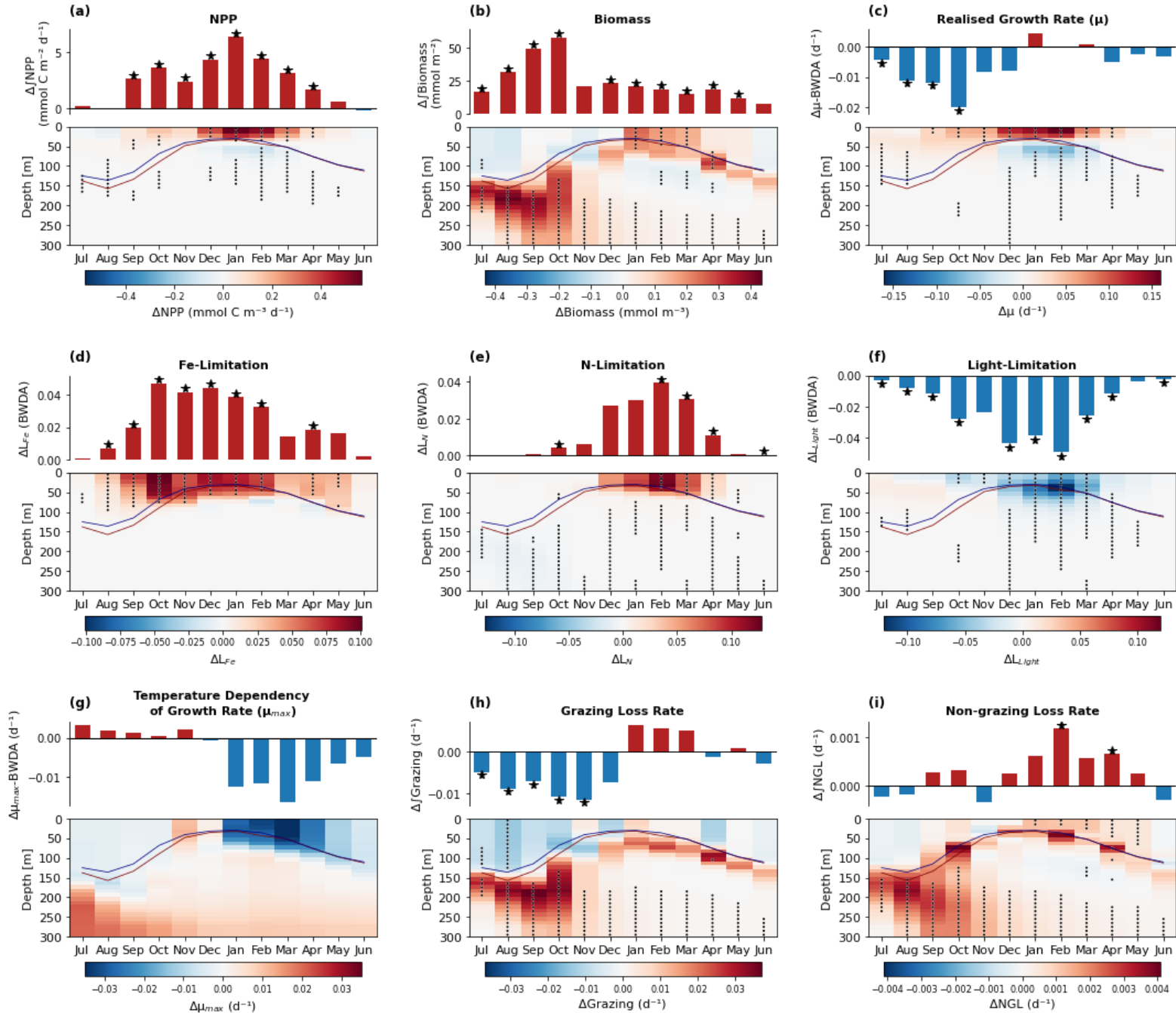
Figure 7. Simulated integrated (barplots) and depth resolved (interpolated onto a 10 m regular grid) mean climatological (a) \Delta\text{NPP} , (b) \Delta\text{Biomass} , (c) biomass-weighted depth-averaged growth rate \Delta\mu , (d) biomass-weighted depth-averaged iron limitation, \Delta L_{\text{Fe}} , (e) biomass-weighted depth-averaged nitrogen limitation \Delta L_{\text{N}} , (f) biomass-weighted depth-averaged light limitation \Delta L_{\text{light}} , (g) Biomass-weighted depth-averaged growth rate temperature dependency \mu_{\text{max}} , (h) phytoplankton biomass normalized specific grazing loss rate \Delta\text{Grazing} , and (i) phytoplankton biomass normalized specific non-grazing loss rate \Delta\text{NGL} . \Delta terms were determined from the mean climatological difference between high and low integrated total NPP seasons. Stars and stippling denote that mean monthly climatological difference in the selected high and low NPP season groups significantly exceeds the full time series climatological variability at the p < 0.05 level (10,000 iteration random year bootstrapping analysis). Red and blue solid lines denote mean MLDs in respective high and low NPP year groups.
