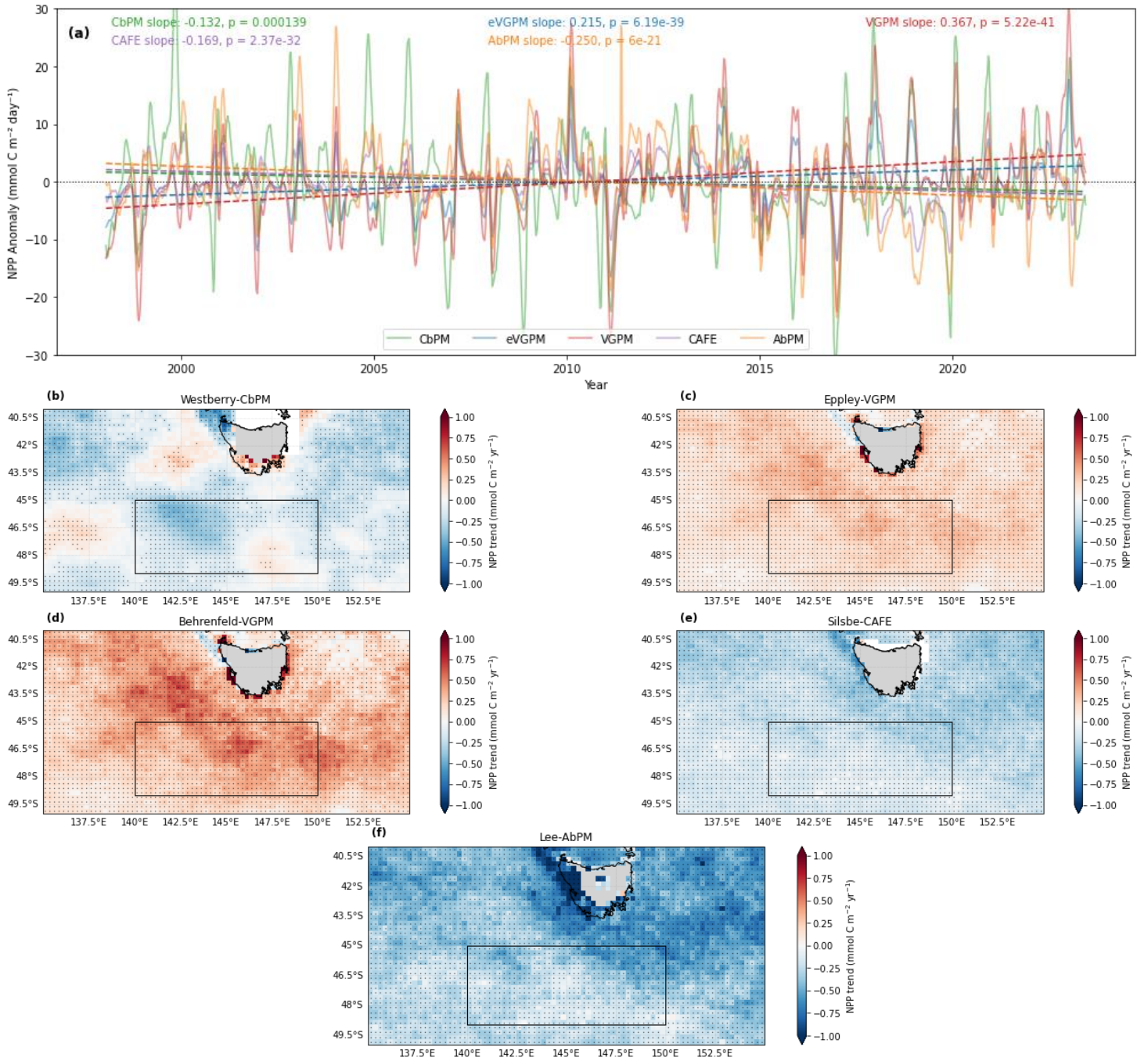
Figure 9. (a) Timeseries (1998 – 2022) of monthly NPP anomalies from the five remote sensing NPP algorithms, spatially averaged over the SOTS region (45–49S, 140–150E). Trends were determined from ordinary least squares regression of the monthly anomalies, with trend slope and p-values for significance given. . (b – e) Spatial trends computed from ordinary least squares regressions on monthly single pixel NPP anomalies for each remote sensing NPP algorithm in (a) . Stippling in pixels indicates significant trends at the p < 0.05 level. The black box denotes study region used for averaging in (a) .
