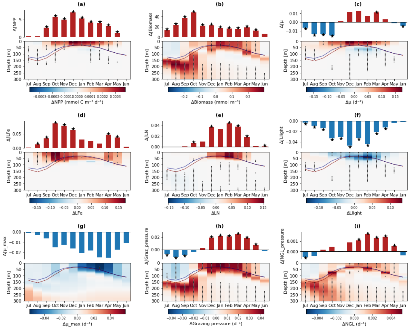
Figure A3. Simulated nanophytoplankton class specific integrated (barplots) and depth resolved (interpolated onto a 10 m regular grid) mean climatological a) \Delta NPP b) \Delta Biomass , c) biomass-weighted depth-averaged growth rate \Delta \mu , d) biomass-weighted depth-averaged iron limitation, \Delta L_{Fe} , e) biomass-weighted depth-averaged nitrogen limitation \Delta L_N , f) biomass-weighted depth-averaged light limitation \Delta L_{light} , g) Biomass-weighted depth-averaged growth rate temperature dependency \mu_{max} , h) phytoplankton biomass normalized specific grazing loss rate, \Delta Grazing , i) phytoplankton biomass normalized specific non-grazing loss rate, \Delta NGL . \Delta terms were determined from the mean climatological difference between high and low integrated total NPP seasons. Stars denote that mean monthly climatological difference in the selected high and low NPP season groups significantly exceeds the full time series climatological variability at the p < 0.05 level (10,000 iteration random year bootstrapping analysis).
