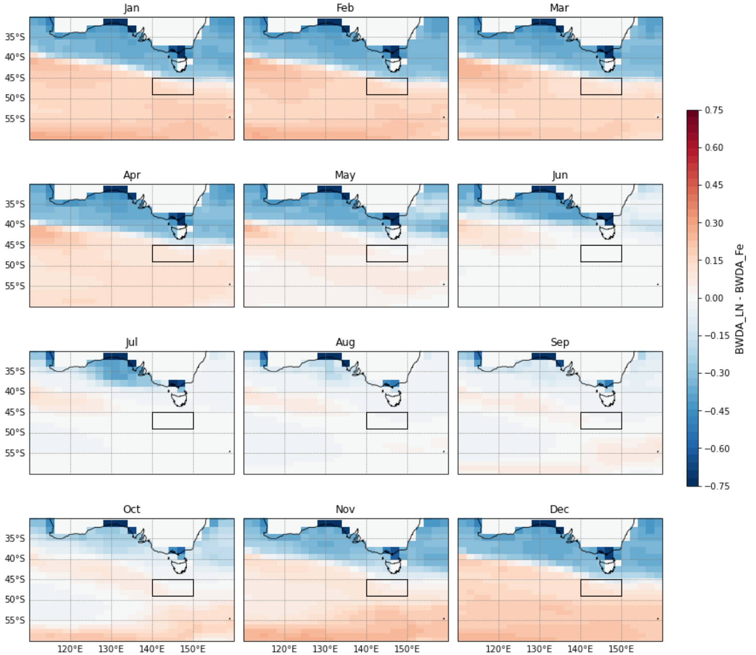
Figure A1. Simulated PISCES-Quota-Fe climatological biomass-weighted depth-averaged difference between L_N and L_{Fe} limitation terms for the period 1975-2022. Red shading denotes L_{Fe} dominance ( L_{Fe} < L_N ), and blue shading denotes L_N dominance ( L_{Fe} > L_N ), defining the nutrient limitation state of phytoplankton classes. Black box denotes study region used to calculate spatial means.
