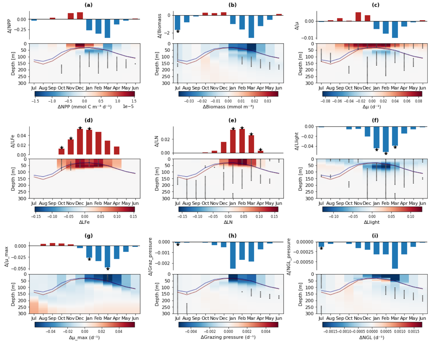
Figure A5. Simulated diatom class specific integrated (barplots) and depth resolved (interpolated onto a 10 m regular grid) mean climatological a) \Delta NPP b) \Delta Biomass , c) biomass-weighted depth-averaged growth rate \Delta \mu , d) biomass-weighted depth-averaged iron limitation, \Delta L_{Fe} , e) biomass-weighted depth-averaged nitrogen limitation \Delta L_N , f) biomass-weighted depth-averaged light limitation \Delta L_{light} , g) Biomass-weighted depth-averaged growth rate temperature dependency \mu_{max} , h) phytoplankton biomass normalized specific grazing loss rate, \Delta Grazing , i) phytoplankton biomass normalized specific non-grazing loss rate, \Delta NGL . \Delta terms were determined from the mean climatological difference between high and low integrated total NPP seasons. Stars denote that mean monthly climatological difference in the selected high and low diatom NPP season groups significantly exceeds the full time series climatological variability at the p < 0.05 level (10,000 iteration random year bootstrapping analysis).
