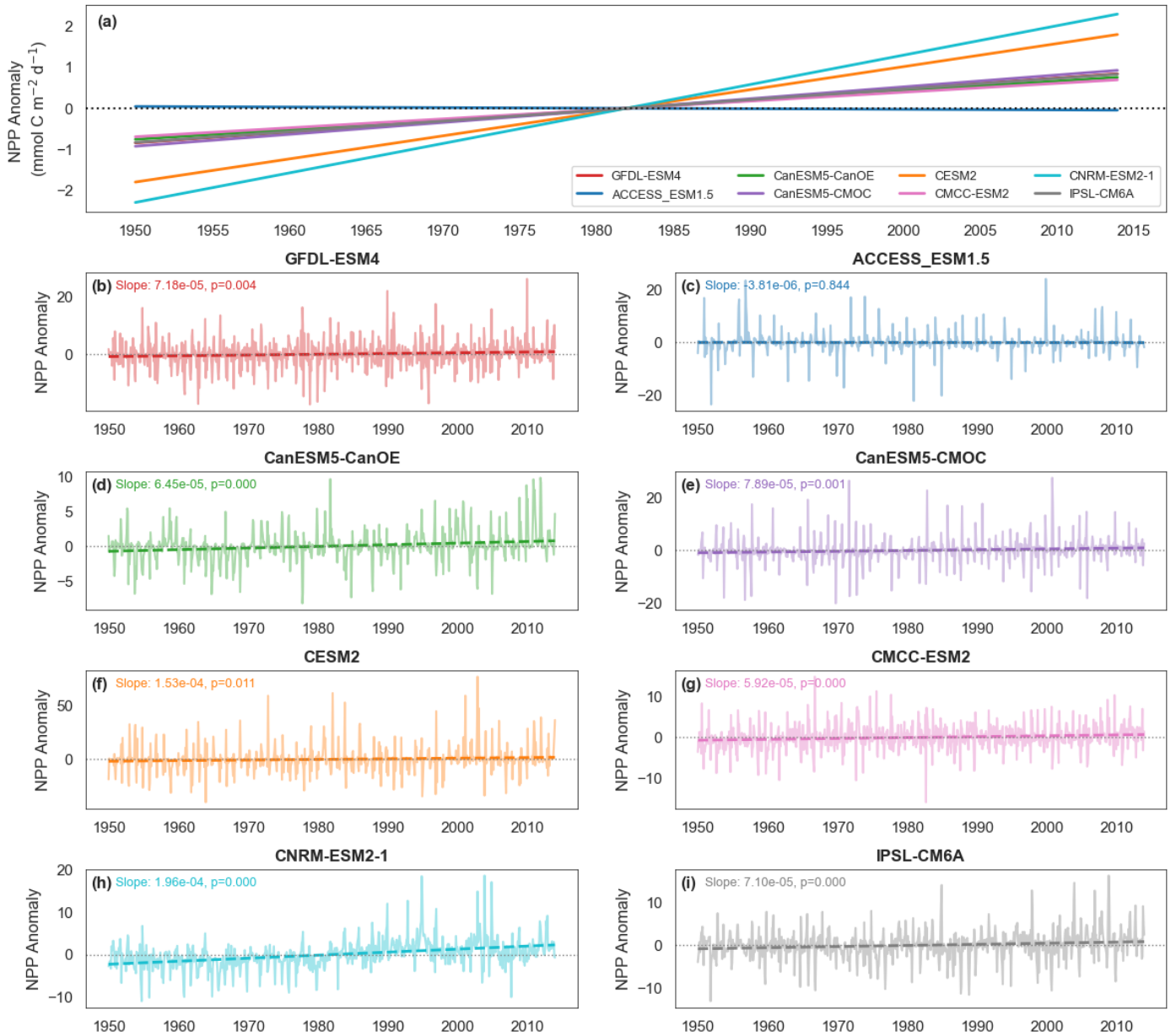
Figure A8. (a) Trends in monthly anomalous NPP time series from the 8 CMIP6 historical models listed in Table 2, (b – i) Individual CMIP6 model time series of spatial mean monthly NPP anomalies. Linear trends were calculated using ordinary least squares regression, with slope and p-values given for trends significantly different from zero (climate modes were not subtracted).
