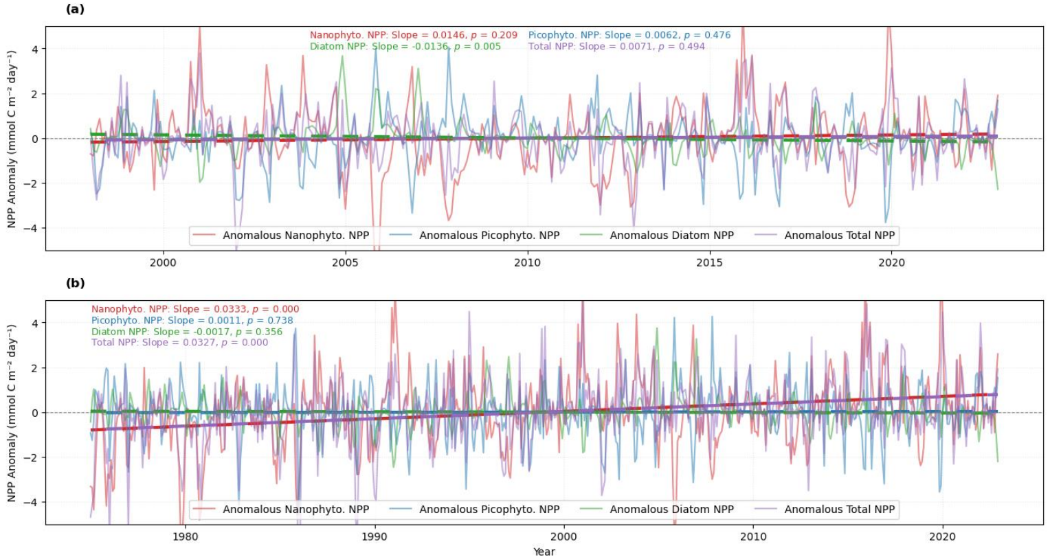
Figure 10. (a) PISCES-Quota-Fe simulated class specific NPP monthly anomalies (thin lines), fitted with ordinary least squares trend regressions for the period 1998-2022 corresponding to the remote sensing record. (b) Extended NPP trend analysis over the full study simulation time series 1975-2022.
