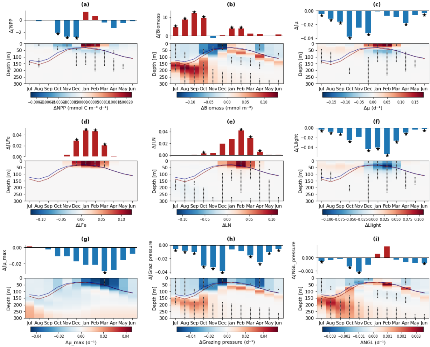
Figure A4. Simulated picophytoplankton class specific integrated (barplots) and depth resolved (interpolated onto a 10 m regular grid) mean climatological a) \Delta NPP b) \Delta Biomass , c) biomass-weighted depth-averaged growth rate \Delta \mu , d) biomass-weighted depth-averaged iron limitation, \Delta L_{Fe} , e) biomass-weighted depth-averaged nitrogen limitation \Delta L_N , f) biomass-weighted depth-averaged light limitation \Delta L_{light} , g) Biomass-weighted depth-averaged growth rate temperature dependency \mu_{max} , h) phytoplankton biomass normalized specific grazing loss rate, \Delta Grazing , i) phytoplankton biomass normalized specific non-grazing loss rate, \Delta NGL . \Delta terms were determined from the mean climatological difference between high and low integrated total NPP seasons. Stars denote that mean monthly climatological difference in the selected high and low picophytoplankton NPP season groups significantly exceeds the full time series climatological variability at the p < 0.05 level (10,000 iteration random year bootstrapping analysis).
