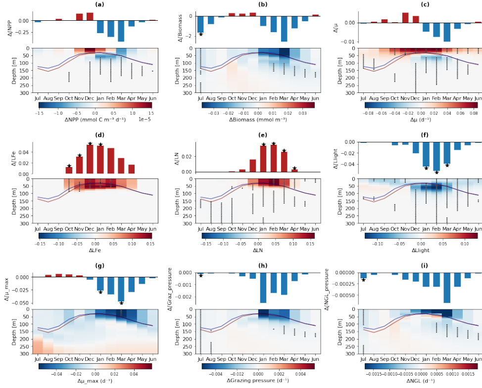
Figure A5. Simulated diatom class specific integrated (barplots) and depth resolved (interpolated onto a 10 m regular grid) mean climatological a) \Delta\text{NPP} b) \Delta\text{Biomass} , c) biomass-weighted depth-averaged growth rate \Delta\mu , d) biomass-weighted depth-averaged iron limitation, \Delta L_{\text{Fe}} , e) biomass-weighted depth-averaged nitrogen limitation \Delta L_{\text{N}} , f) biomass-weighted depth-averaged light limitation \Delta L_{\text{light}} , g) Biomass-weighted depth-averaged growth rate temperature dependency \mu_{\text{max}} , h) phytoplankton biomass normalized specific grazing loss rate, \Delta\text{Grazing} , i) phytoplankton biomass normalized specific non-grazing loss rate, \Delta\text{NGL} . \Delta terms were determined from the mean climatological difference between high and low integrated total NPP seasons. Stars denote that mean monthly climatological difference in the selected high and low diatom NPP season groups significantly exceeds the full time series climatological variability at the p < 0.05 level (10,000 iteration random year bootstrapping analysis).
