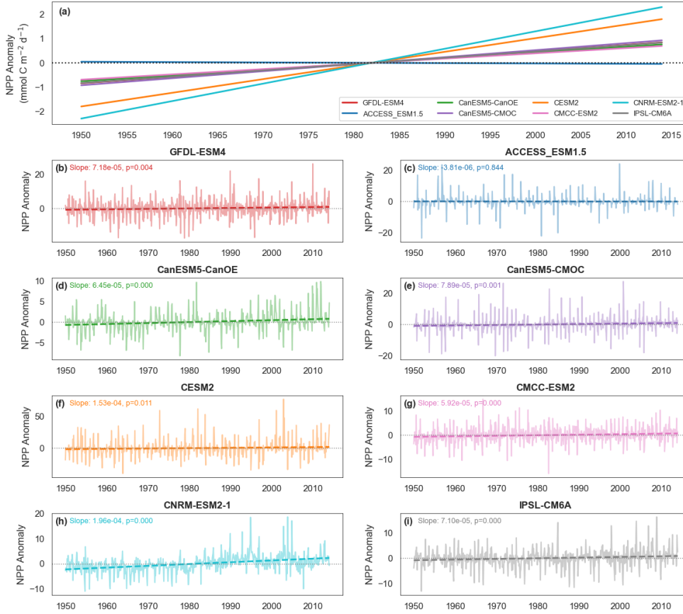
Figure A8. (a) Trends in monthly anomalous NPP time series from the 8 CMIP6 historical models listed in Table 2. (b – i) Individual CMIP6 model time series of spatial mean monthly NPP anomalies. Linear trends were calculated using ordinary least squares regression, with slope and p-values given for trends significantly different from zero (climate modes were not subtracted).
