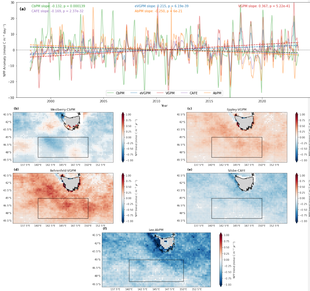
Figure 9. (a) Timeseries (1998 – 2022) of monthly NPP anomalies from the five remote sensing NPP algorithms, spatially averaged over the SOTS region (45–49S, 140–150E). Trends were determined from ordinary least squares regression of the monthly anomalies, with trend slope and p-values for significance given. (b – e) Spatial trends computed from ordinary least squares regressions on monthly single pixel NPP anomalies for each remote sensing NPP algorithm in (a). Stippling in pixels indicates significant trends at the p < 0.05 level. The black box denotes study region used for averaging in (a).
