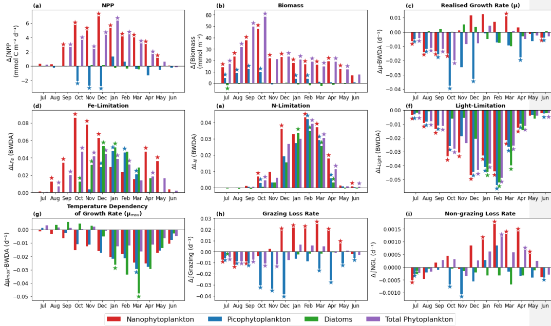
Figure 6. Simulated changes ( \Delta ) in phytoplankton class specific and total mean climatological terms determined from the mean climatological difference between high and low integrated total NPP seasons for: (a) depth integrated \Delta NPP, (b) depth integrated \Delta Biomass, (c) biomass-weighted depth-averaged growth rate \Delta\mu , (d) biomass-weighted depth-averaged iron limitation, \Delta L_{Fe} , (positive \Delta L_{Fe} indicates reduced iron limitation), (e) biomass-weighted depth-averaged nitrogen limitation \Delta L_N (positive \Delta L_N indicates reduced nitrate limitation), (f) biomass-weighted depth-averaged light limitation \Delta L_{light} (negative \Delta L_{light} indicates increased light limitation), (g) biomass-weighted depth-averaged growth rate temperature dependency \mu_{max} , (h) phytoplankton biomass normalized specific grazing loss rate \Delta Grazing, and (i) phytoplankton biomass normalized specific non-grazing loss rate \Delta NGL. Stars denote that mean monthly climatological difference in the selected high and low NPP season groups is significantly exceeds the full time series climatological variability at the p < 0.05 level (10,000 iteration random year group bootstrapping analysis).
