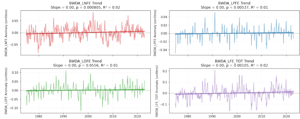
765 Figure A7. Trends in PISCES-Quota-Fe phytoplankton class specific biomass-weighted, depth-averaged (BWDA) iron limitation terms (positive values indicate decreasing iron limitation).
