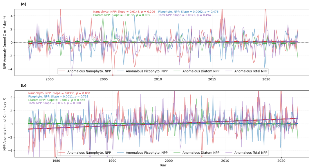
Figure 10. (a) PISCES-Quota-Fe simulated class specific NPP monthly anomalies (thin lines), fitted with ordinary least squares trend regressions for the period 1998-2022 corresponding to the remote sensing record. (b) Extended NPP trend analysis over the full study simulation time series 1975-2022.
