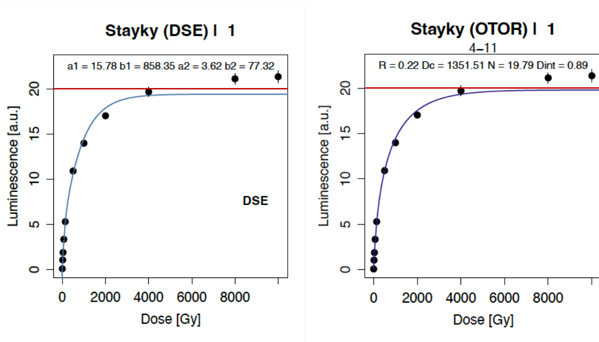
Supplement Figure to RC3. The SAR-derived data of sample Stayky 4-11 (quartz) fitted using the DSE function (left) and the OTOR function (right). The red line is thought to guide the eyes.
