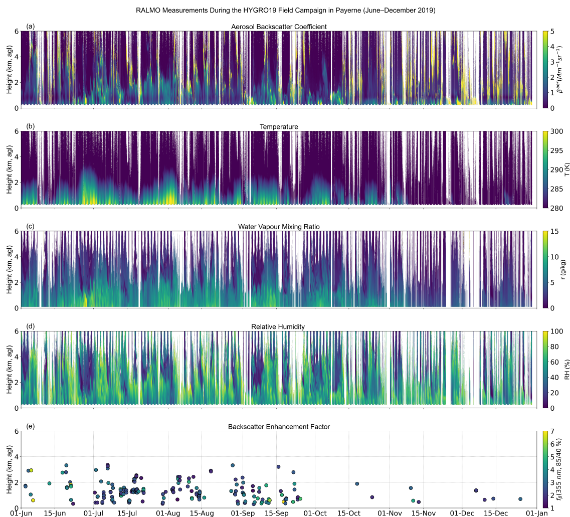
Figure 3. Temporal and vertical evolution of RALMO measurements during the HYGRO19 field campaign at the MeteoSwiss station in Payerne from June to December 2019. (a) Aerosol backscatter coefficient at 355 nm, (b) temperature, (c) water vapour mixing ratio, (d) relative humidity, and (e) backscatter enhancement factor at 355 nm and 85 % RH, normalised to 40 % RH.
