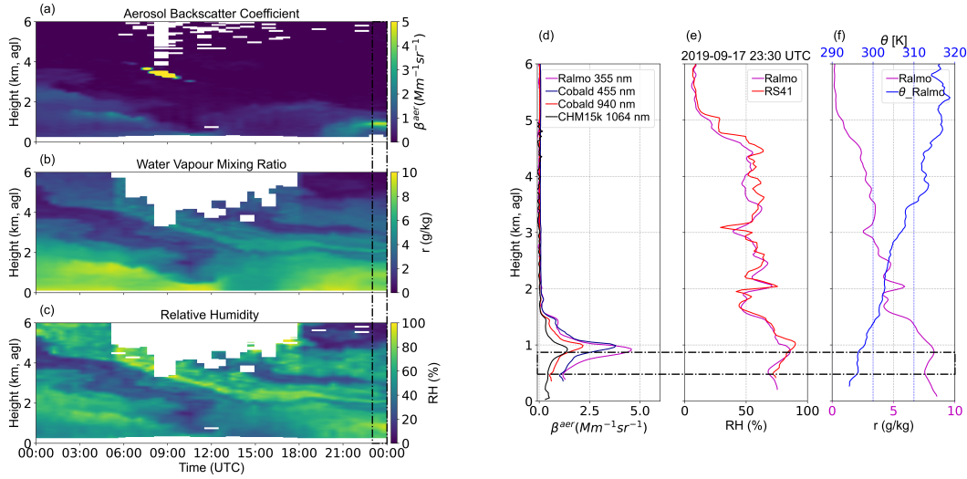
Figure 9. Temporal evolution of (a) \beta^{aer} (355 nm), (b) water vapour mixing ratio, and (c) RH profiles from RALMO on 17 September 2019. (d) \beta^{aer} profiles from RALMO at 355 nm (purple), COBALD at 455 and 940 nm (blue and red), and ceilometer at 1064 nm (black). (e) RH profiles from RALMO (purple) and RS41 (red). (f) Water vapour mixing ratio (purple) and potential temperature (blue) profiles from RALMO. The vertical profiles correspond to 23:30–23:59 UTC for RALMO and ceilometer, and 23:00–23:30 UTC for COBALD-RS41.
