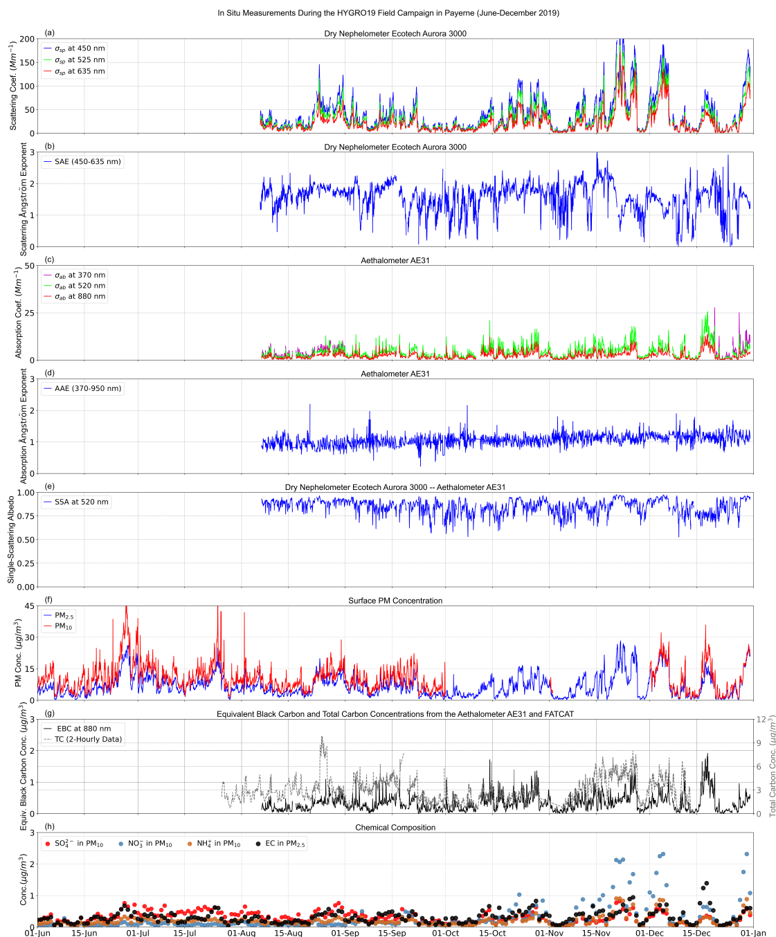
Figure 2. Time series of in situ ground-based measurements of (a) aerosol scattering coefficient at 450, 525, and 635 nm and (b) scattering Ångström exponent (SAE (450–635 nm)) from the Aurora 3000 dry nephelometer; (c) absorption coefficient at 370, 520, and 880 nm and (d) absorption Ångström exponent (AAE (370–950 nm)) from the aethalometer AE31; (e) single scattering albedo (SSA (520 nm)) derived from the dry nephelometer and aethalometer data, (f) PM concentrations, (g) equivalent black carbon at 880 nm from the aethalometer and total carbon concentrations from FATCAT; and (h) chemical composition. The data represent hourly mean values, except for TC concentrations and chemical compositions that are 2-hourly and daily measurements.
