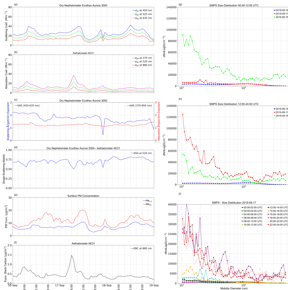
Figure A1. Time hourly series (left panels) over 16 to 18 September 2019 of: (a) aerosol scattering coefficient at 450, 525, and 635 nm from the Aurora 3000 dry nephelometer, (b) absorption coefficient at 370, 520 and 880 nm from the aethalometer AE31, (c) scattering (SAE (450–635 nm)) and absorption (AAE (370–950 nm)) Ångström exponents and (d) single scattering albedo (SSA) at 520 nm derived from the dry nephelometer and aethalometer, (e) PM concentrations, (f) equivalent black carbon at 880 nm from the aethalometer. Aerosol size distribution from the SMPS (right panels) for mean between (g) 00:00–12:00 UTC and (h) 12:00–24:00 UTC from 16 to 18 September 2019, and (i) 2 hourly mean on 17 September 2019.
