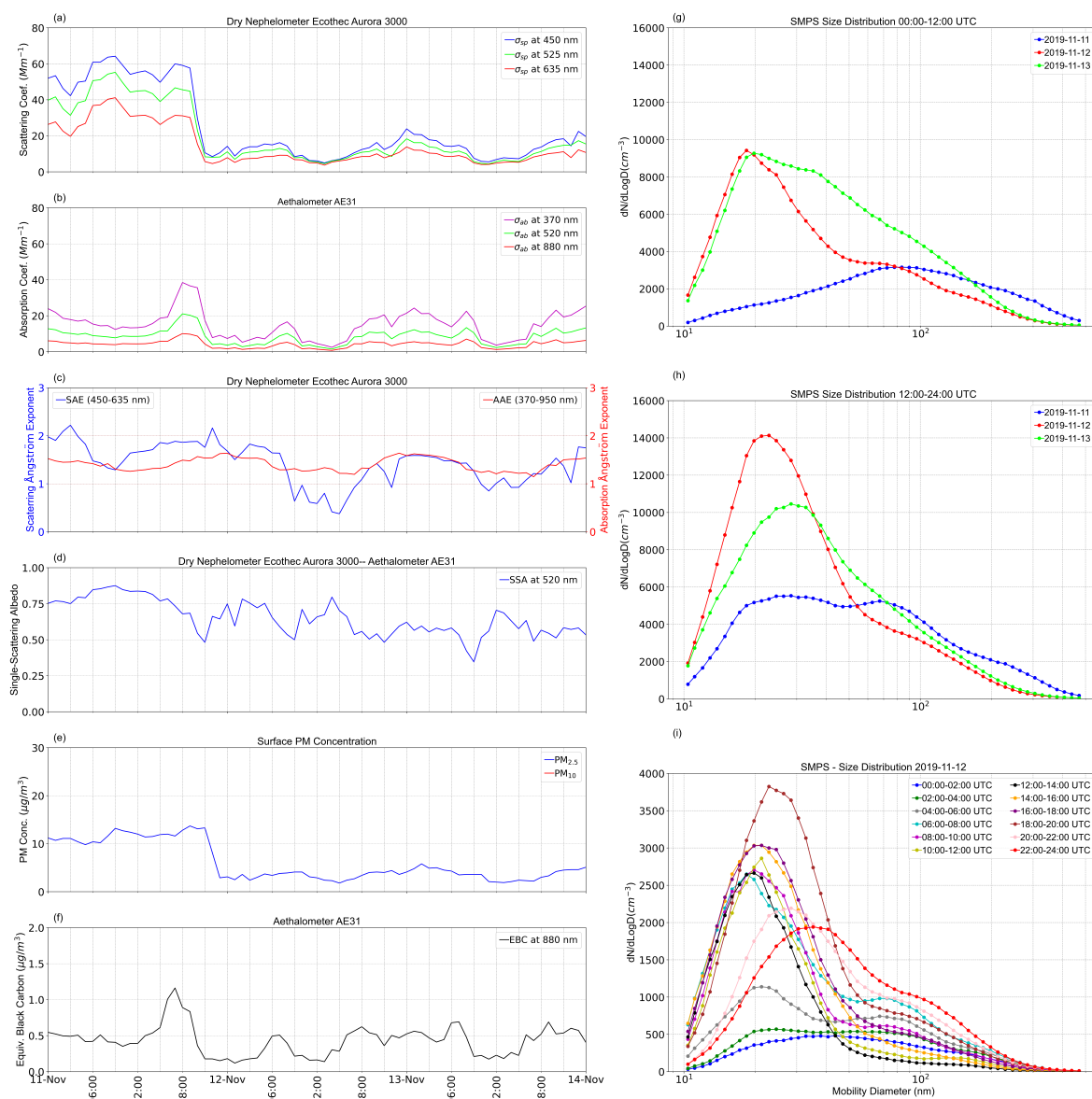
Figure A2. Time hourly series (left panels) over 11 to 13 November 2019 of: (a) aerosol scattering coefficient at 450, 525, and 635 nm from the Aurora 3000 dry nephelometer, (b) absorption coefficient at 370, 520 and 880 nm from the aethalometer AE31, (c) scattering (SAE (450–635 nm)) and absorption (AAE (370–950 nm)) Ångström exponents and (d) single scattering albedo (SSA) at 520 nm derived from the dry nephelometer and aethalometer, (e) PM concentrations, (f) equivalent black carbon at 880 nm from the aethalometer. Aerosol size distribution from the SMPS (right panels) for mean between (g) 00:00–12:00 UTC and (h) 12:00–24:00 UTC from 11 to 13 November 2019, and (i) 2 hourly mean on 12 November 2019.
