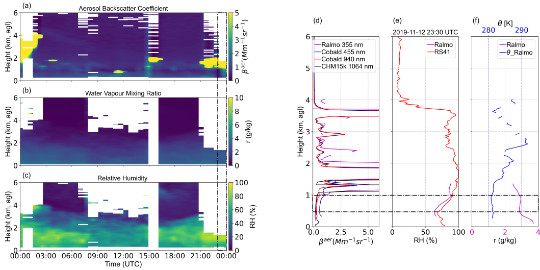
Figure 11. Temporal evolution of (a) \beta^{aer} (355 nm), (b) water vapour mixing ratio, and (c) RH profiles from RALMO on 12 November 2019. (d) \beta^{aer} profiles from RALMO at 355 nm (purple), COBALD at 455 and 940 nm (blue and red), and ceilometer at 1064 nm (black). (e) RH profiles from RALMO (purple) and RS41 (red). (f) Water vapour mixing ratio (purple) and potential temperature (blue) profiles from RALMO. The vertical profiles correspond to 23:30–23:59 UTC for RALMO and ceilometer, and 23:00–23:30 UTC for COBALD-RS41.
