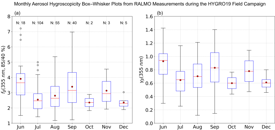
Figure 6. Box-whisker plots of (a) f_{\beta}(355 \text{ nm}, 85/40 \%) and (b) \gamma_{\beta}(355 \text{ nm}) from RALMO measurements for every month during the HYGRO19 field campaign. In each box plot, the central mark represents the median, the red point indicates the mean, and the box extends vertically from the 25th to the 75th percentiles. N represents the number of cases.
