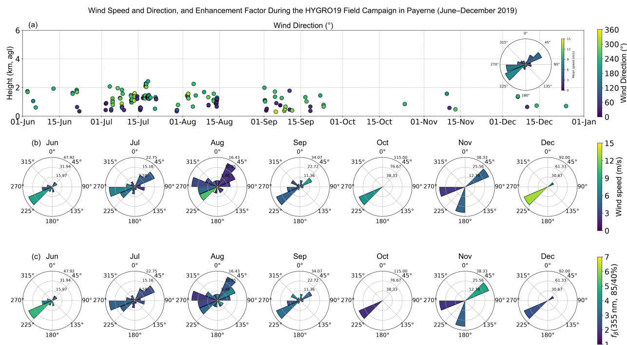
Figure 7. Temporal and vertical evolution of wind direction (a) for the hygroscopic aerosol layers from wind profiler measurements during the HYGRO19 field campaign (June–December 2019). The inset in panel (a) shows the wind rose. Monthly wind rose plots depicting wind speed (b) and the f_{\beta}(355 \text{ nm}, 85/40 \%) from RALMO measurements (c).
