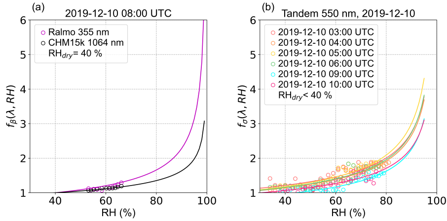
Figure 14. Enhancement factor ( f_c(\lambda, RH) ) retrieved from (a) RALMO and ceilometer within the 0.70–0.97 km agl layer, and from (b) tandem nephelometers at different times on 10 December 2019. The parameters are summarised in Table 7. Note that the humidograms in the left panel were normalised to dry conditions at 40 % RH, whereas the tandem measurements correspond to RH values below 40 %.
