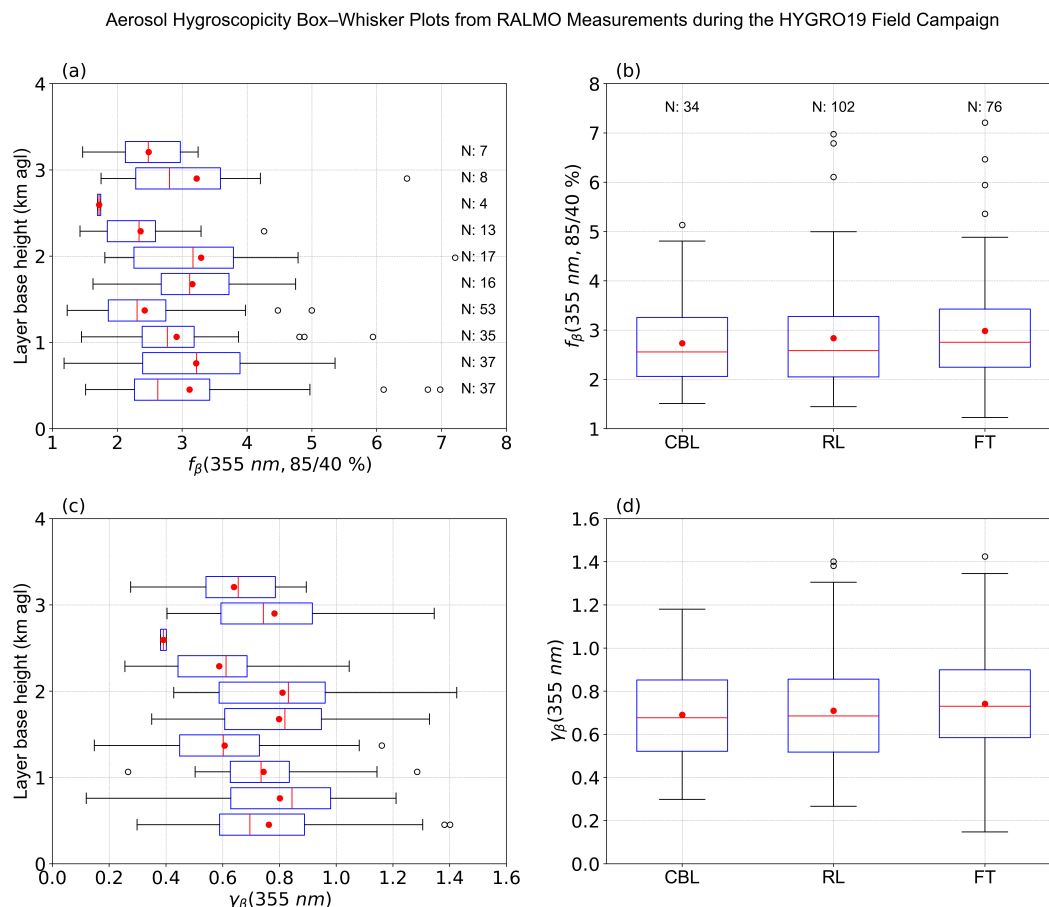
Figure 5. Box-whisker plots of (a) f_{\beta}(355 \text{ nm}, 85/40 \%) and (c) \gamma_{\beta}(355 \text{ nm}) by different height ranges. The analyses are also presented for the CBL, RL, and FT (b, d). In each box plot, the central mark represents the median, the red point indicates the mean, and the box extends vertically from the 25th to the 75th percentiles. N represents the number of cases.
