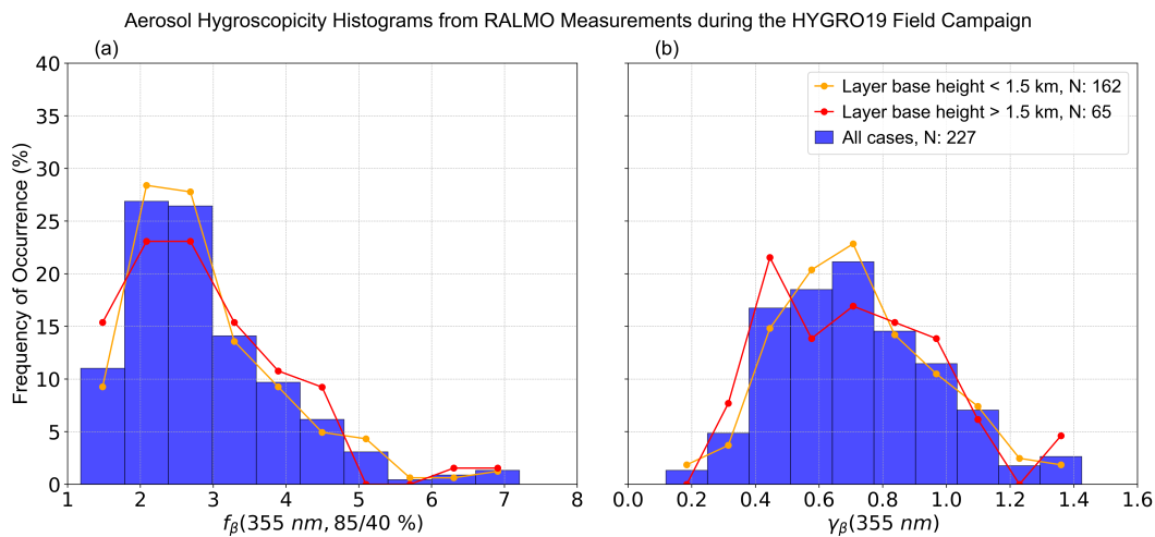
Figure 4. Frequency of occurrence of (a) f_{\beta}(355 \text{ nm}, 85/40 \%) and (b) \gamma_{\beta}(355 \text{ nm}) obtained from RALMO measurements during the HYGRO19 field campaign from June to December 2019. The analysis includes all detected aerosol hygroscopicity layers, as well as cases recorded below and above 1.5 km agl. N represents the number of cases.
