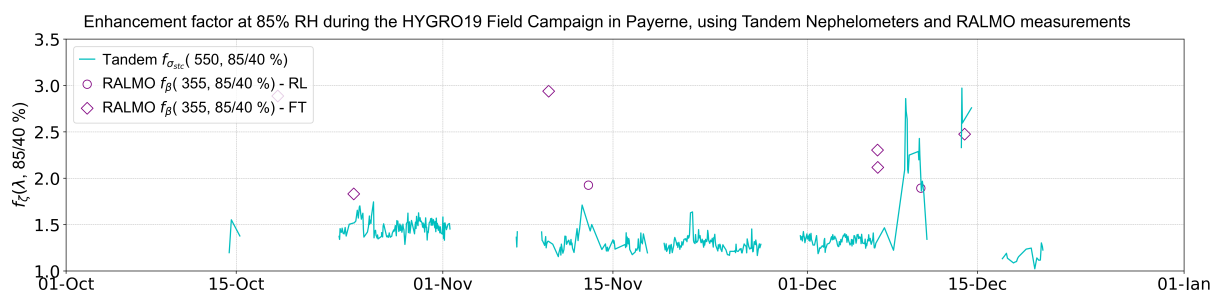
Figure 8. Temporal evolution of f_{\sigma}(550 \text{ nm}, 85 / < 40 \%) obtained using a tandem nephelometers during the HYGRO19 field campaign. The purple points and diamonds indicate f_{\beta}(355 \text{ nm}, 85 / 40 \%) from RALMO measurements in the RL and FT, respectively. Note that the values for RALMO were normalised to 40 % RH, whereas the tandem measurements correspond to RH values below 40%.
