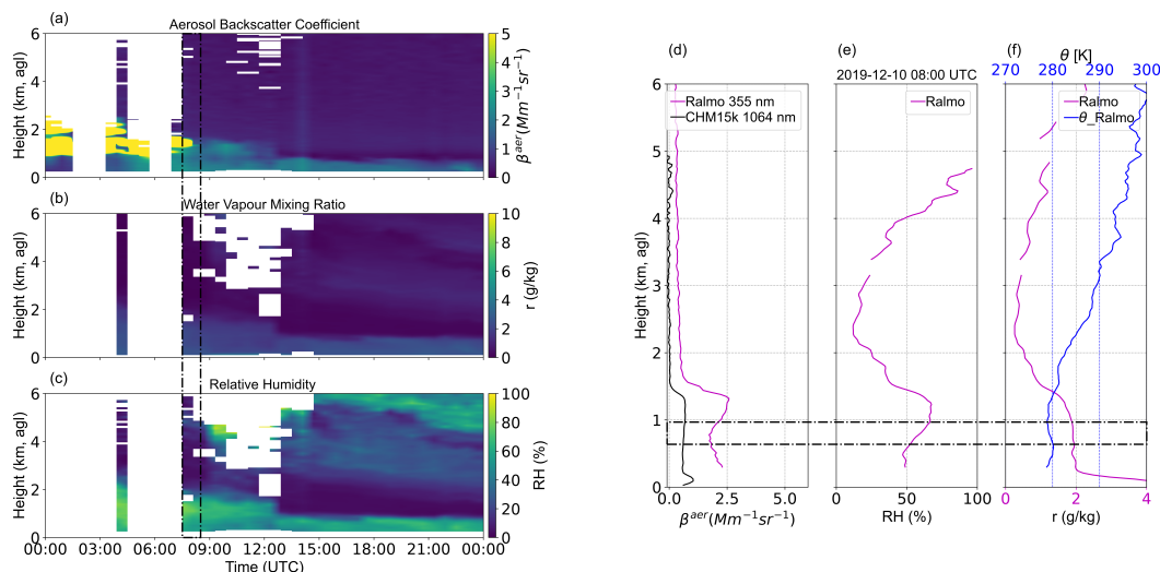
Figure 13. Temporal and vertical evolution of (a) \beta^{aer} (355 nm), (b) water vapour mixing ratio, and (c) RH from RALMO on 10 December 2019. (d) \beta^{aer} profiles from RALMO at 355 nm (purple), and ceilometer at 1064 nm (black). (e) RH, (f) Water vapour mixing ratio (purple) and potential temperature (blue) profiles from RALMO during the 08:00–08:30 UTC interval.
