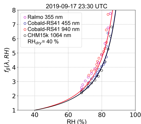
Figure 10. Enhancement factor ( f_{\beta}(\lambda, RH) ) retrieved from RALMO, COBALD-RS41 and ceilometer within the 0.48–0.87 km agl layer. The time interval corresponds to 23:30–23:59 UTC for RALMO and ceilometer, and 23:00–23:30 UTC for COBALD-RS41. The retrieved parameters are summarised in Table 7.
