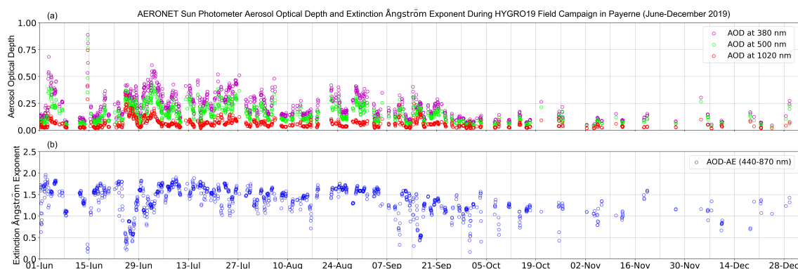
Figure 1. Hourly time series of AERONET observations during the HYGRO19 campaign from June–December 2019: (a) aerosol optical depth (AOD) at 380, 500, and 1020 nm, and (b) extinction Ångström exponent (AOD-AE (440–870 nm)).
