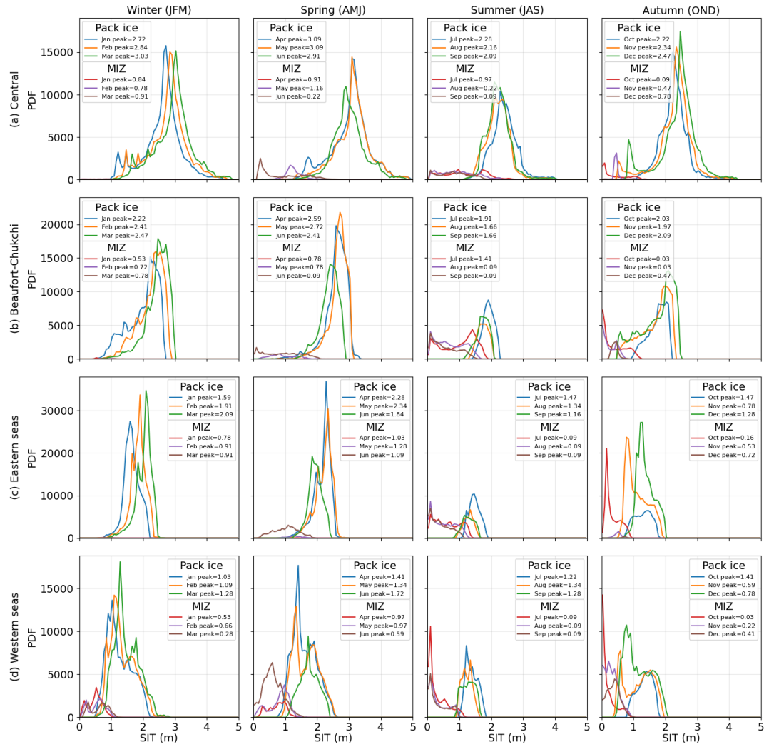
Figure S2. Probability density function (PDF) of pack and marginal ice SIT computed from GREP climatology in the period 1993–2020 for the selected sub-Arctic sectors.
