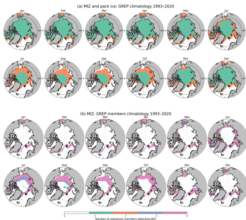
Figure S1. (a) Maps of pack (green) and marginal ice (orange) based on GREP monthly output data for 1993–2020. (b) Number of GREP members (0–4) detecting MIZ conditions at each grid cell on the same period.
