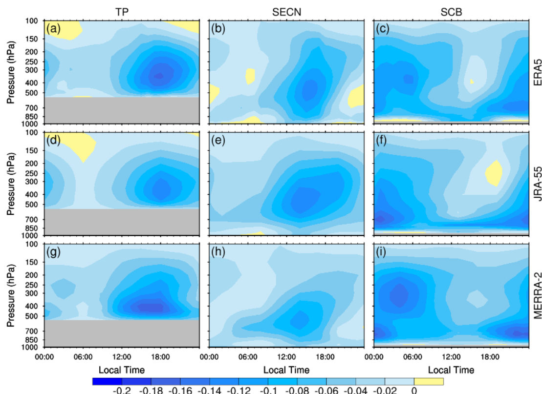
310 Figure 11. Diurnal variation of vertical velocity over TP (left), SECN (middle) and SCB (right) from ERA5 (top), JRA-55 (middle) and MERRA-2 (bottom). Units: \text{Pa s}^{-1} .
