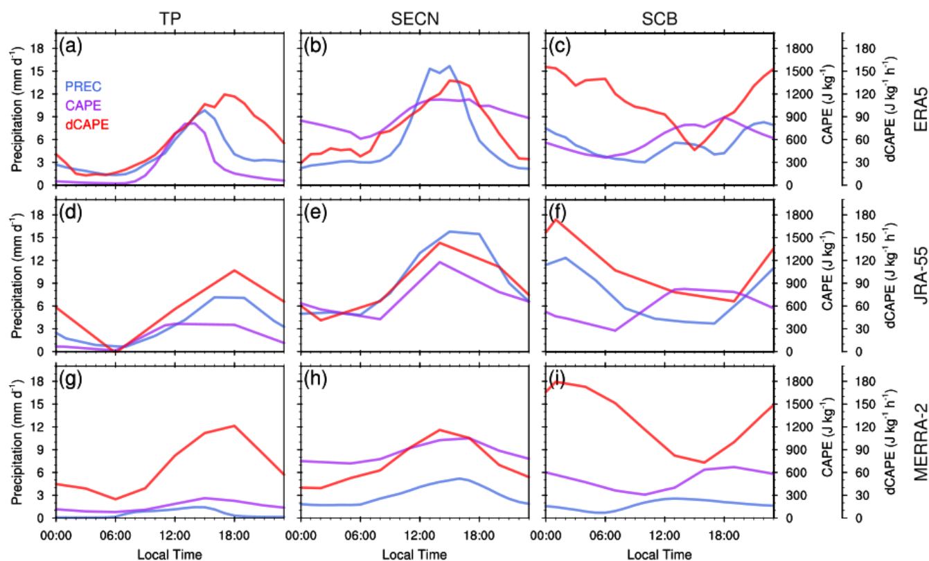
Figure 12. Diurnal variations of convective precipitation, CAPE and dCAPE over TP (left), SECN (middle) and SCB (right) from ERA5 (top), JRA-55 (middle) and MERRA-2 (bottom).
