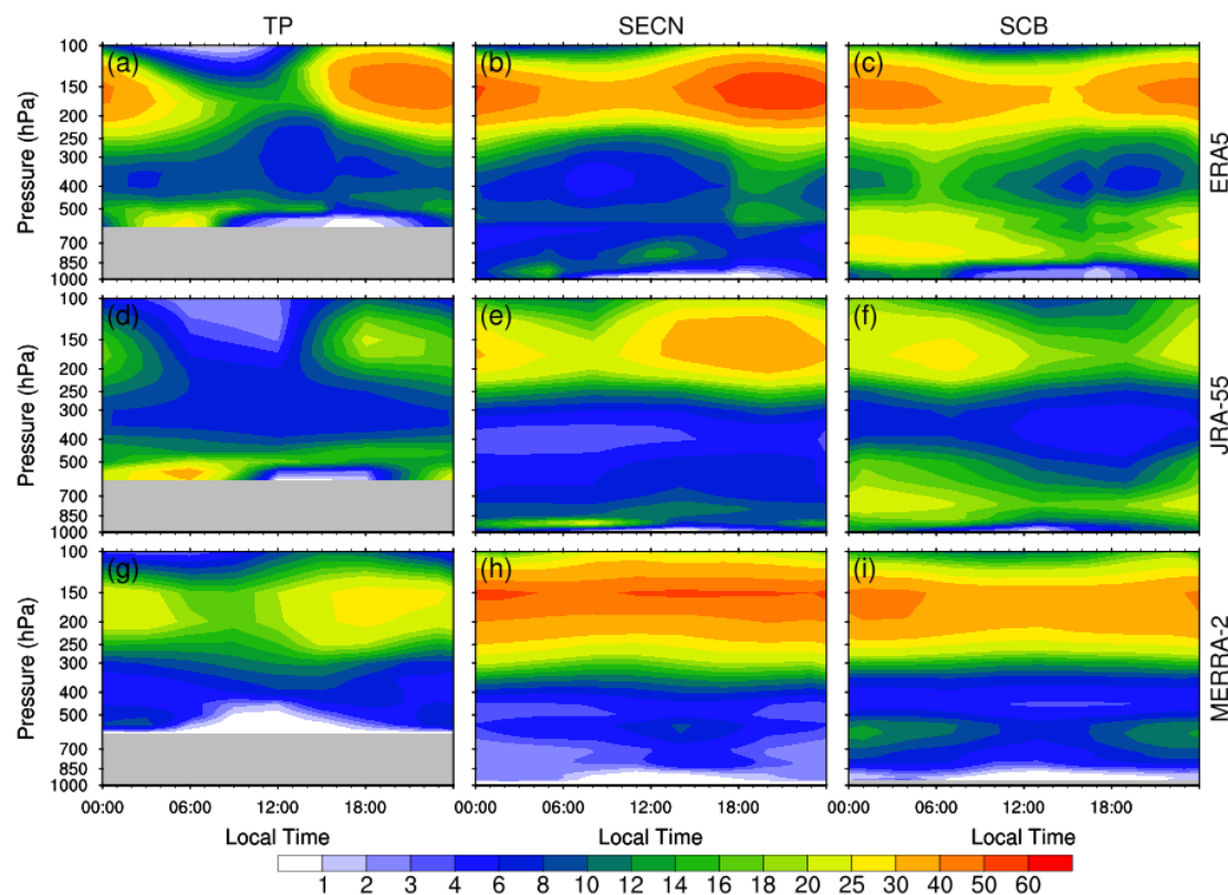
290 Figure 9. Diurnal variation of cloud fraction over TP (left), SECN (middle) and SCB (right) from ERA5 (top), JRA-55 (middle) and MERRA-2 (bottom). Units: %.
