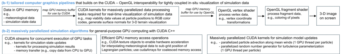
Figure 2: Conceptual summary of heterogeneous CPU-GPU implementation. (a) key elements on CPU, including tailored multi-threading for efficiency; (b) key elements on GPU, including tailored computer graphics pipelines and massively parallelized simulation algorithms.
