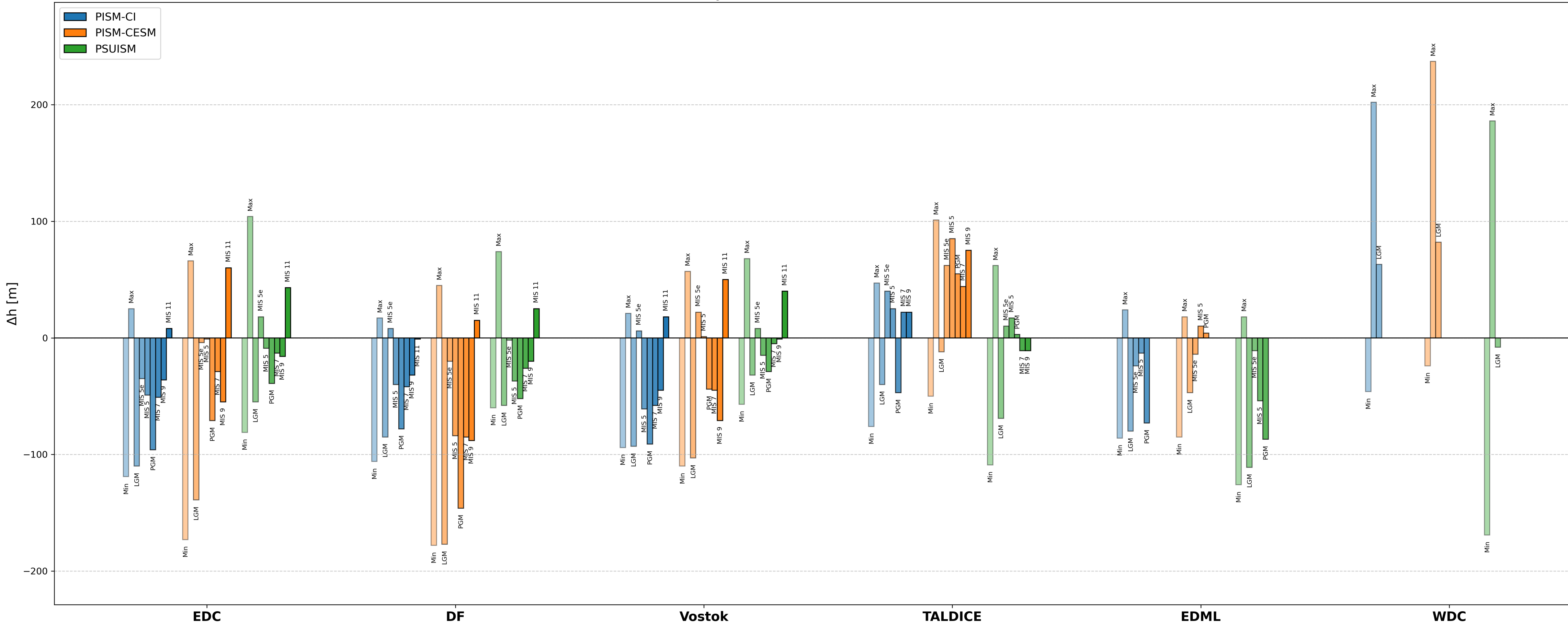
\Delta h anomalies by Ice Core Site and ISM (Min to MIS 11)
