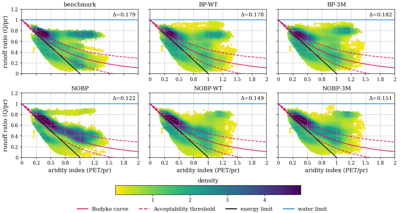
Figure 7. Density plot of aridity index vs runoff/P. The blue line represent the water limit, where runoff < precipitation, the green-black line is the energy limit, derived from the relation PET \geq AET , hence runoff/Pr \geq 1 - PET/Pr . On the top right corner of each plot the average distance (adimensional) of each pixel from the Budyko curve is indicated.
