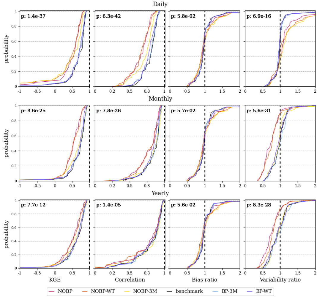
Figure 3. Empirical cumulative distribution functions (CDFs) of KGE and its three components (correlation, bias and variability ratio) across all the 60 calibrated sub-catchments for the six alternative -LISFLOOD setups (including the benchmark), evaluated at daily (top row), monthly (middle) and yearly (bottom) time scale. In the top left corner of each plot, the minimum p-value for all pairs of the Friedman test (FT) is shown: p > 0.05 indicates no significant differences among the six LISFLOOD setups, while p < 0.05 indicates significant differences.
