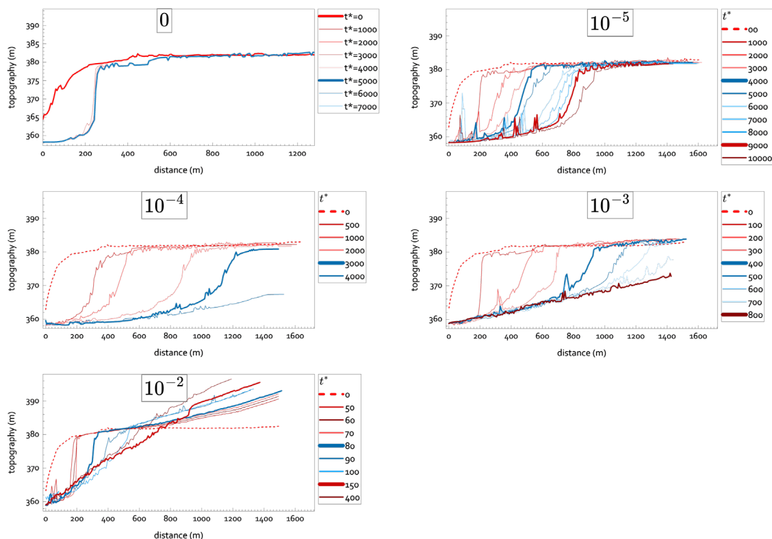
375 Figure 9: Temporal evolution of river long profile in simulation with varying sediment concentration. Canyon profile at different times for the simulation shown in Figure 8.
