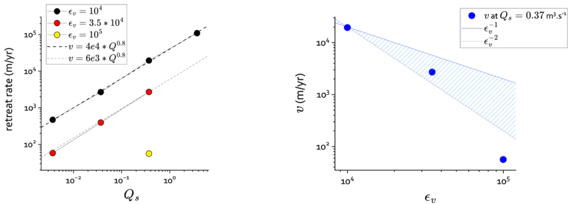
Figure 12. Left: Evaluation of the knickpoint retreat rates in m/y as a function of the inlet sediment flux for the three values of the abrasion parameter \epsilon_v . The symbols are indicated in the graph legend. The thick and thin dashed line are the fits v(Q_s) for \epsilon_v = 10^4 and 3.5 \cdot 10^4 Pa. Right: evolution of v with the abrasion parameter \epsilon_v at Q_s = 0.37 \text{ m}^3 \cdot \text{s}^{-1} . The blue lines indicate a dependency on \epsilon_v^{-1} (solid line) and \epsilon_v^{-2} (dashed line).
