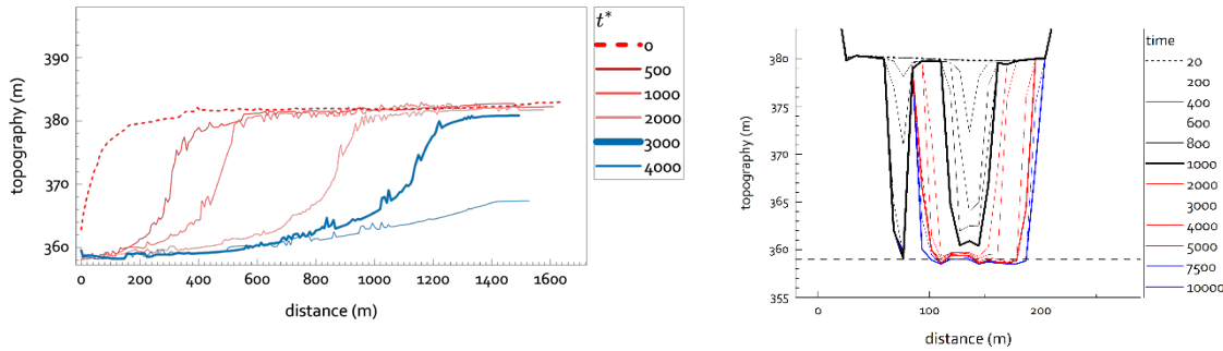
Figure 7: Temporal evolution of river profile in baseline model simulation. Left. Canyon profile at different times for the simulation shown in Figure 6. The profile is calculated for one simulation stage, so it may not be exactly on the river path everywhere at all times. Right. Canyon width at different times in the section indicated by the yellow line on the first plan view of Figure 6. The dashed line is the altitude of the base of the Schaffhausen fall.
