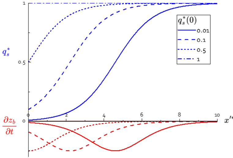
Figure 1. Plot of q_s^* = q_s/q_s^\infty (in blue) and \frac{\partial z_b}{\partial t} (in red) as a function of the dimensionless distance x'^* = \alpha x/\xi for different values of the initial conditions q_s^*(0) as indicated in the legend box.
