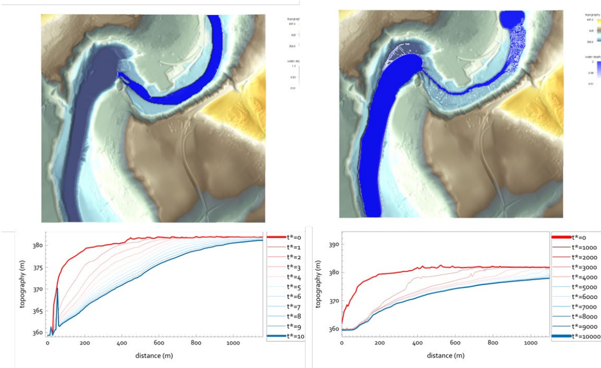
Figure 5: Simulations with a basement equation similar to the sediment equation and an input sediment concentration of 10^{-3} . The blue color indicates water depth. Left: Erodibility for the basement is the same as for the sediment. Right: erodibility is 1,000 times lower than in the left case.
