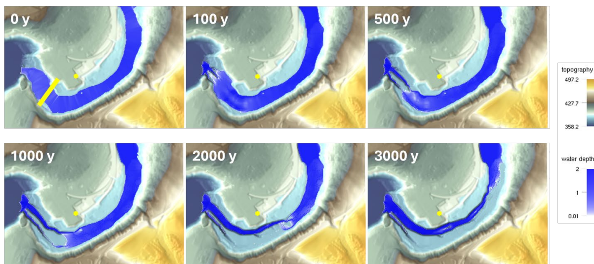
Figure 6. Simulations of the baseline model. Plan views of a simulation at 6 different times for the baseline model with \epsilon_v = 10^4 Pa and c_s^{in} = 10^{-4} with same color scales as in Figure 5.
