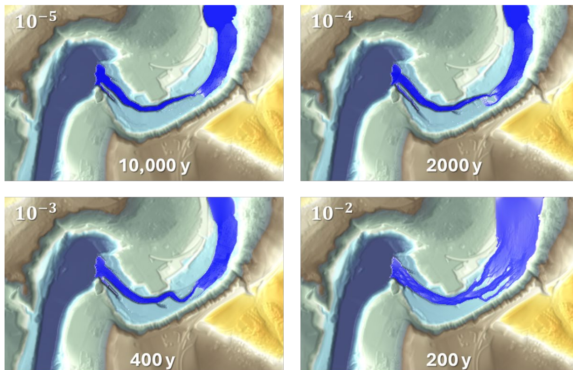
Figure 8: Simulation results varying sediment concentration. Plan view of 4 runs with \epsilon_v = 10^{-4} and input sediment concentrations of 10^{-5} at 10,000 y (top left), 10^{-4} at 2,000 y (top right), 10^{-3} at 400 y (bottom left), and 10^{-2} at 200 y (bottom right). same color scales as in Figure 6.
