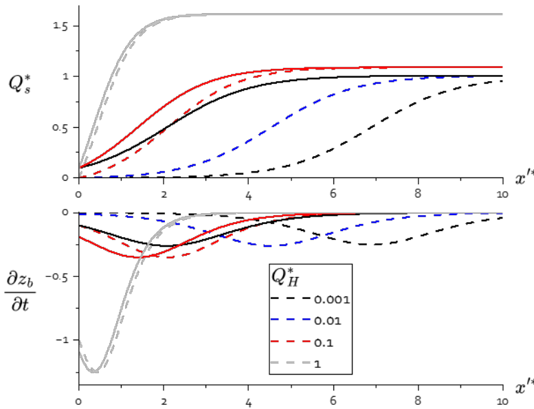
Figure 3. Top: Plot of q_s^* = q_s/q_s^\infty as a function of the dimensionless distance x'^* = \alpha x/\xi for different values of the hillslope supply parameter Q_H^* (colors as indicated in the legend box) and Q_s^*(0) . The dashed lines are plotted for Q_s^*(0)=0 ; the solid lines are plotted for Q_s^*(0) = 0.1 . Bottom: plot of the bedrock erosion rate as a function of x'^* . The legends are the same as for the top graph.
