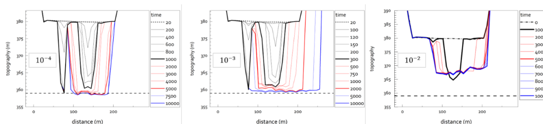
Figure 10 Temporal evolution of river cross section in simulation with varying sediment concentration. Evolution of the canyon section shown by the yellow line in Figure 6 for 3 runs corresponding to inlet sediment concentration of 10^{-4} , 10^{-3} , and 10^{-2} .
