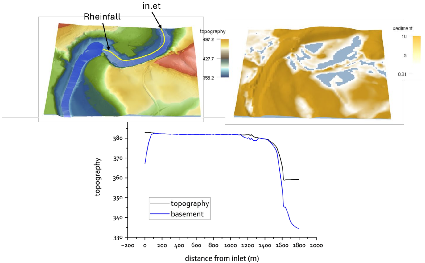
Figure 5 Top row, topography (left) and sediment (right) maps of the studied area. The units are meters. Bottom row, topography and bedrock profiles from inlet to the bottom of the Rheinfall knickpoint (yellow line in top row left).
