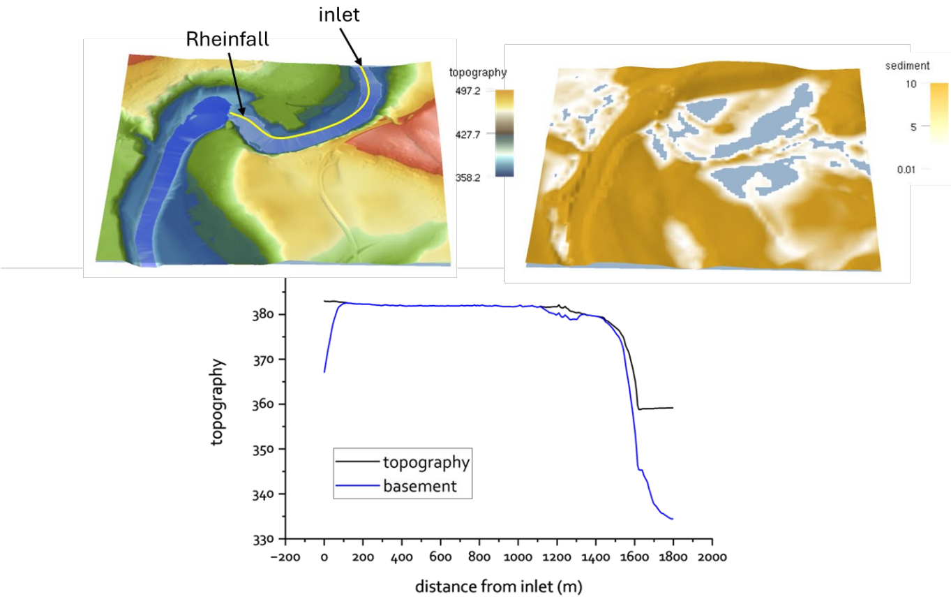
Figure 5 Top row, topography (left) and sediment (right) maps of the studied area. Bottom row, topography and bedrock profiles from inlet to the bottom of the Rheinfall knickpoint (yellow line in top row left).
