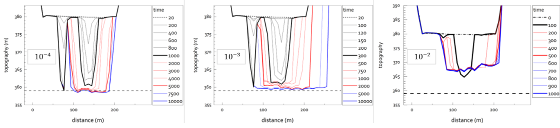
Figure 11: Temporal evolution of river cross section in simulation with varying sediment concentration. Evolution of the canyon section shown by the yellow line in Figure 7 for 3 runs corresponding to inlet sediment concentration of 10^{-4} , 10^{-3} , and 10^{-2} .
