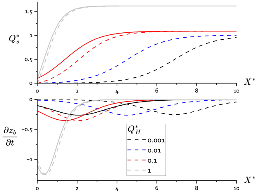
240 Figure 4. Top: Plot of q_s^* = q_s/q_s^\infty as a function of the dimensionless distance x'^* = \alpha x/\xi for different values of the hillslope supply parameter Q_H^* (colours as indicated in the legend box) and Q_s^*(0) . The dashed lines are plotted for Q_s^*(0)=0 ; the solid lines are plotted for Q_s^*(0) = 0.1 . Bottom: plot of the bedrock erosion rate as a function of x'^* . The legends are the same as for the top graph.
