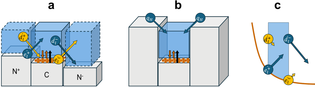
Figure 3. a. Sketch showing the vertical and lateral fluxes in the vicinity of a cell C and the different compartments they link. e_l and d_l indicates the lateral erosion and deposition, respectively. The subscript + ( - , resp.), indicates the fluxes from cells N^+ ( N^- , resp.) with higher (lower, resp.) topography. The processes with the blue arrows ( e_l^+ and d_l^- ) are controlled by the flow properties of C , specifically shear stress and bedload, and affect the bedload and topography of the adjacent cells N^+ or N^- . Conversely, the lateral fluxes indicated by yellow arrows are controlled by the flow properties of the adjacent cells and affect C . b. The case of a river supplied with sediment from lateral hillslopes (see text). c. The case where the main lateral fluxes are e_l^+ and d_l^- , i.e. those controlled by the flow characteristics of the cell.
