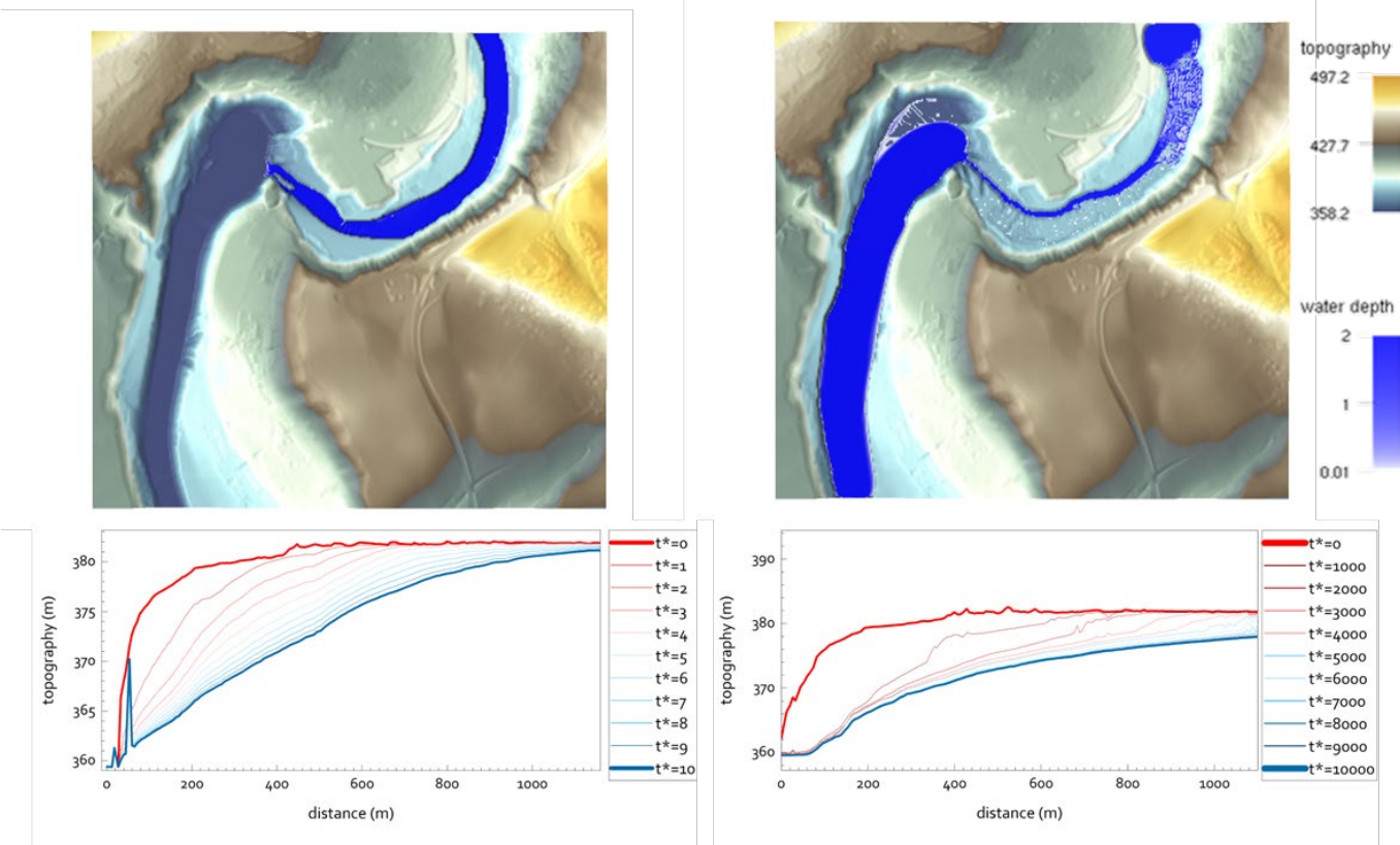
Figure 6: Simulations with a basement equation similar to the sediment equation and an input sediment concentration of 10^{-3} . The blue colour indicates water depth. Left: Erodibility for the basement is the same as for the sediment. Right: erodibility is 1,000 times lower than in the left case.
