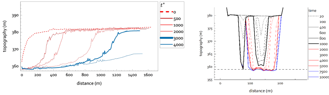
Figure 8: Temporal evolution of river profile in baseline model simulation. Left. Canyon profile at different times for the simulation shown in Figure 7. Right. Canyon width at different times in the section indicated by the yellow line on the first plan view of Figure 7. The dashed line is the altitude of the base of the Schaffhausen fall.
