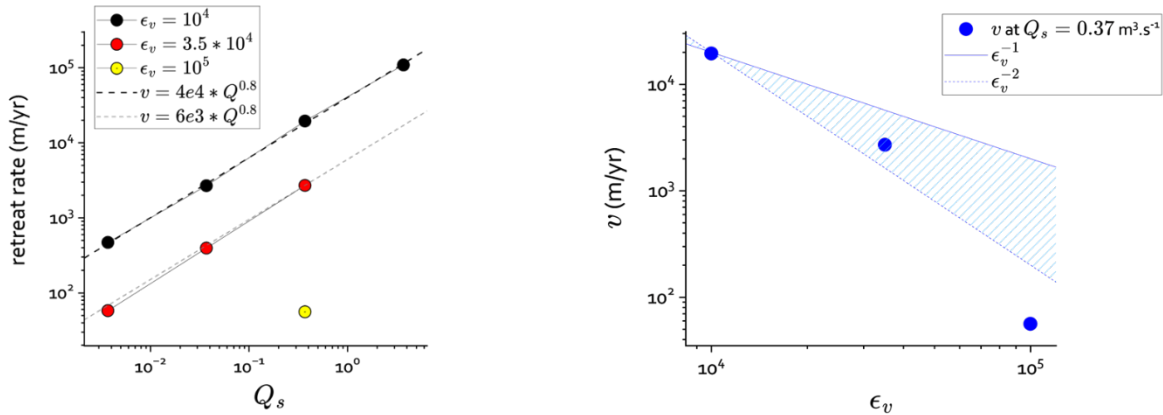
Figure 13. Left: Knickpoint retreat rates in m/y as a function of the inlet sediment flux for the three values of the abrasion parameter \epsilon_v . The symbols are indicated in the graph legend. The thick and thin dashed line are the fits v(Q_s) for \epsilon_v = 10^4 and 3.5 \cdot 10^4 Pa. Right: evolution of v with the abrasion parameter \epsilon_v at Q_s = 0.37 m 3 ·s -1 . The blue lines indicate a dependency on \epsilon_v^{-1} (solid line) and \epsilon_v^{-2} (dashed line).
