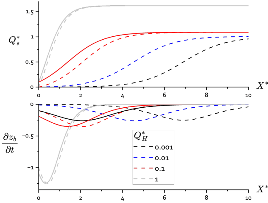
Figure 4. Top: Plot of q_s^* = q_s/q_s^\infty as a function of the dimensionless distance x'^* = \alpha x/\xi for different values of the hillslope supply parameter Q_H^* (colours as indicated in the legend box) and Q_s^*(0) . The dashed lines are plotted for Q_s^*(0)=0 ; the solid lines are plotted for Q_s^*(0) = 0.1 . Bottom: plot of the bedrock erosion rate as a function of x'^* . The legends are the same as for the top graph.
