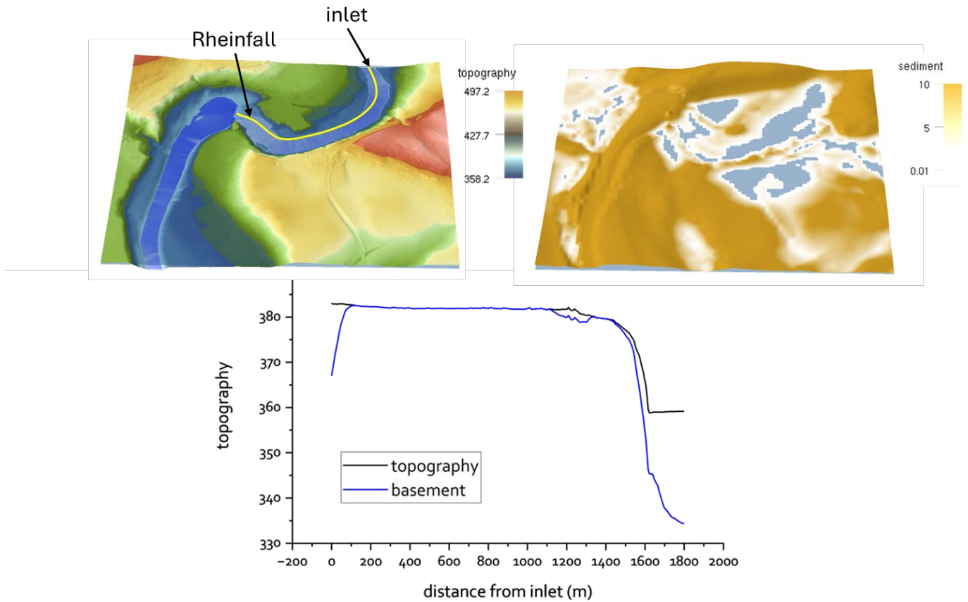
Figure 5 Top row, topography (left) and sediment (right) maps of the studied area. The units are meters. Bottom row, topography and bedrock profiles from inlet to the bottom of the Rheinfall knickpoint (yellow line in top row left).
