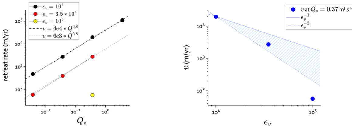
445 Figure 13. Left: Knickpoint retreat rates in m/y as a function of the inlet sediment flux for the three values of the abrasion parameter \epsilon_v . The symbols are indicated in the graph legend. The thick and thin dashed line are the fits v(Q_s) for \epsilon_v = 10^4 and 3.5 \cdot 10^4 Pa. Right: evolution of v with the abrasion parameter \epsilon_v at Q_s = 0.37 m 3 .s -1 . The blue lines indicate a dependency on \epsilon_v^{-1} (solid line) and \epsilon_v^{-2} (dashed line).
