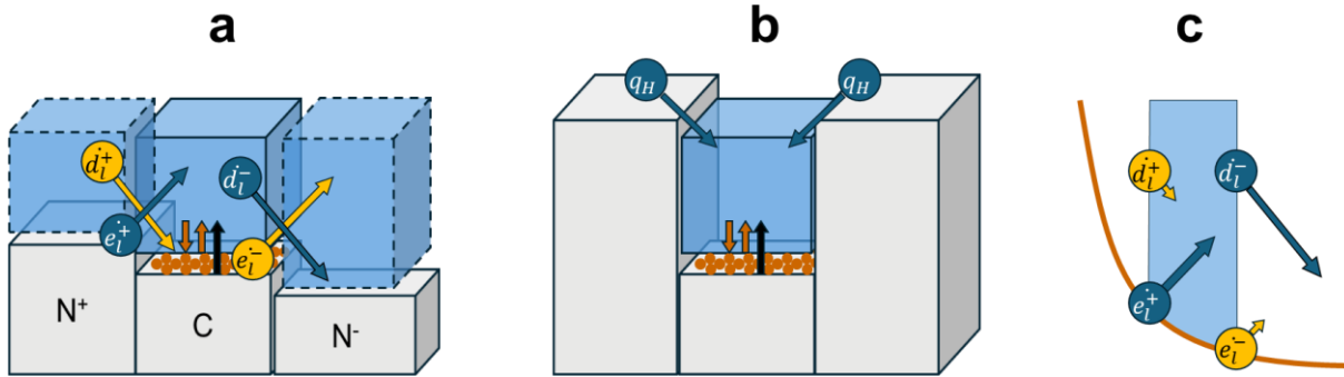
Figure 3332. a. Sketch showing the vertical and lateral fluxes in the vicinity of a cell C and the different compartments they link. e_l and d_l indicates the lateral erosion and deposition, respectively. The subscript + ( - , resp.), indicates the fluxes from cells N^+ ( N^- , resp.) with higher (lower, resp.) topography. The processes with the blue arrows ( e_l^+ and d_l^- ) are controlled by the flow properties of C , specifically shear stress and bedload, and affect the bedload and topography of the adjacent cells N^+ or N^- . Conversely, the lateral fluxes indicated by yellow arrows are controlled by the flow properties of the adjacent cells and affect C . b. The case of a river supplied with sediment from lateral hillslopes (see text). c. The case where the main lateral fluxes are e_l^+ and d_l^- , i.e. those controlled by the flow characteristics of the cell.
