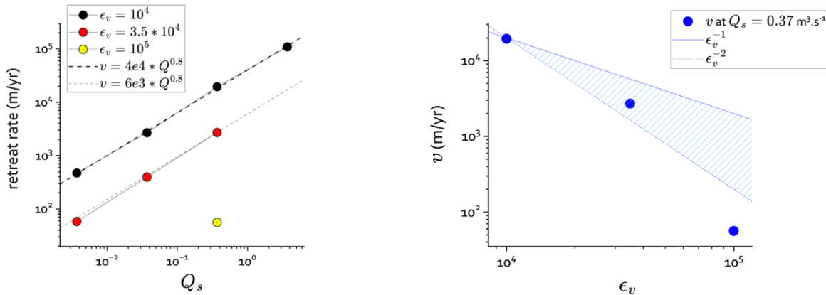
Figure 13. Left: Evaluation of the knickpoint retreat rates in m/y as a function of the inlet sediment flux for the three values of the abrasion parameter \epsilon_v . The symbols are indicated in the graph legend. The thick and thin dashed line are the fits v(Q_s) for \epsilon_v = 10^4 and 3.5 \cdot 10^4 Pa. Right: evolution of v with the abrasion parameter \epsilon_v at Q_s = 0.37 \text{ m}^3 \cdot \text{s}^{-1} . The blue lines indicate a dependency on \epsilon_v^{-1} (solid line) and \epsilon_v^{-2} (dashed line).
