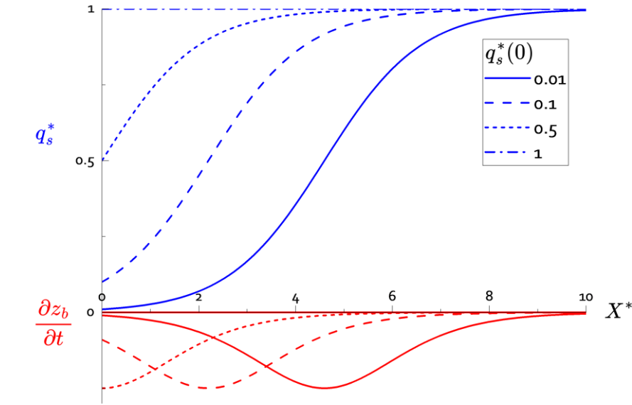
Figure 2221. Plot of q_s^* = q_s/q_s^\infty (in blue) and \frac{\partial z_b}{\partial t} (in red) as a function of the dimensionless distance x^{f*} = \alpha x/\xi for different values of the initial conditions q_s^*(0) as indicated in the legend box.
