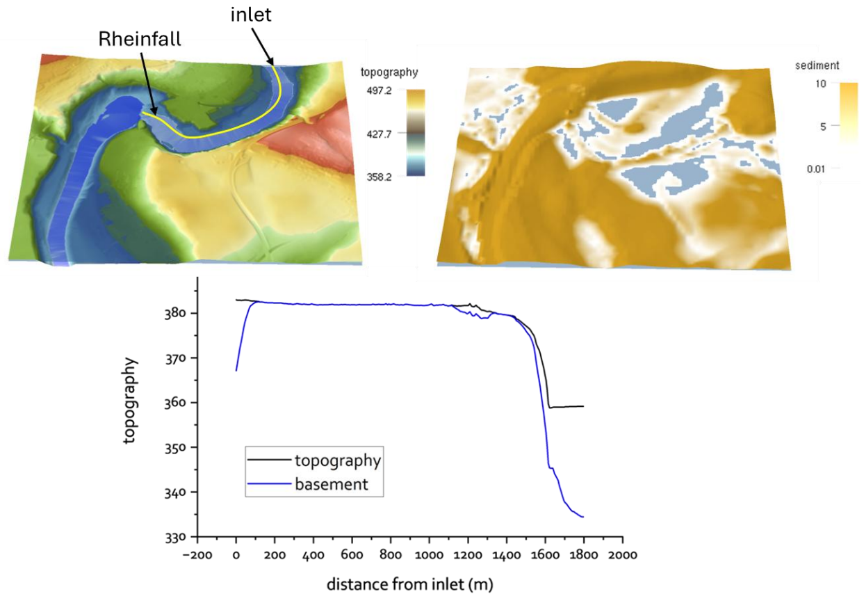
Figure 554 Top row, topography (left) and sediment (right) maps of the studied area. Bottom row, topography and bedrock profiles from inlet to the bottom of the Rheinfall knickpoint (yellow line in top row left).
