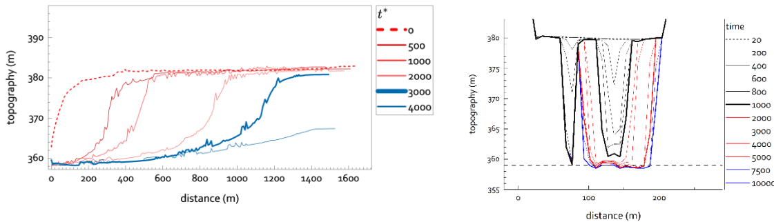
Figure 8887: Temporal evolution of river profile in baseline model simulation. Left. Canyon profile at different times for the simulation shown in Figure 7Figure 7Figure 6Figure 6. The profile is calculated for one simulation stage, so it may not be exactly on the river path everywhere at all times. Right. Canyon width at different times in the section indicated by the yellow line on the first plan view of Figure 7Figure 7Figure 6Figure 6. The dashed line is the altitude of the base of the Schaffhausen fall.
