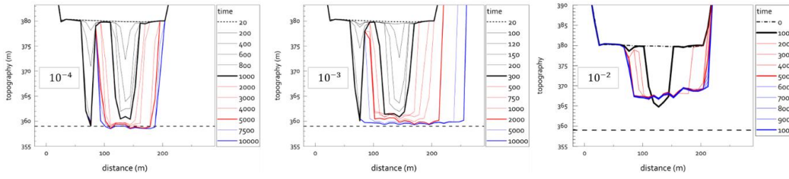
Figure 11: Temporal evolution of river cross section in simulation with varying sediment concentration. Evolution of the canyon section shown by the yellow line in Figure 7 for 3 runs corresponding to inlet sediment concentration of 10^{-4} , 10^{-3} , and 10^{-2} .
