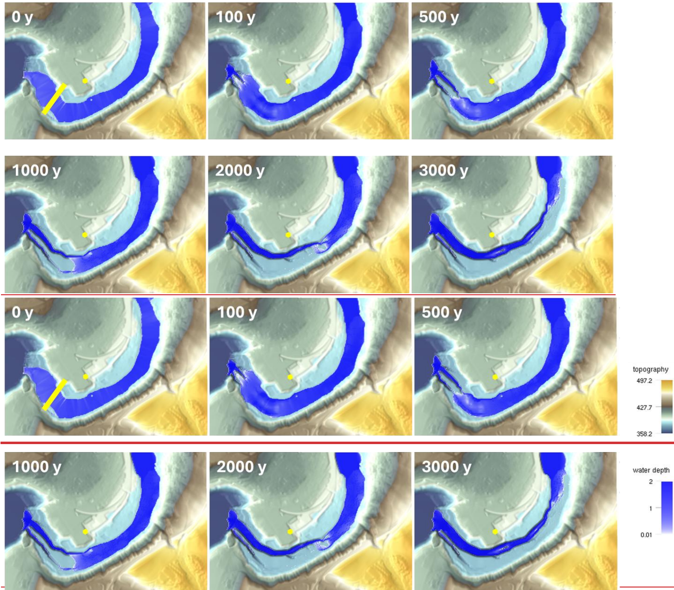
Figure 7776. Simulations of the baseline model. Plan views of a simulation at 6 different times for the baseline model with \epsilon_p = 10^4 Pa and c_s^{ln} = 10^{-4} with same color colour scales as in Figure 6 Figure 6 Figure 5.
