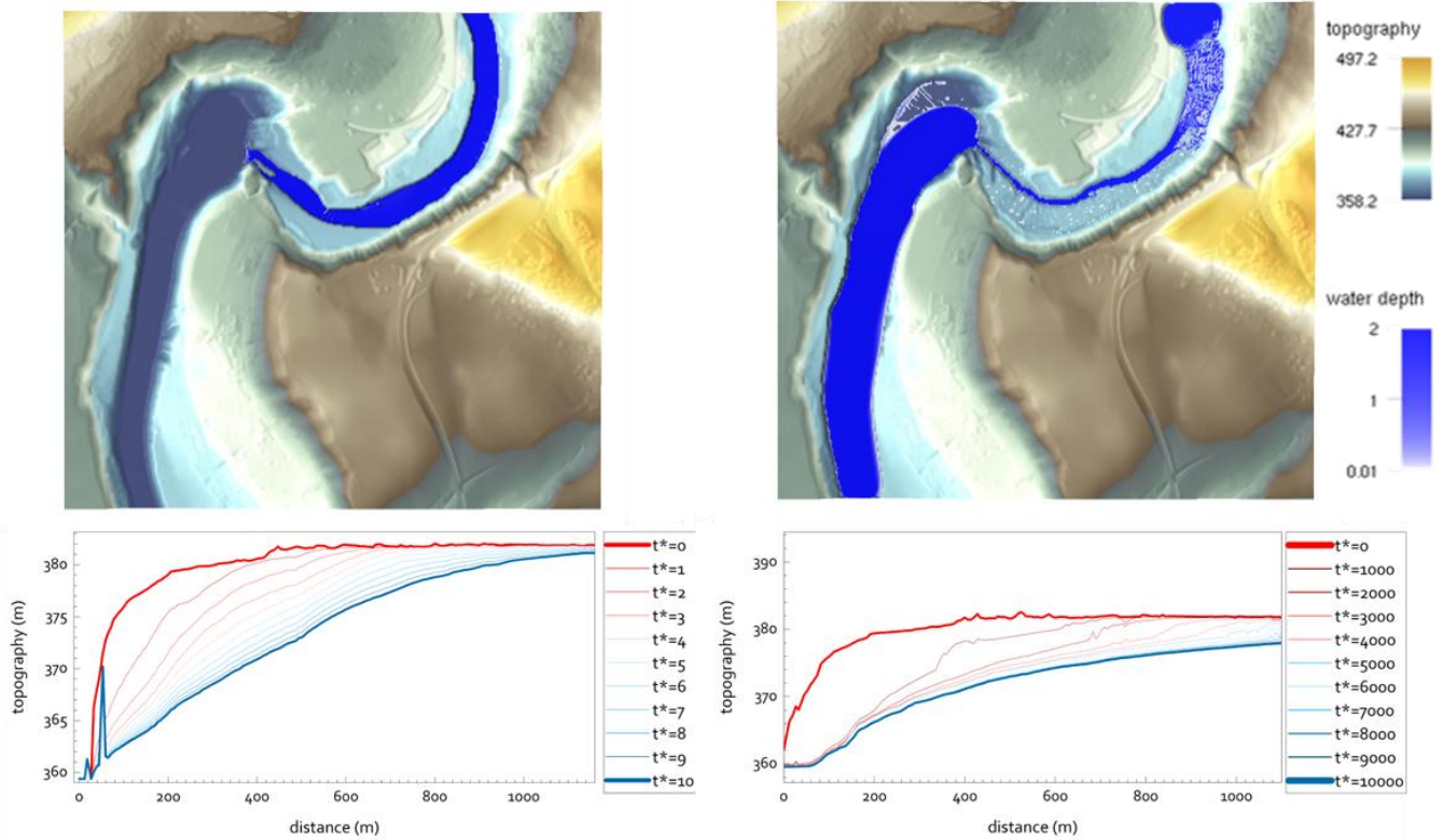
Figure 6665: Simulations with a basement equation similar to the sediment equation and an input sediment concentration of 10^{-3} . The blue color indicates water depth. Left: Erodibility for the basement is the same as for the sediment. Right: erodibility is 1,000 times lower than in the left case.
