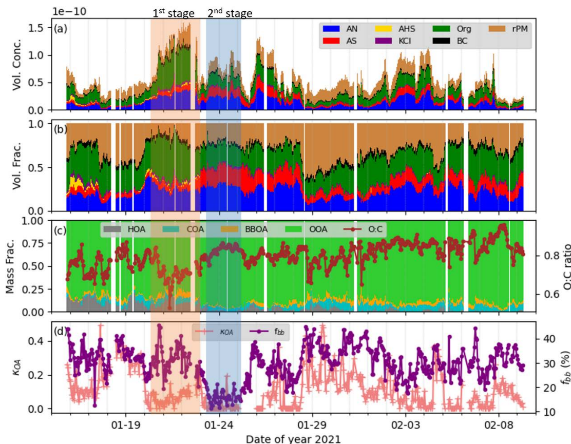
Figure 3: Time series of (a) volume concentrations (b) volume fractions of different chemical species in PM_{2.5} , (c) mass fractions of different OA factors and O:C ratio, (d) \kappa_{OA} and relative contribution of biomass burning to BC ( f_{bb} ) at the Huainan site during the winter campaign. The shaded area denotes a persistent pollution episode from 20 to 25 January 2021, with different colors indicating distinct stages of the episode.
