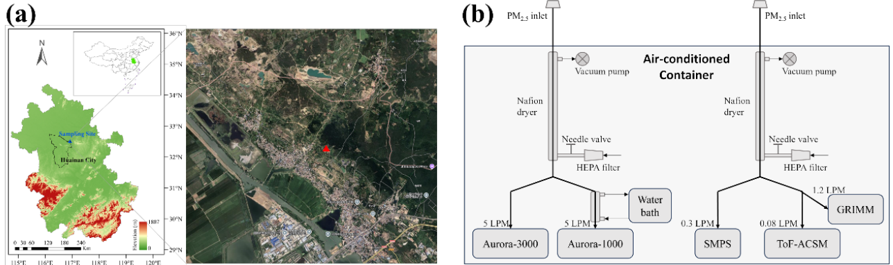
100 Figure 1: (a) The geographic location of the Huainan Climate and Environment Observatory marked by a triangle on the topographic map; (b) schematic diagram of the hygroscopicity observation system. Map data © 2025 Google.
